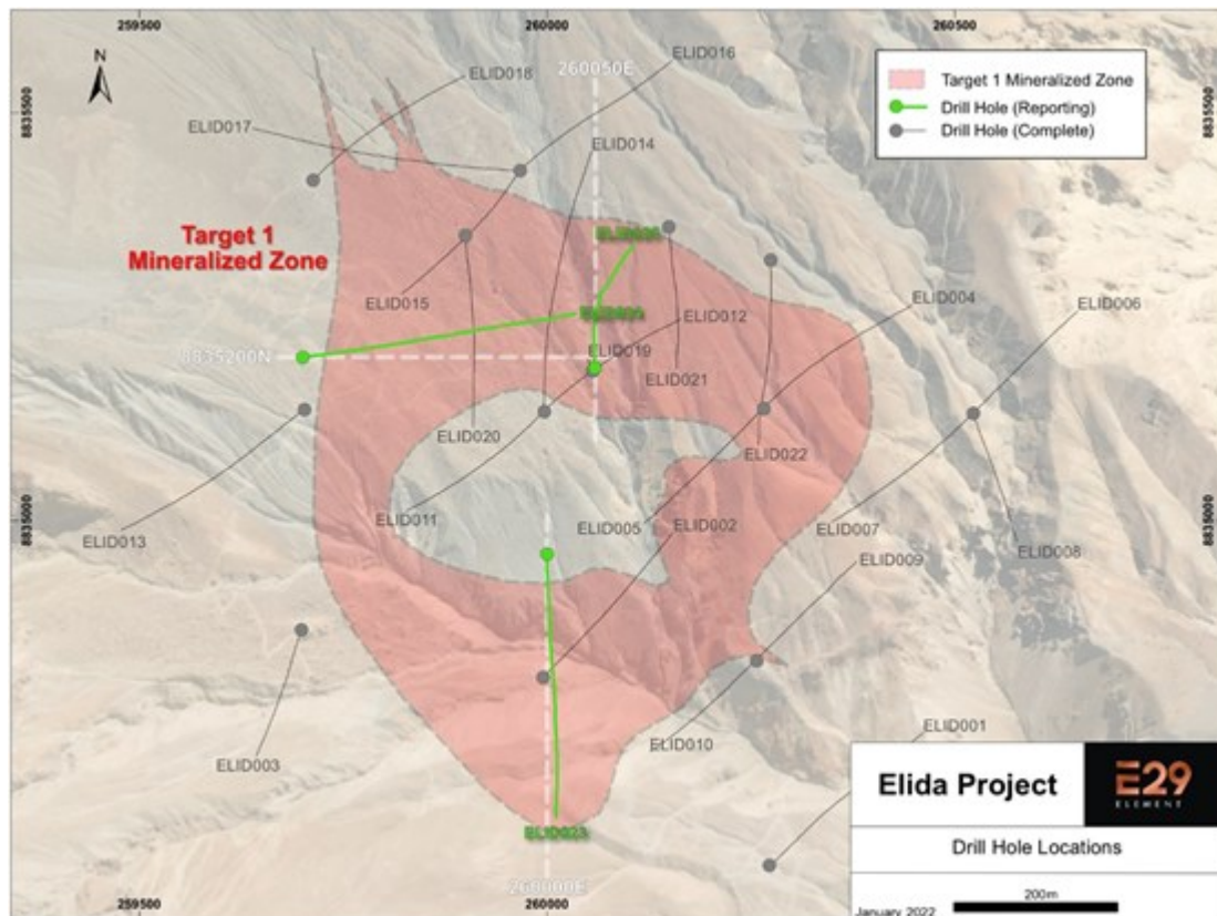
Figure 1. Plan view of Target 1 at the Elida Porphyry Cu-Mo project. The Phase 1 drilling program consisting of seven holes was completed in December 2021. The last three holes from this program are reported in this press release. Section locations for Figures 2, 3 and 4 are indicated with white dashed lines. Holes ELID001 - ELID018 were completed by Lundin Mining in 2014/15 and ELID019 - ELID025 were completed by Element 29 in 2021.
