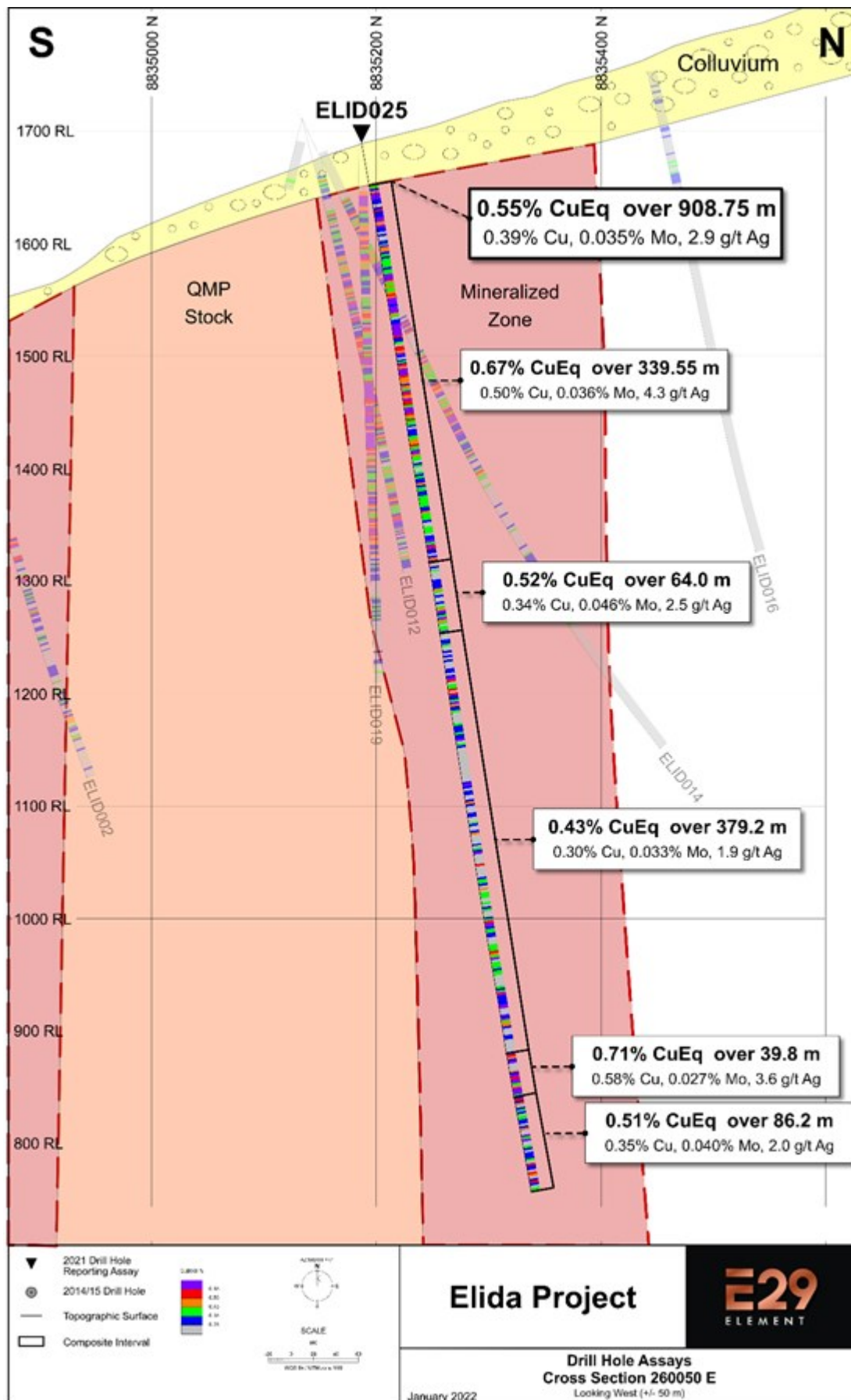
Figure 2. Cross section 260050 E showing hole ELID025 . The hole entered well-mineralized, potassic-altered sedimentary rocks immediately beneath 35 m of gravel cover. Continuous mineralization was encountered to the bottom of the hole at 947.2 m. This hole demonstrated the vertical continuity of mineralization to a depth of 933 m below surface. Apart from the zone of strong mineralization present near the top of the hole, other well mineralized intervals are distributed throughout the hole. The hole ended in mineralization and the mineralized zone remains open at depth.
