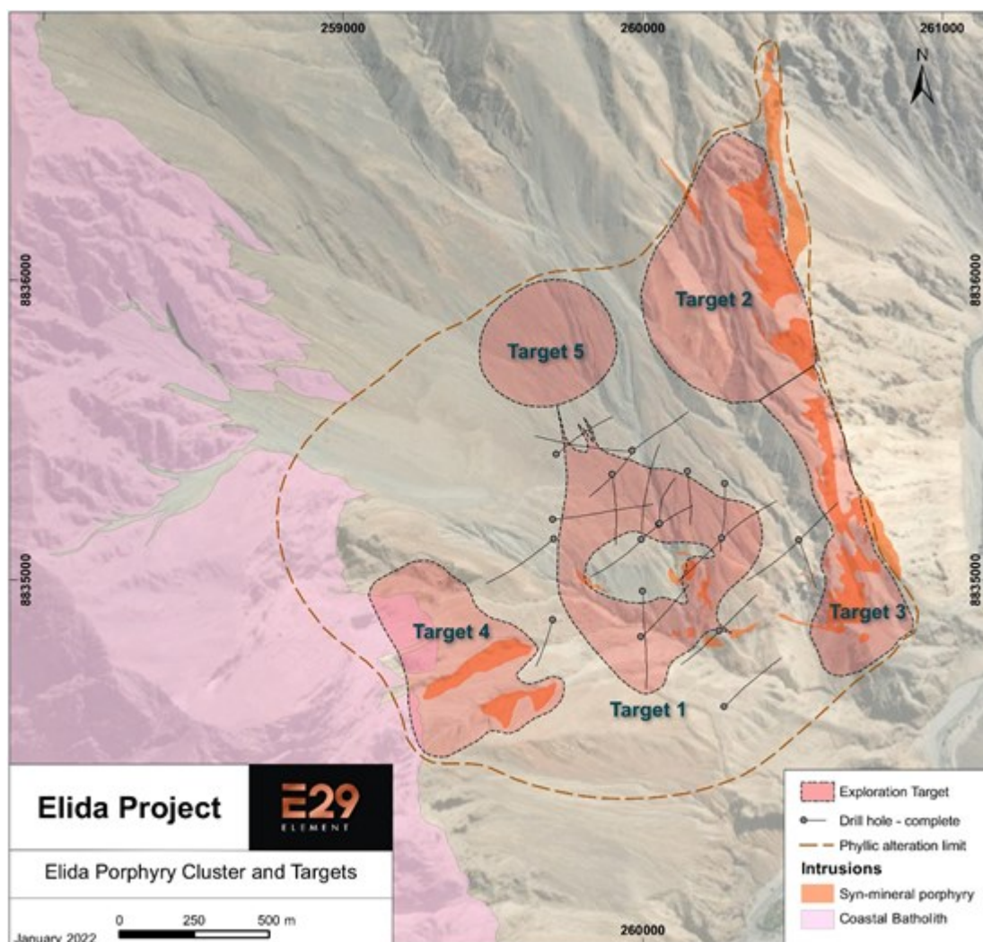
Figure 5. Plan view of the Elida exploration targets represented by five porphyry centres enclosed by a 2 x 2 km alteration system. Only Target 1 has been drill-tested. Targets 2 and 3 contain exposed leached capping associated with quartz monzonite porphyry intrusions overprinted by quartz vein stockworks. The Company plans to complete initial drilling on Targets 2 and 3 later in 2022.
