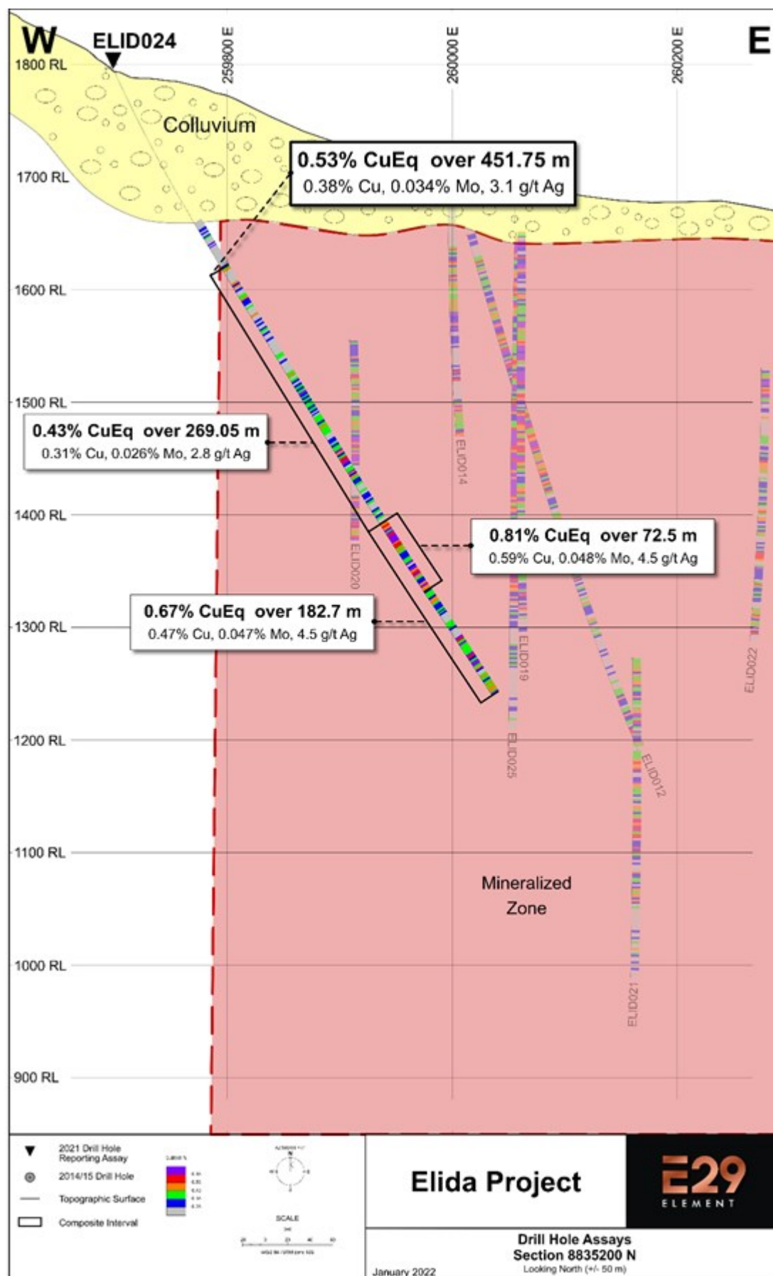
Figure 3. Cross section at 8835200 N showing the position of ELID024 . This hole was designed to constrain the western limit of Target 1 mineralized zone and test for continuity of mineralization in a
