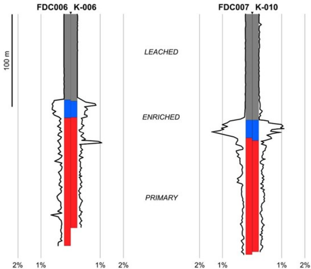
Figure 7. (a) Graphic comparison of results from FDC006 and historical hole K-006. (b) Graphic comparison of FDC007 and K-010. There were small differences in the position of the oxide and enrichment zone boundaries. The twinned hole was positioned approximately 2 m away from the historical hole.
