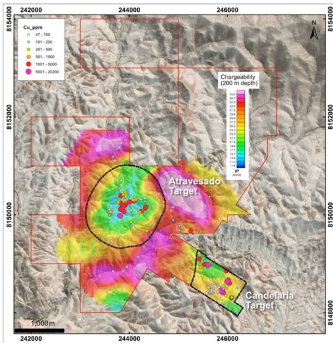
Figure 9. The Atravesado porphyry target is characterized by moderate resistivity, anomalous copper geochemistry, potassic alteration and associated quartz vein stockworks. Phyllic alteration correlates with zones of high chargeability. The Candelaria target area is located 2.0 km to the southeast.
