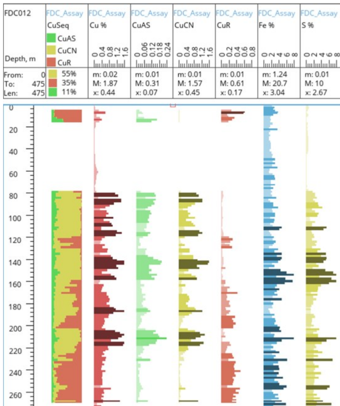
Figure 5. Profile of drill hole FDC012 showing Cu grade with the proportions of Cu given by sequential leach analysis. The abrupt contact of the enrichment zone at 79.9m is visible in the Cu% column. The enrichment zone (79.9 - 180.0 m) is dominated by CuCN, which measures soluble copper sulfide minerals such as chalcocite. A transitional zone containing mixtures of chalcocite and chalcopyrite extends to 232.0m. The remainder of the hole intersected primary sulphide (chalcopyrite) mineralization. The profile shows the portion of the hole where sequential leach analysis was undertaken. FDC012 was drilled to a depth of 475 m.
