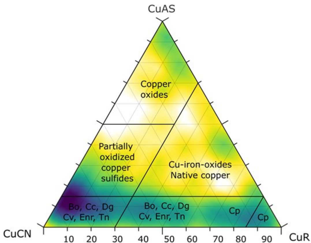
Figure 3. Ternary diagram used to display results (674 samples) from sequential leach analysis for data from Flor de Cobre. The proportions of copper reported in sulphuric acid, sodium cyanide, and four-acid
