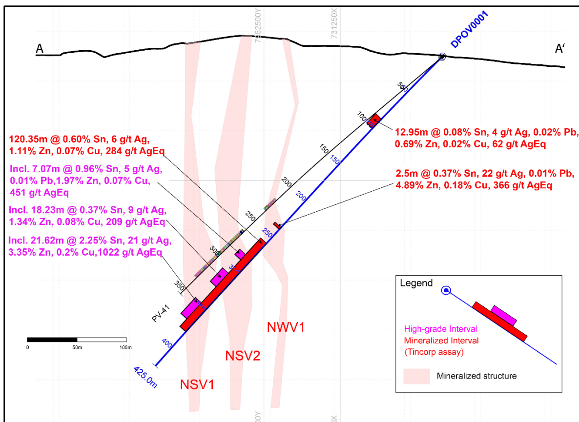
Figure 2. Cross section of drill hole DPOV0001 (Looking SSE)
