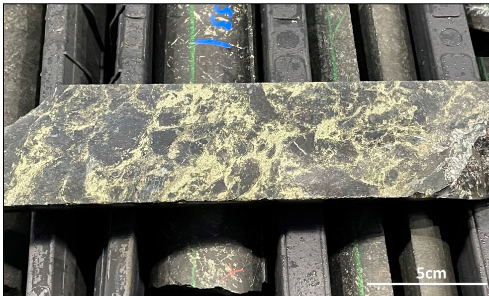
Figure 5. High-grade chalcopyrite matrix breccia in massive magnetite altered host rock, 0.5m @ 4.76% Cu and 0.48g/t Au from 354m, SDD008, South Darwin prospect.
