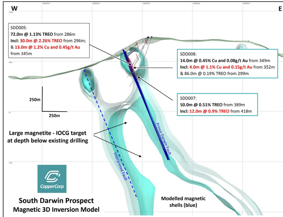
Figure 4. South Darwin prospect 3D section (looking north) showing the 3D inversion standard magnetic susceptibility model and deep target zone underlying the prospect area. Shown magnetic susceptibility isosurface shells are for 0.5 SI (inner), 0.3 SI (middle) and 0.2 SI (outer).
