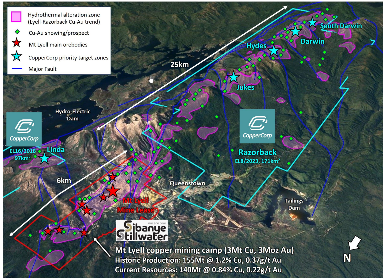
Figure 1. – Location of the Razorback property relative to the Mt Lyell copper-gold mine – Blue outlines are CopperCorp’s 100% owned licenses.
