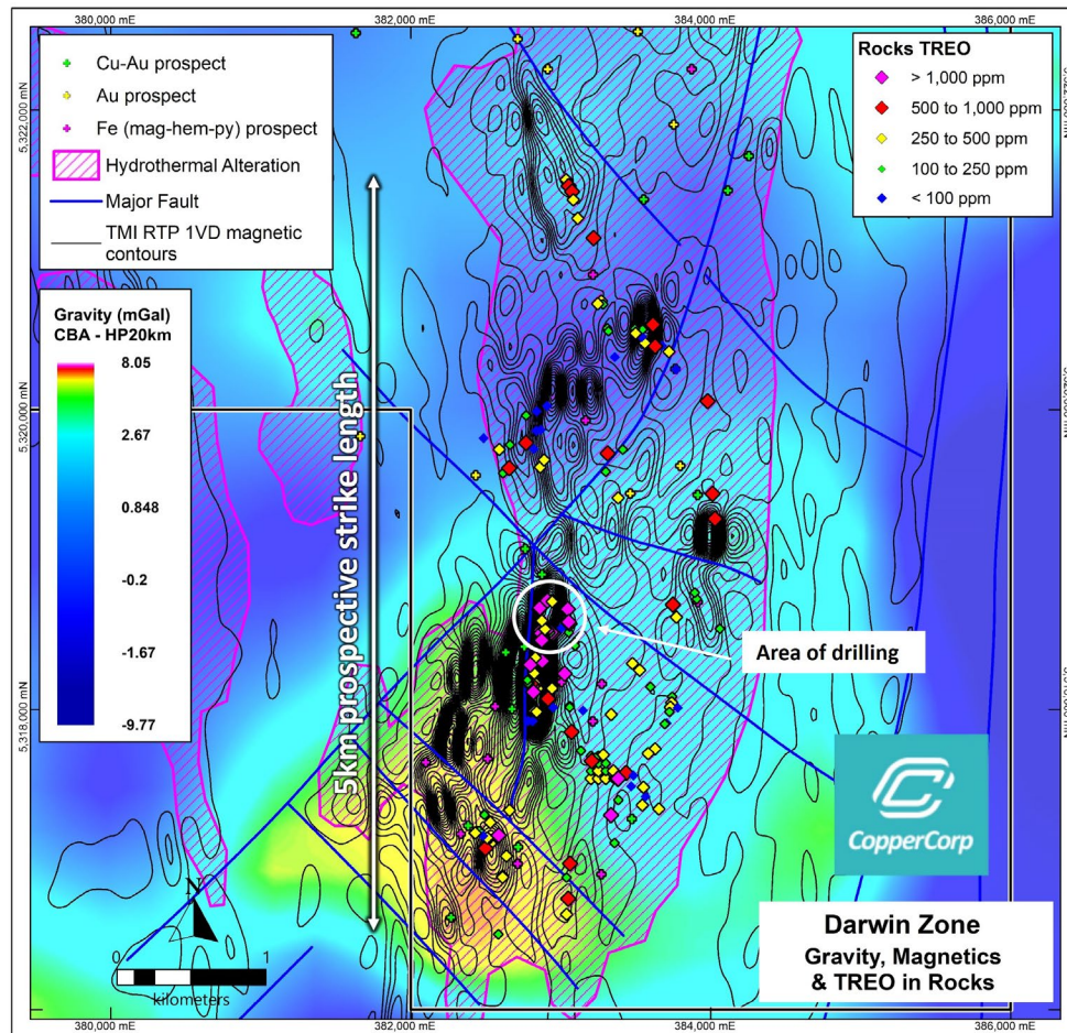
Figure 7. Darwin Zone area with complete bouguer anomaly (CBA), 20km high-pass (HP20km) residual gravity image, TMI 1VD magnetic contours, rock chip total rare earth oxide (TREO) values.
