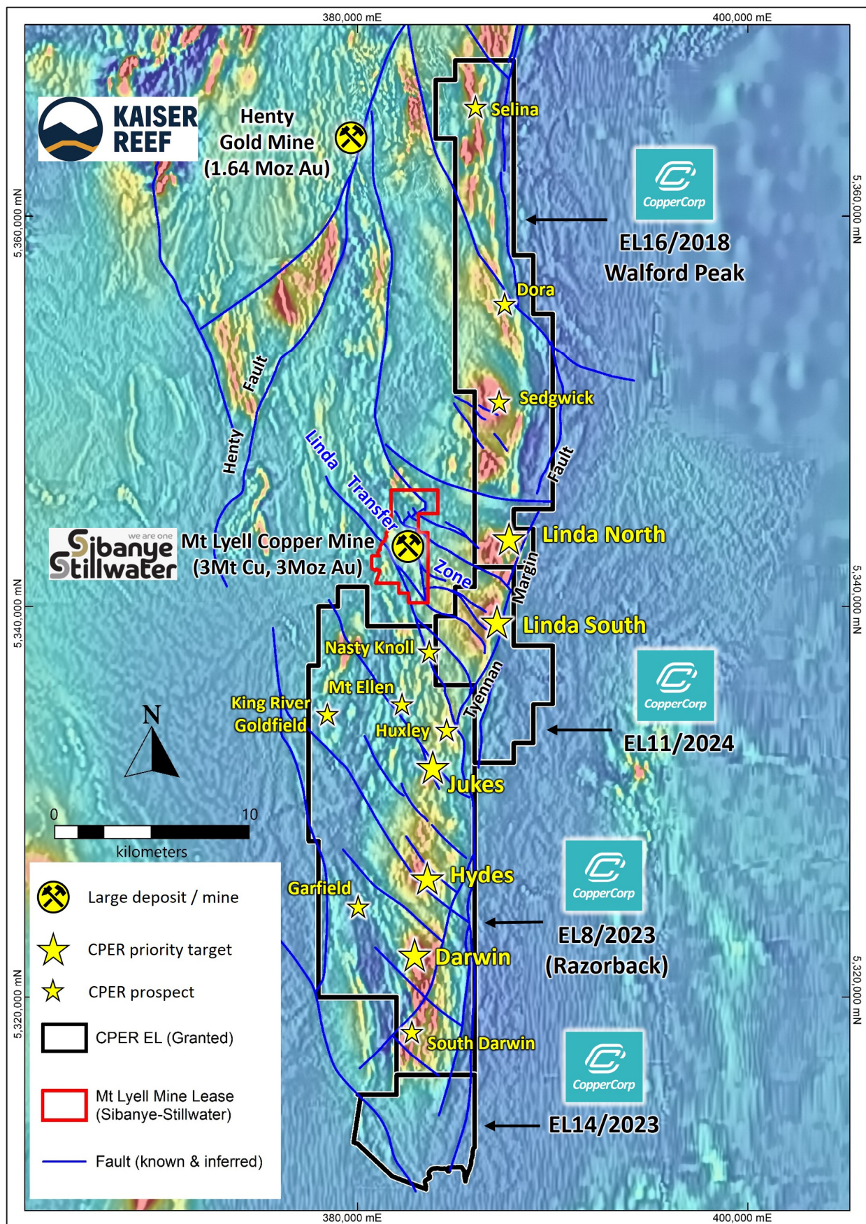
Figure 1. Southern Skyline Project properties and exploration target areas with magnetics TMI RTP image.
