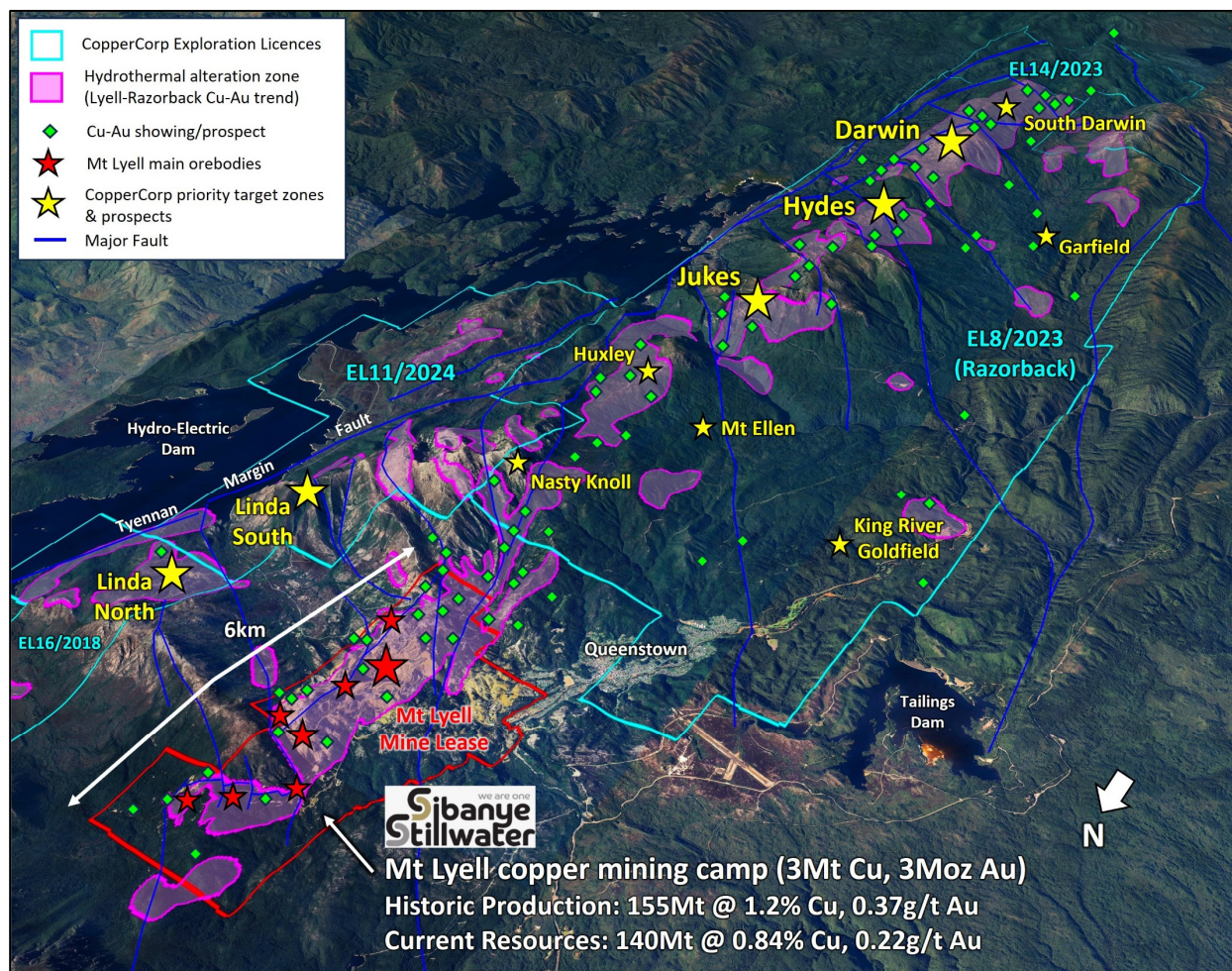
Figure 2. Location of the Razorback property and the Jukes Zone target area relative to the Mt Lyell copper-gold mine. Blue outlines are CopperCorp's 100% owned licenses.
