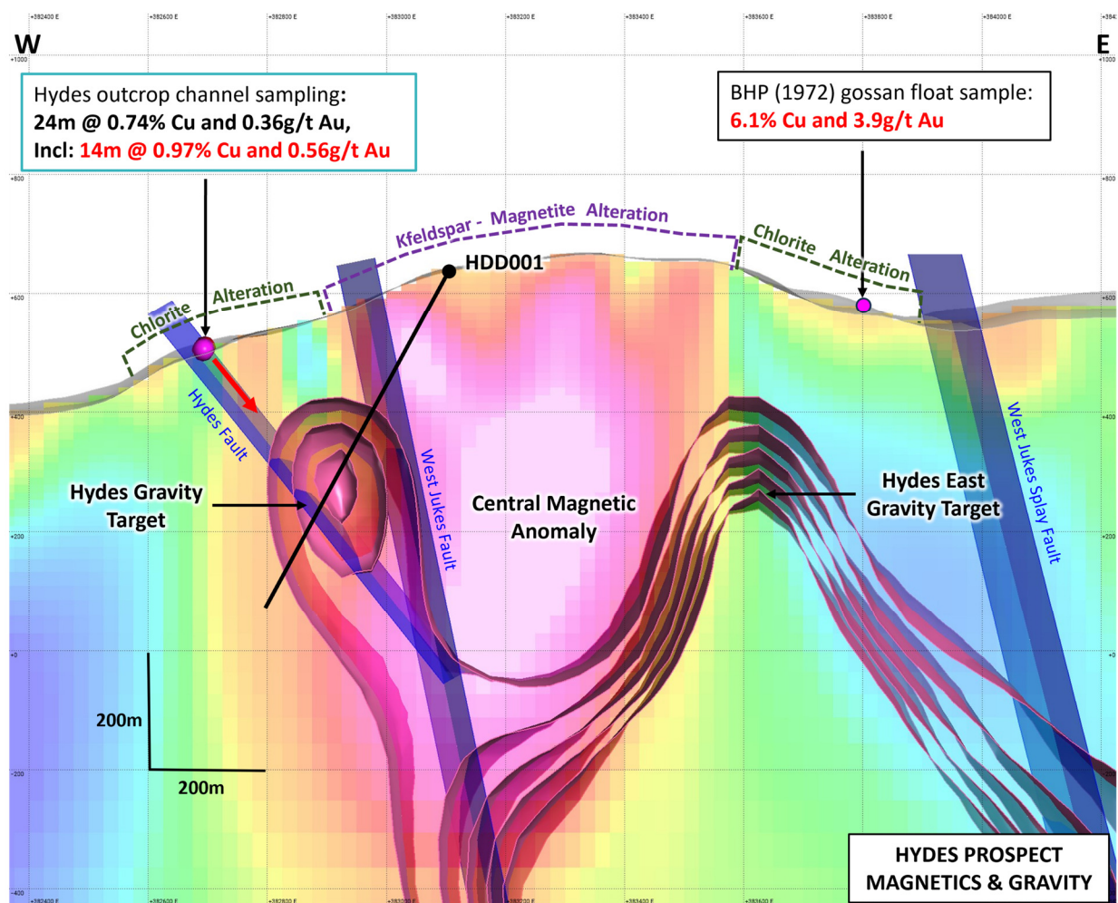
Figure 3. Hydes cross-section 5326400mN (looking north) showing revised 3D inversion models for magnetics (pseudocolour grid) and gravity/density (pink isosurface shells) and planned first drill hole trace targeting the Hydes gravity anomaly down-dip of outcropping mineralization.
