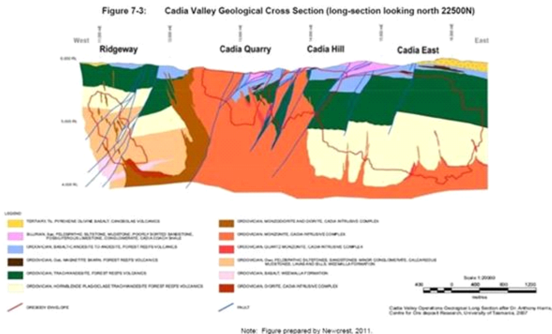
Figure 2 - West – East Geological Cross Section (looking North) of Ridgeway – Cadia deposit area. Note: the entire section is underlain by the igneous complex (Gleeson et al 2020).
