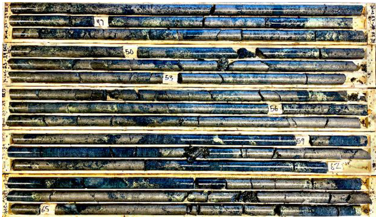
Figure 1. Diamond Drill Hole Wine 23-29 (45.2m-66.4m) Main Zone Mineralization
