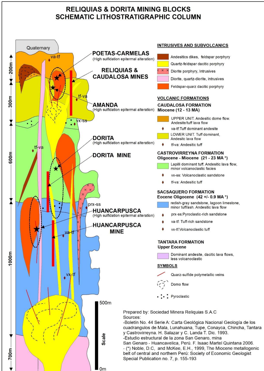
Figure 7-2: Regional Stratigraphic Column
