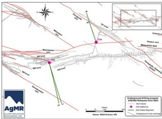
Figure 3: Location of initial four drill holes from Phase 2 of the 2023 drill program (CNW Group/Silver Mountain Resources Inc.)
