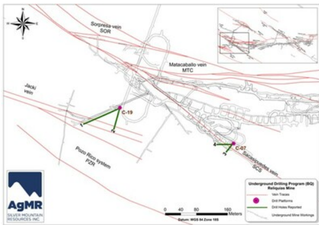
Figure 5: Location of Phase 1 Pozo Rico BQ diameter drill holes (CNW Group/Silver Mountain Resources Inc.)
