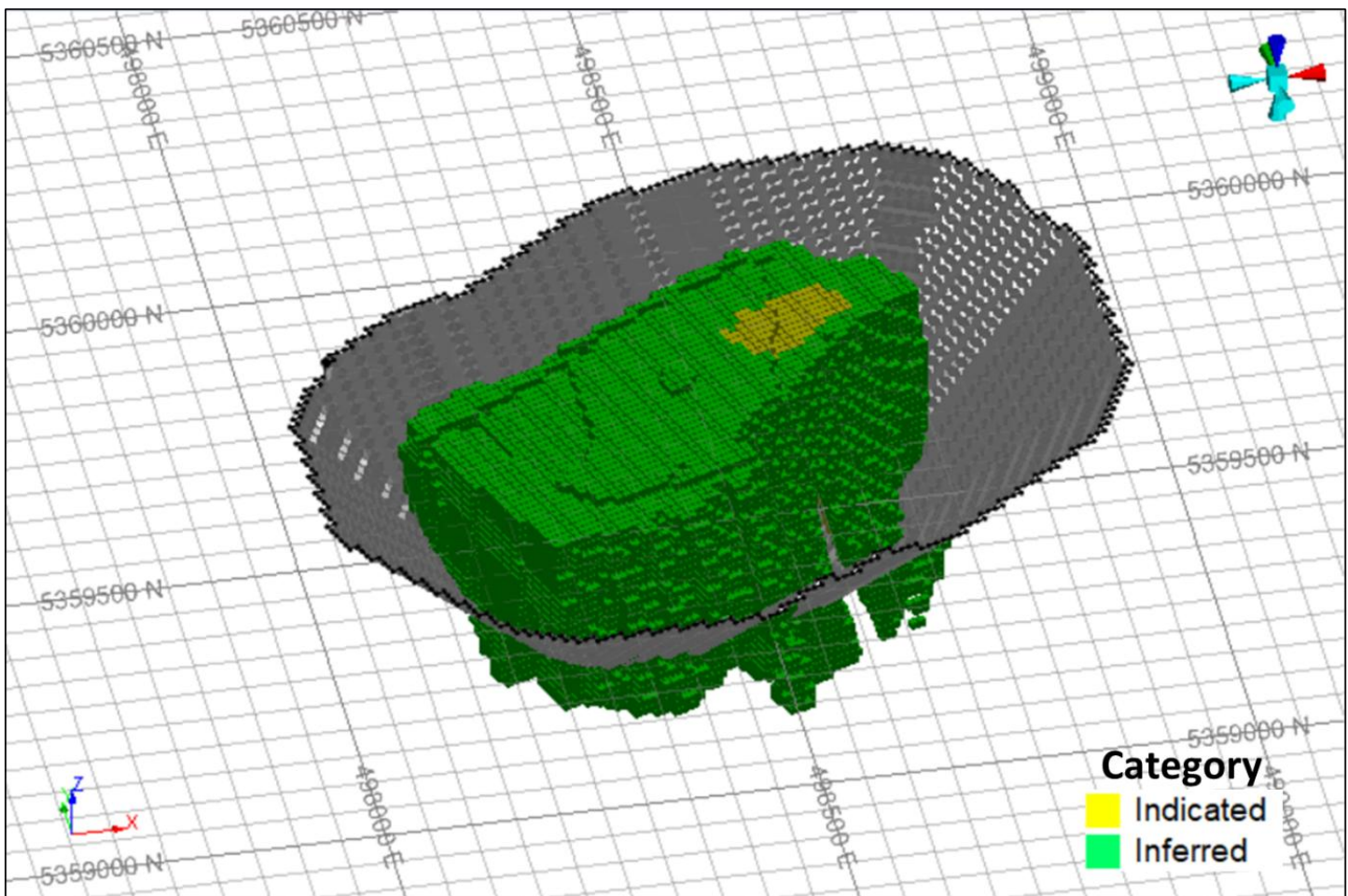
Figure 2: Isometric View Showing the pit shell (light grey) with respect to the modelled Indicated and Inferred Resources
