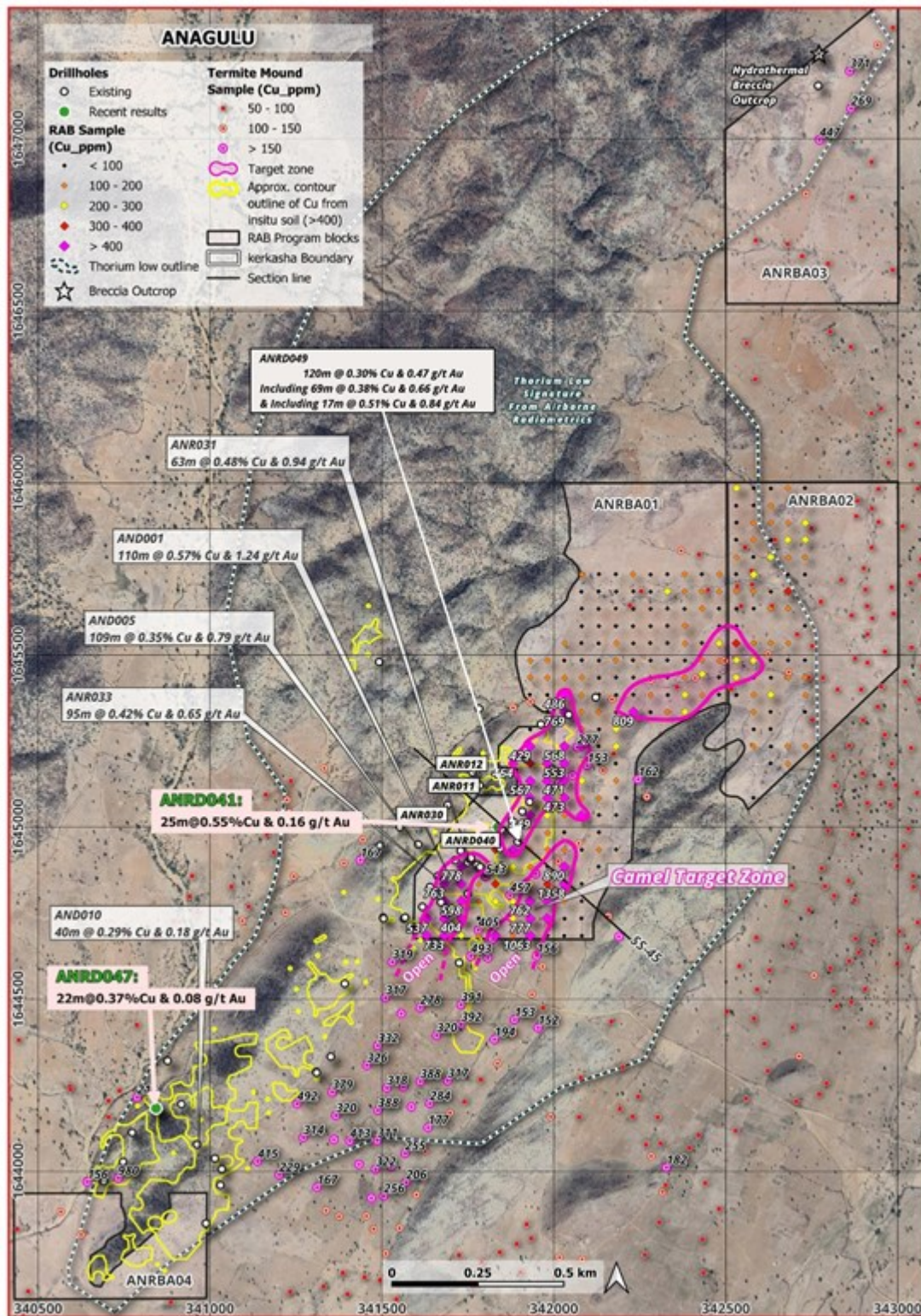
Figure 1: Map Showing RAB Drilling, Termite Mound Sampling Results, Newly Identified Target Zones with Drill holes ANRD041/ANRD049 Locations, and Previous Reported Selected Drilling Results.
