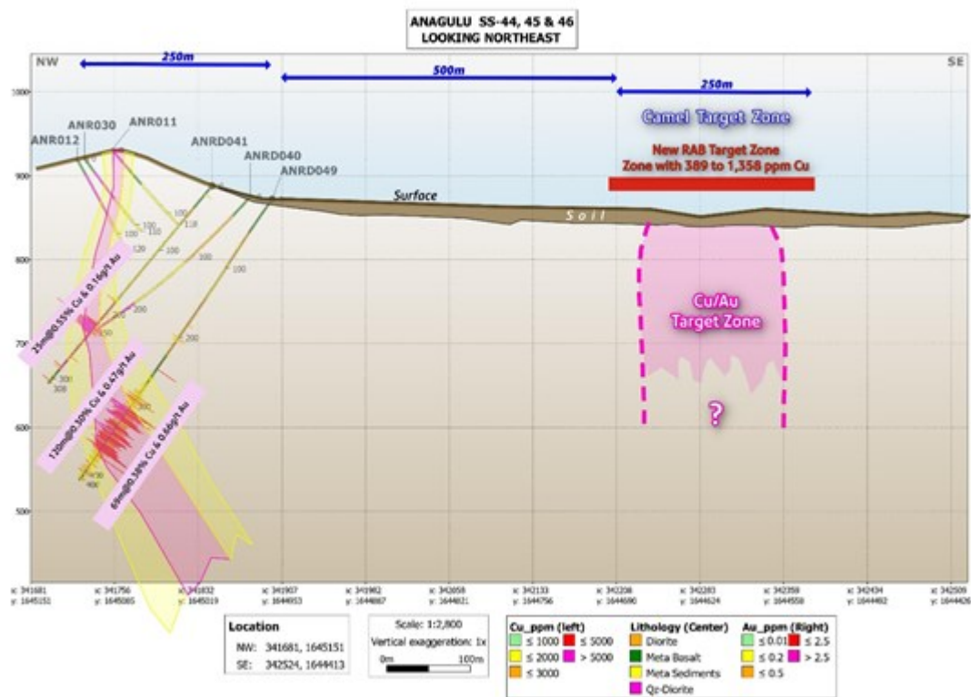
Figure 2: Cross Section SS-45 Showing ANRD041 and ANRD049 with Drill Holes from Lines SS-46 & SS-44 Projected (40 metres) and Position of New Camel Target Zone (1,358 to 389ppm Copper over ~250m width)
