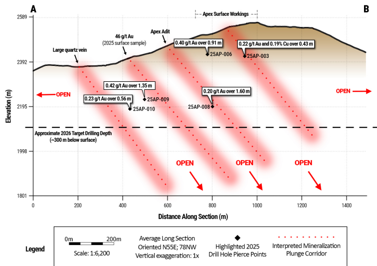
Figure 1. Long section of the Apex gold system showing highlighted 2025 drill pierce points with associated assays, interpreted mineralized plunge corridors, and the approximate depth of planned 2026 drilling. The 2026 program is designed to test the continuity of multiple interpreted mineralized plunge corridors that remain open along strike and at depth.
