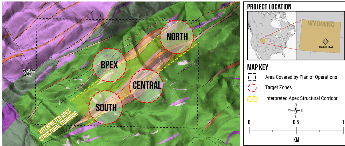
Figure 2. Bradley Peak overview showing the principal 2026 exploration target areas within the approved five-year Plan of Operations. Follow-up drilling will systematically evaluate the interpreted Apex structural corridor through testing of the Northern, Central and Southern Inflection targets and the BPEX shear zone, while maintaining flexibility to advance additional targets across the Bradley Peak Gold Camp.
