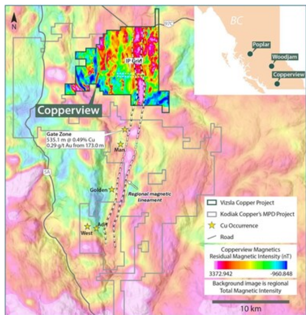
Figure 1. Map of the Copperview Project showing the location of the M5 target in relation to a regional magnetic-high lineament and Kodiak Copper's Gate discovery (CNW Group/Vizsla Copper Corp.)
