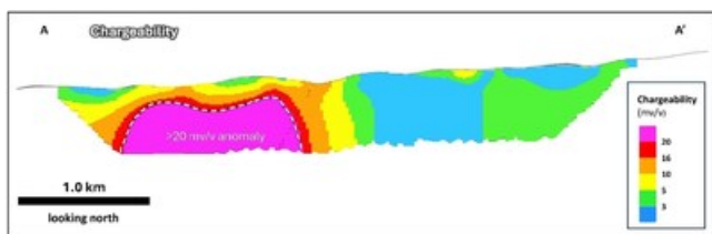
Figure 3. Section through the M5 chargeability 3D voxel model showing the strong-chargeability anomaly which has never been drill tested. Section line A to A' shown in Figure 2. (CNW Group/Vizsla Copper Corp.)
