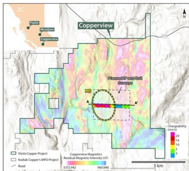
Figure 2. Project scale high-resolution magnetic data showing the location of the IP survey and the strong chargeability anomaly across the M5 target (300m depth slice). (CNW Group/Vizsla Copper Corp.)
