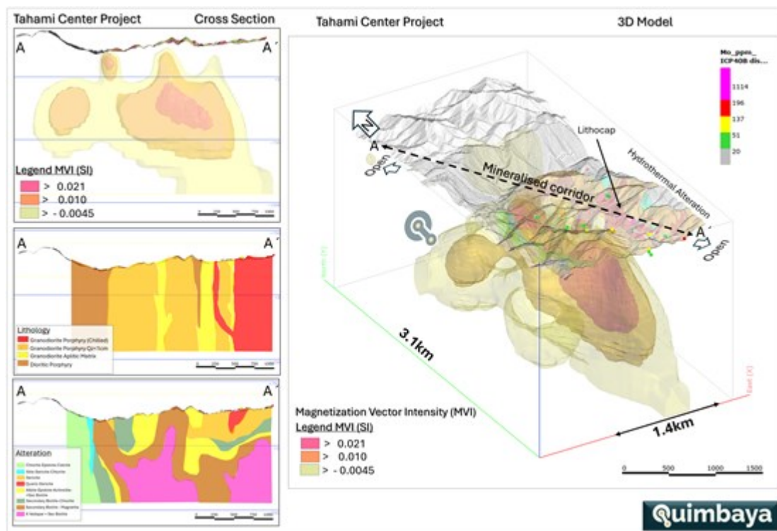
Figure 4. 3D Magnetization Vector Intensity model vs hydrothermal alteration map with the dashed line outlines interpreted mineralised corridor (right). Cross sections of the MVI, Lithology and alteration (left).
