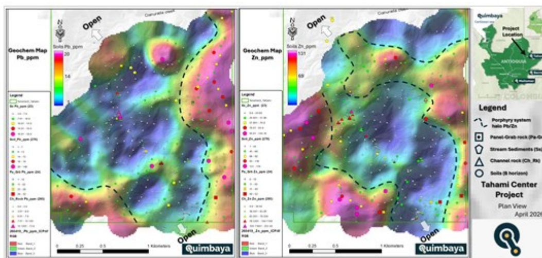
Figure 3. Plan view— Pb and Zn peripheral halos, Tahami Center. Distal Pb-Zn signature surrounding the Cu-Mo core is characteristic of classical porphyry metal zonation.
