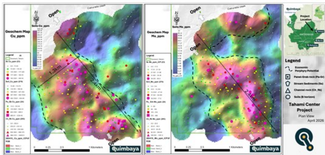
Figure 2. Plan view— Cu and Mo soil geochemistry, Tahami Center. Coherent 2.4 × 1.3 km NW-SE corridor. System open in all directions.
