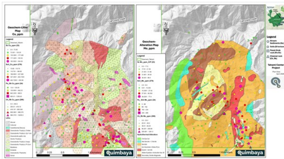
Figure 1. Plan view of the Tahami Center Project showing Lithology map / copper (left) values, and hydrothermal alteration map / molybdenum (right) geochem values, rock and stream sediments geochemistry anomalies associated with the porphyry Cu-Mo-Au system. Dashed line outlines interpreted mineralised corridor.
