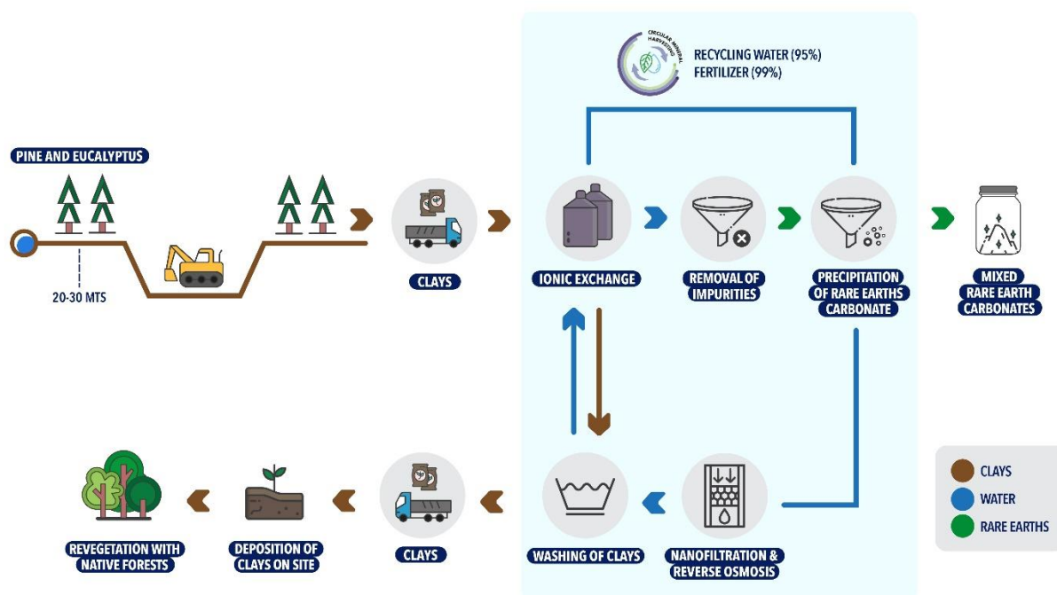
Fig. 2. Aclara's Rare Earths extraction process - Circular Mineral Harvesting
