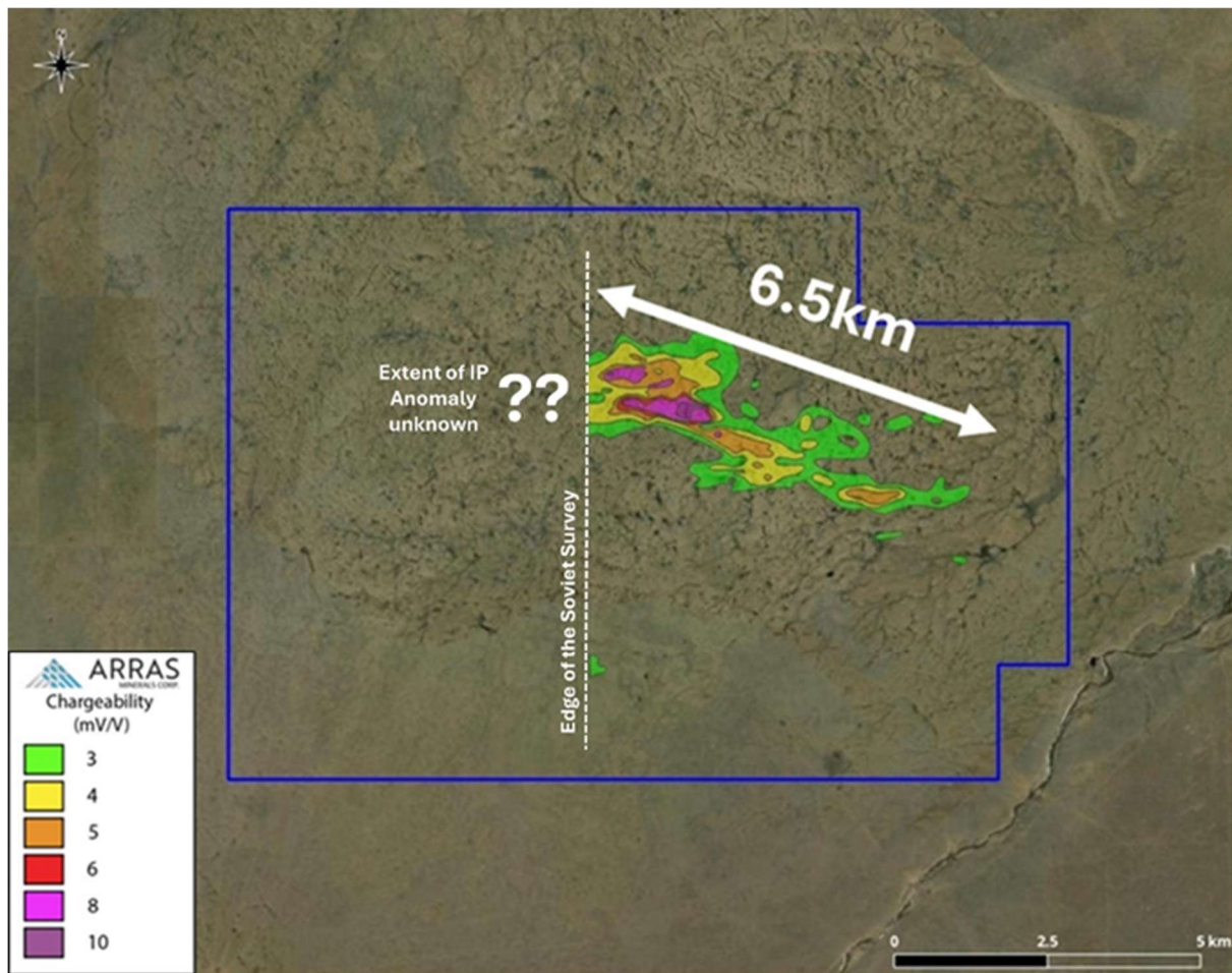
Figure 3. Tay Property historical Soviet IP Chargeability Anomaly.
