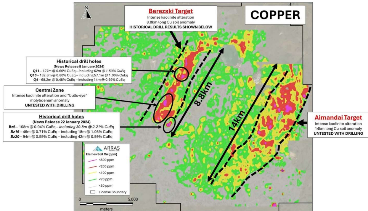
Figure 2. The 14-kilometre long Aimandai and 8.8-kilometre long Berezska Copper Targets are shown as NE-SW trending copper soil anomalies. The location of historical drill holes is also shown on the Berezska anomaly. There is no known drilling on the Aimandai anomaly.
