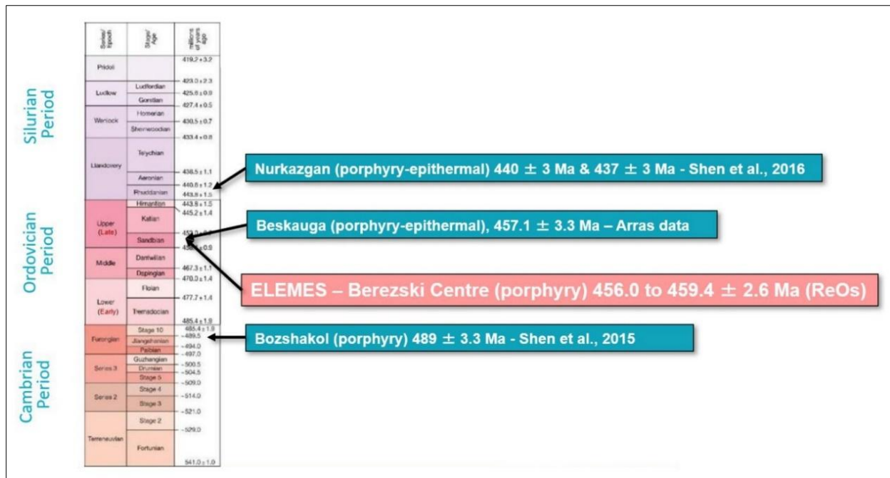
Figure 12. Elemes is hosted in the right belt and is of similar ages to other large porphyry deposits in the area
