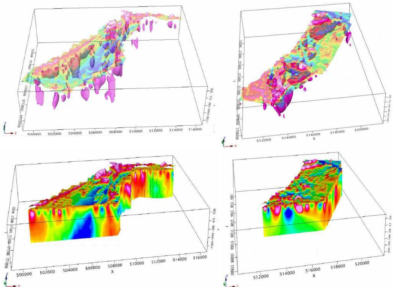
Figure 30. Magnetic Susceptibility Voxels (Berezki to the left, Aimandai to the right)
