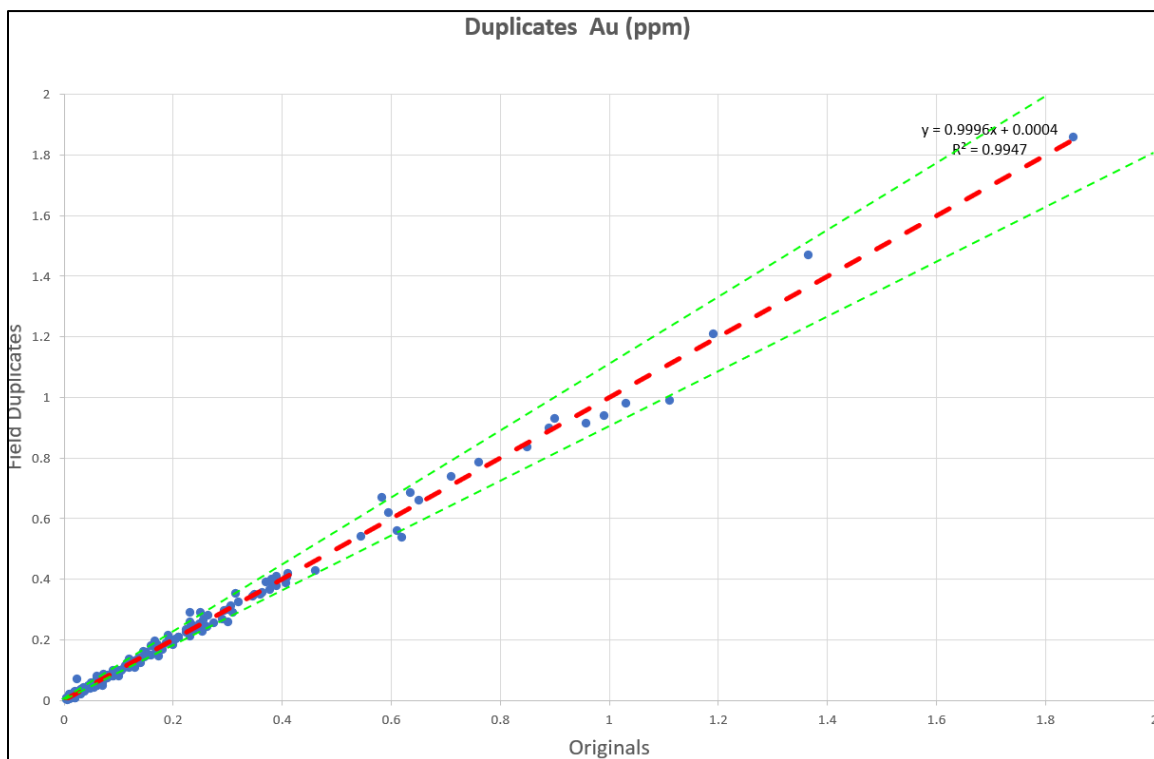
Figure 60. Linear regression of gold for duplicates from 2025
