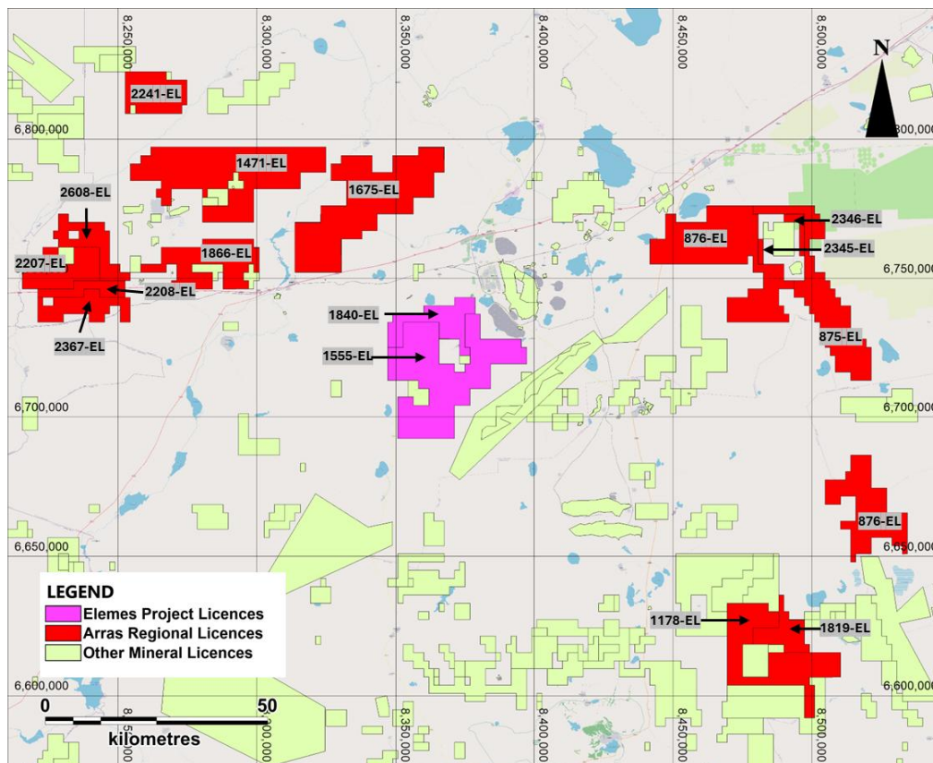
Figure 3. Location of the Elmes Project licences, shown in pink, in relation to the broader regional licence package controlled by Arras, shown in red. Other mineral licences in the area are shown in green
