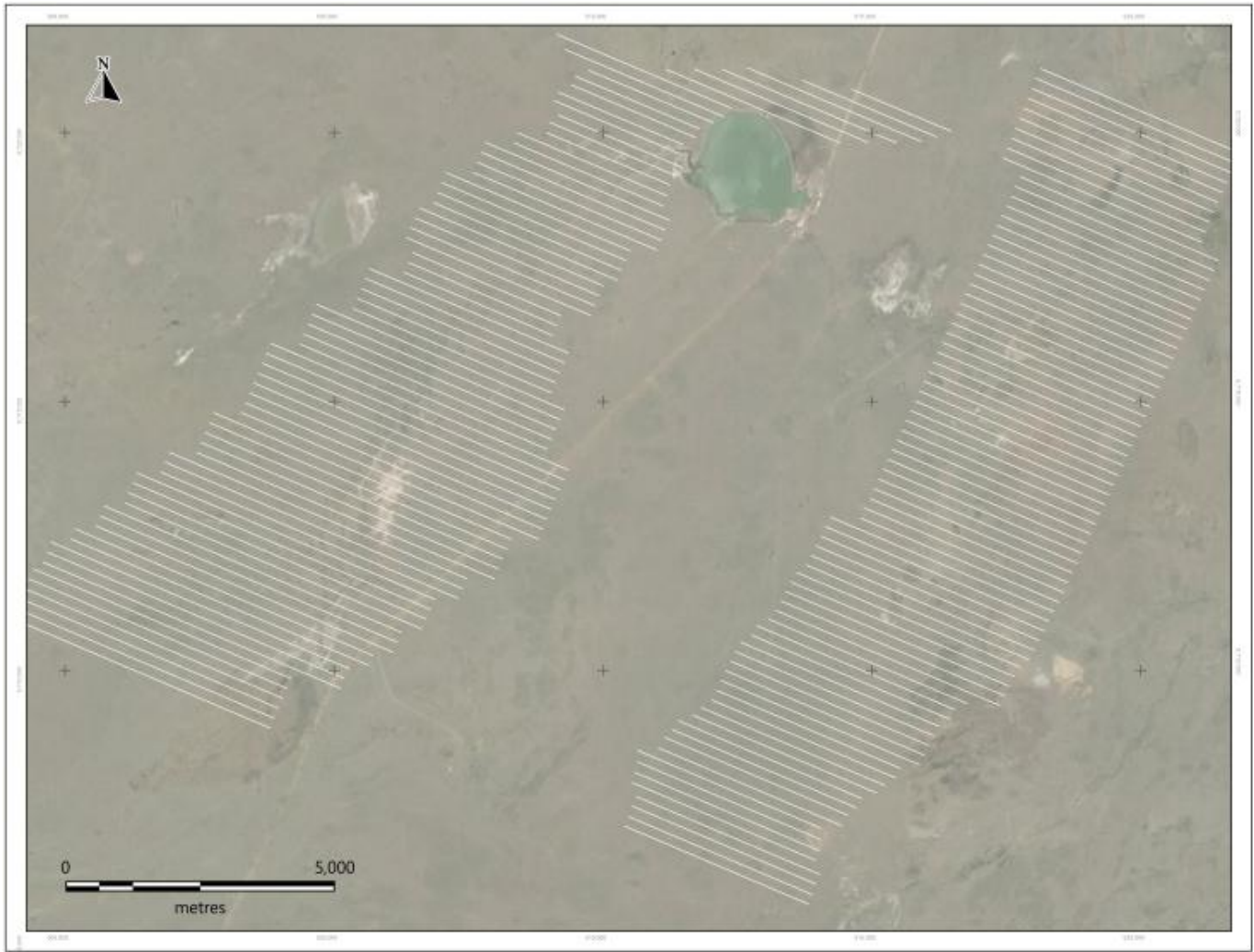
Figure 29. Location map of the planned round magnetic survey lines over Berezski and Aimandai
