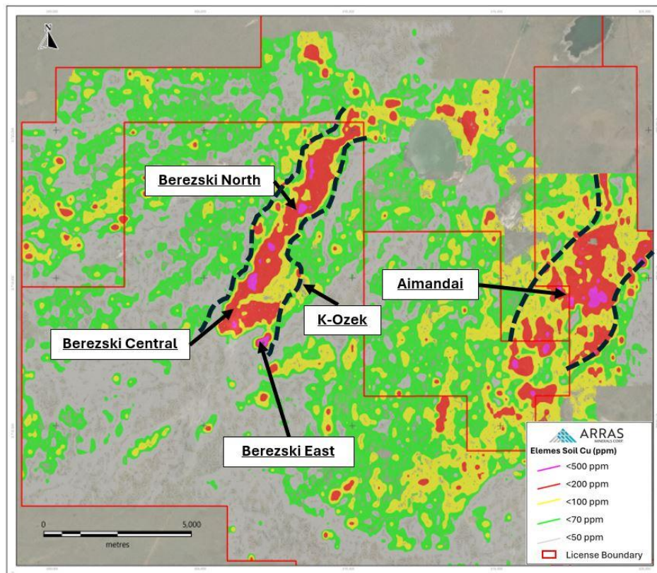
Figure 25. Soil sampling program over Elmes project - pXRF results for copper highlighting two major trends Berezski and Aimadai
