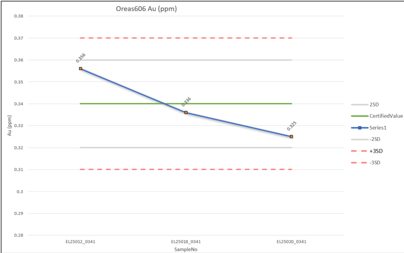
Figure 56. OREAS 606 Shewhart Control Chart for gold
