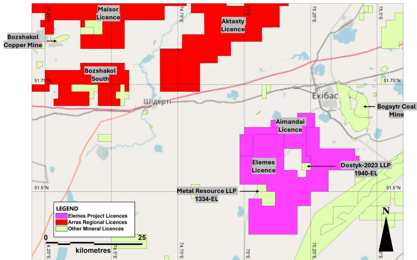
Figure 62. The location of the Elmes Project in relation to other Mines and exploration licences in the area
