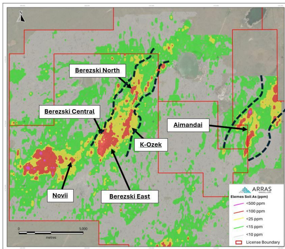
Figure 26. Soil sampling program over Elmes project - pXRF results for arsenic
