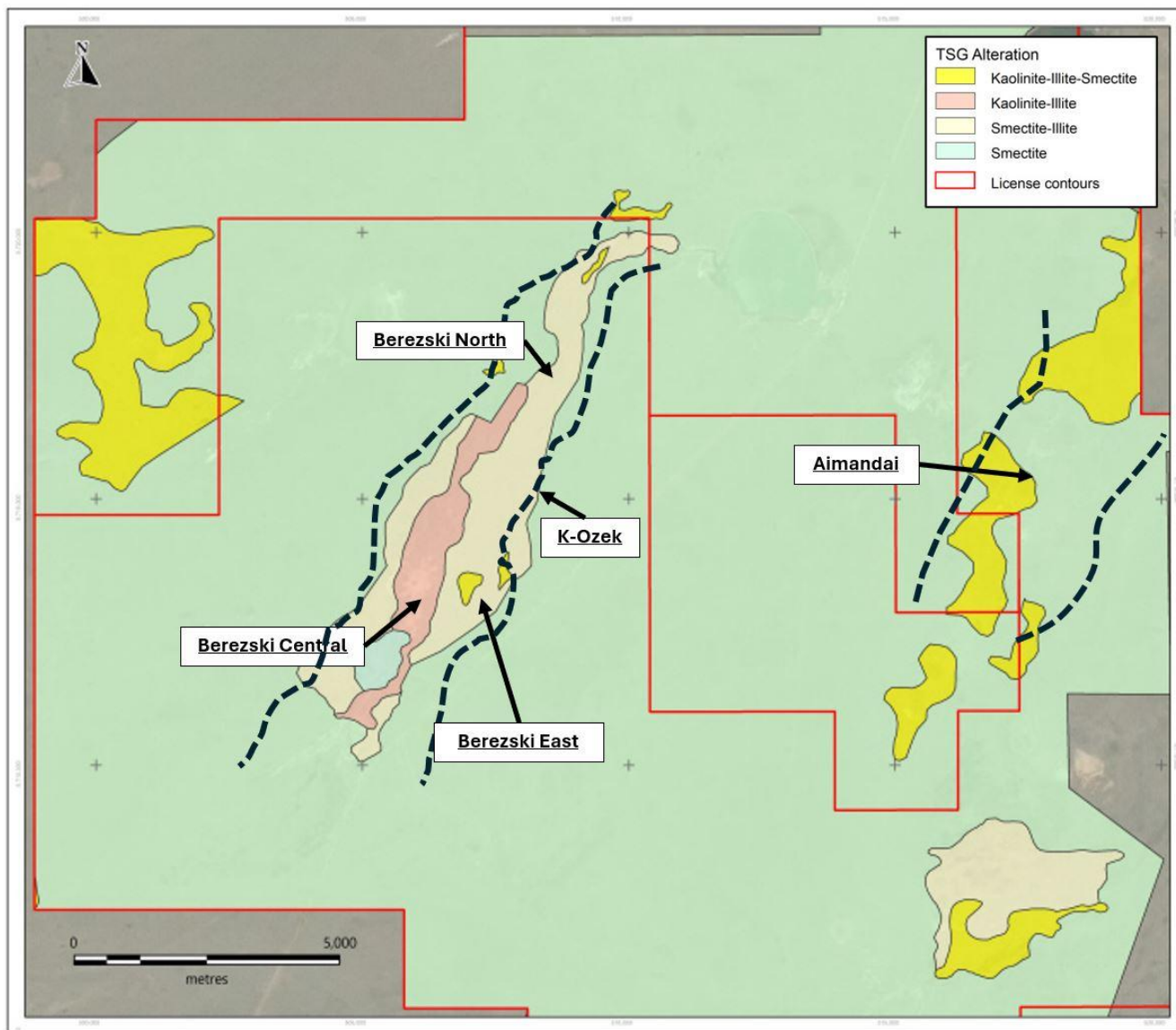
Figure 27. Soil sampling program over Elemes project - TSG detected alteration mineral assemblages
