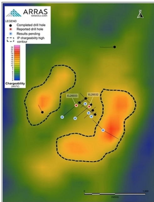
Figure 5. Berezski North target with drill holes drilled to date superimposed on the IP chargeability slice at -100.0 m depth. Strong IP chargeability high envelope surrounding the drilled area with proven porphyry style mineralization.
