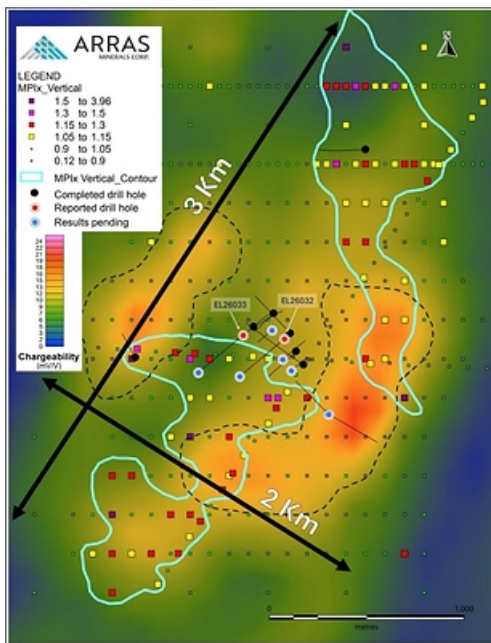
Figure 8. Berezski North target Soil ALS results - porphyry pathfinder elements interpreted using MDRU Porphyry Index (MPIx_Vertical)
