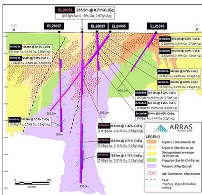
Figure 3. Long Section drill-hole, Berezski North Target showing Arras drill-hole intercepts including hole EL26032. Notes: For copper and gold equivalent calculations the following metal process were used: US$3.75/lb. Copper, US$3,000/oz Gold, US$35/oz Silver, US$30/lb Molybdenum, and metallurgical recoveries have been updated to Cu 90%, Au 85%, Ag 75%, Mo 80%. All intervals are presented as core lengths as the true thicknesses of mineralization is currently unknown.
