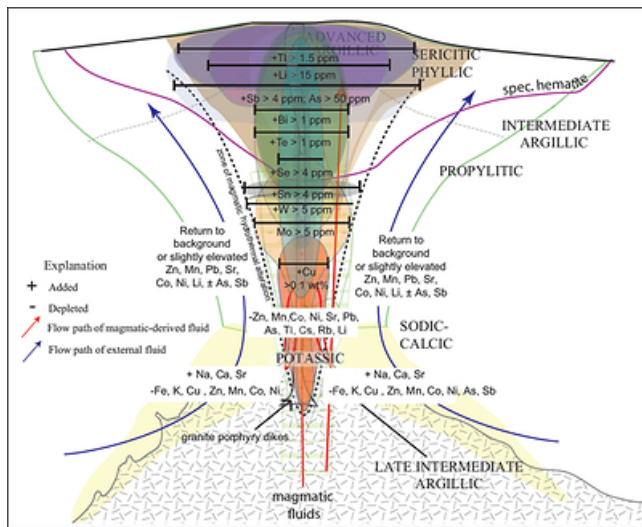
Figure 7. Vertical cross section of a typical porphyry Cu deposit showing distribution of hydrothermal alteration and sulfide minerals. Also shown are generalized contours of the 2,200-nm peak measured in SWIR instruments (Halley et al, 2015)
