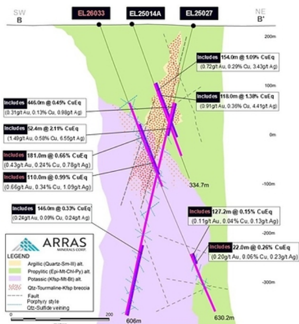
Figure 4. Cross Section, Berezski North Target showing Arras drill-hole intercepts including hole EL26033. Notes: For copper and gold equivalent calculations the following metal process were used: US$3.75/lb. Copper, US$3,000/oz Gold, US$35/oz Silver, US$30/lb Molybdenum, and metallurgical recoveries have been updated to Cu 90%, Au 85%, Ag 75%, Mo 80%. All intervals are presented as core lengths as the true thicknesses of mineralization is currently unknown.
