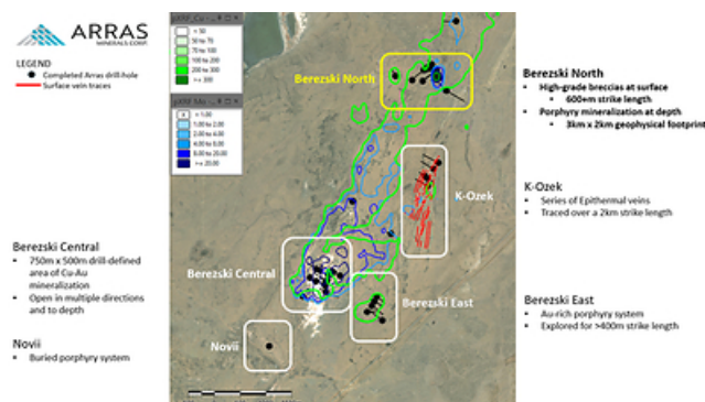
Figure 1. Berezski Trend showing principal targets
