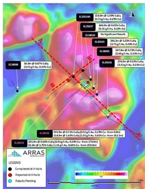
Figure 2. Berezski North Targets with completed drill-holes overlain on reduction to pole (“RTP”) ground magnetic survey data. Notes: For copper and gold equivalent calculations the following metal process were used: US$3.75/lb. Copper, US$3,000/oz Gold, US$35/oz Silver, US$30/lb Molybdenum, and metallurgical recoveries have been updated to Cu 90%, Au 85%, Ag 75%, Mo 80%. All intervals are presented as core lengths, as the true thicknesses of mineralization are currently unknown.
