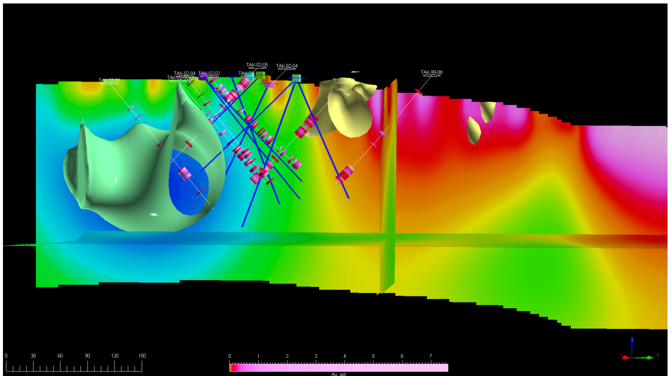
Image 1: Tak Drill Plan Section - Looking WSW - Res 20k ohm - CHG 30ms - Au >0.1 g/t
