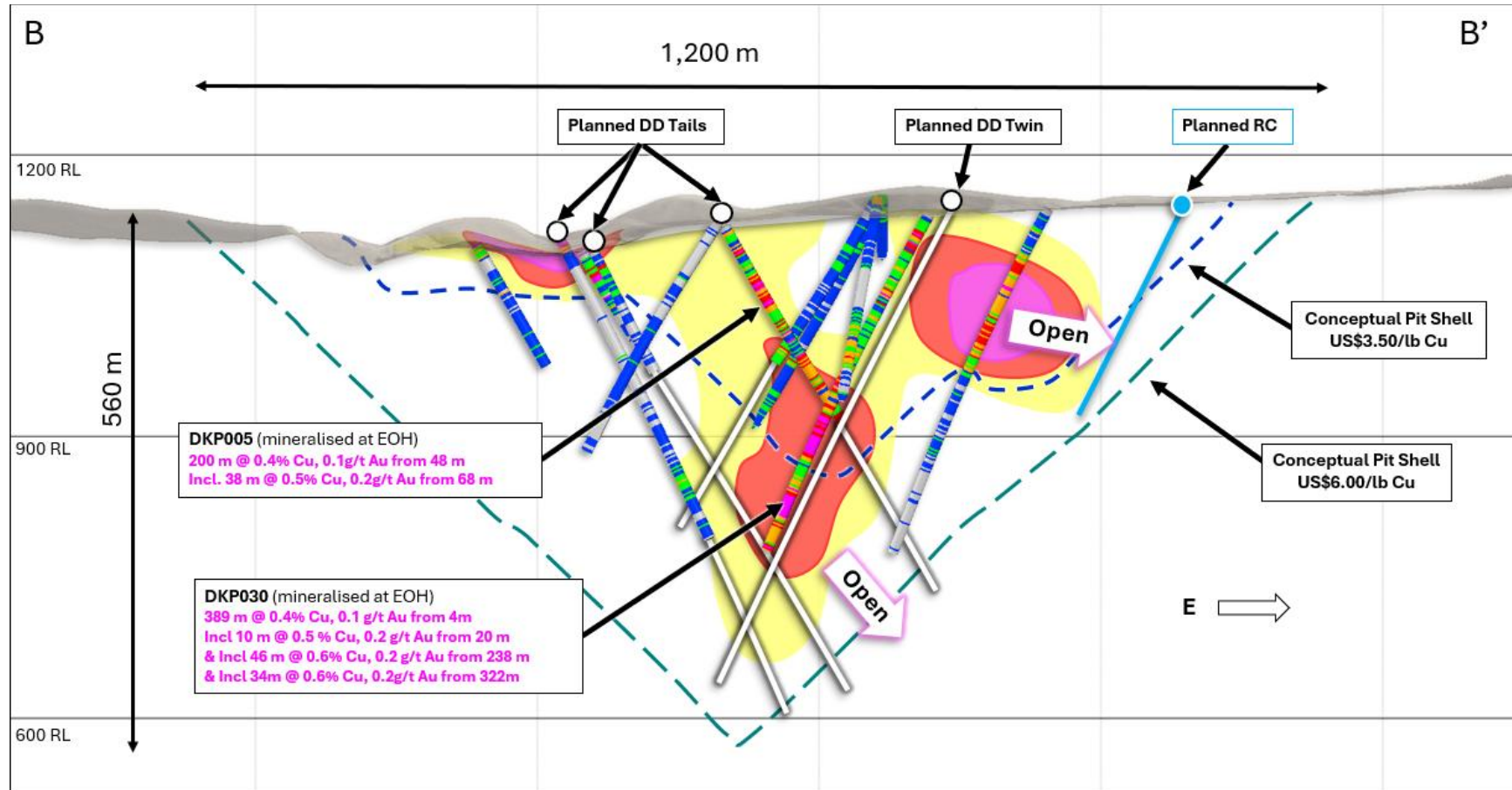
Figure 3. (Top) North facing cross section B - B' (± 75m clipping), (Bottom) and North facing cross section C-C' (± 75m clipping) through the La Verde porphyry system showing planned diamond and RC drill holes compared to +0.2% copper (yellow), +0.3% copper (red), +0.4% copper (Magenta) mineralisation interpolants from returned assay results. Conceptual open pit shells 1 displayed for $US3.50/lb Cu (blue) and $US6.00/lb Cu (green) displayed as dashed lines.
