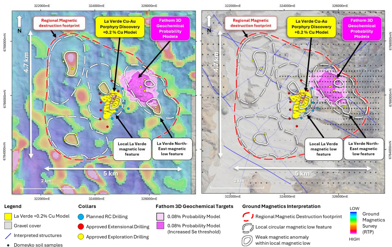
Figure 4. Plan view showing the La Verde +0.2% Cu mineralisation interpolant in relation to regional magnetic destruction footprint (red dashed), local magnetic low features (white dashed), weakly magnetic anomalies (white line) and Fathom 3D geochemical probability models (purple isosurfaces). Left – shown overlain on reduced-to-the-pole (RTP) ground magnetics. Right – shown in relation to mapped gravel cover, interpreted regional structures and soil sample coverage. See announcement dated 29 May 2025 for JORC Table 1 additional technical information.
