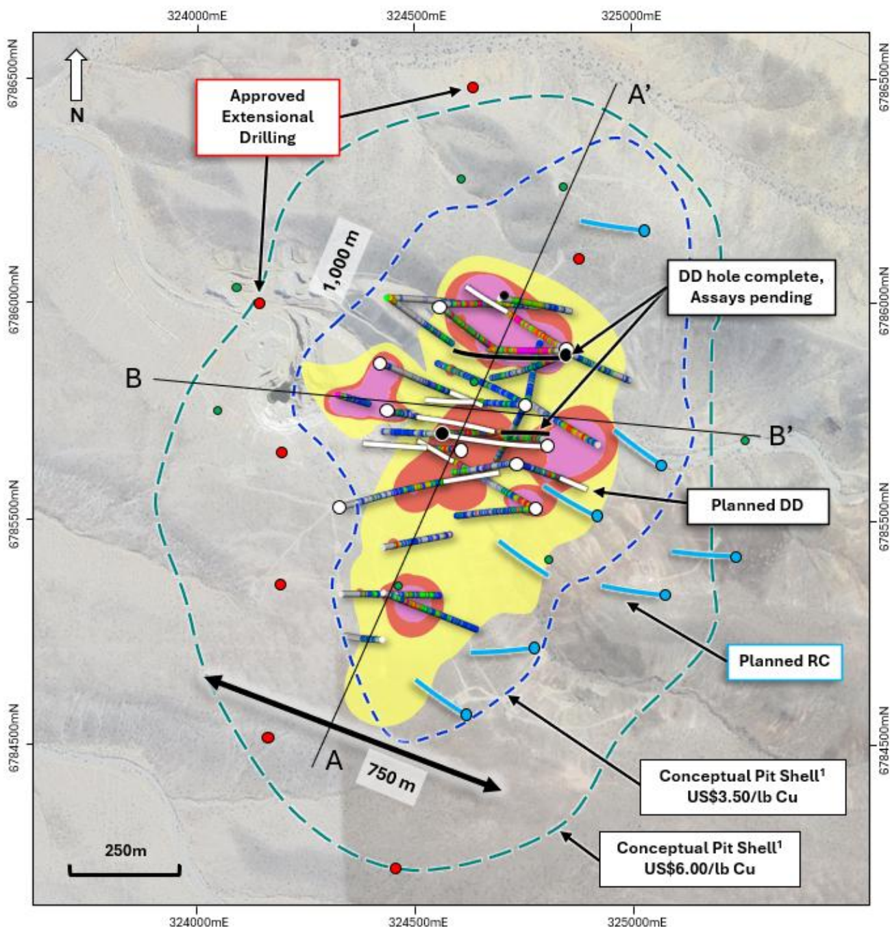
Figure 1. Plan view map of the La Verde porphyry system showing approved extensional collar locations (red points), planned (white traces) and completed DD drilling (black) compared with +0.2% copper (yellow), +0.3% copper (red), +0.4% copper (Magenta) mineralisation interpolants from Phase one drilling. Conceptual open pit shells 1 displayed for $US3.50/lb Cu (blue) and $US6.00/lb Cu (green) displayed as dashed lines. See announcement dated 25 September 2025 for JORC Table 1 additional technical information.
