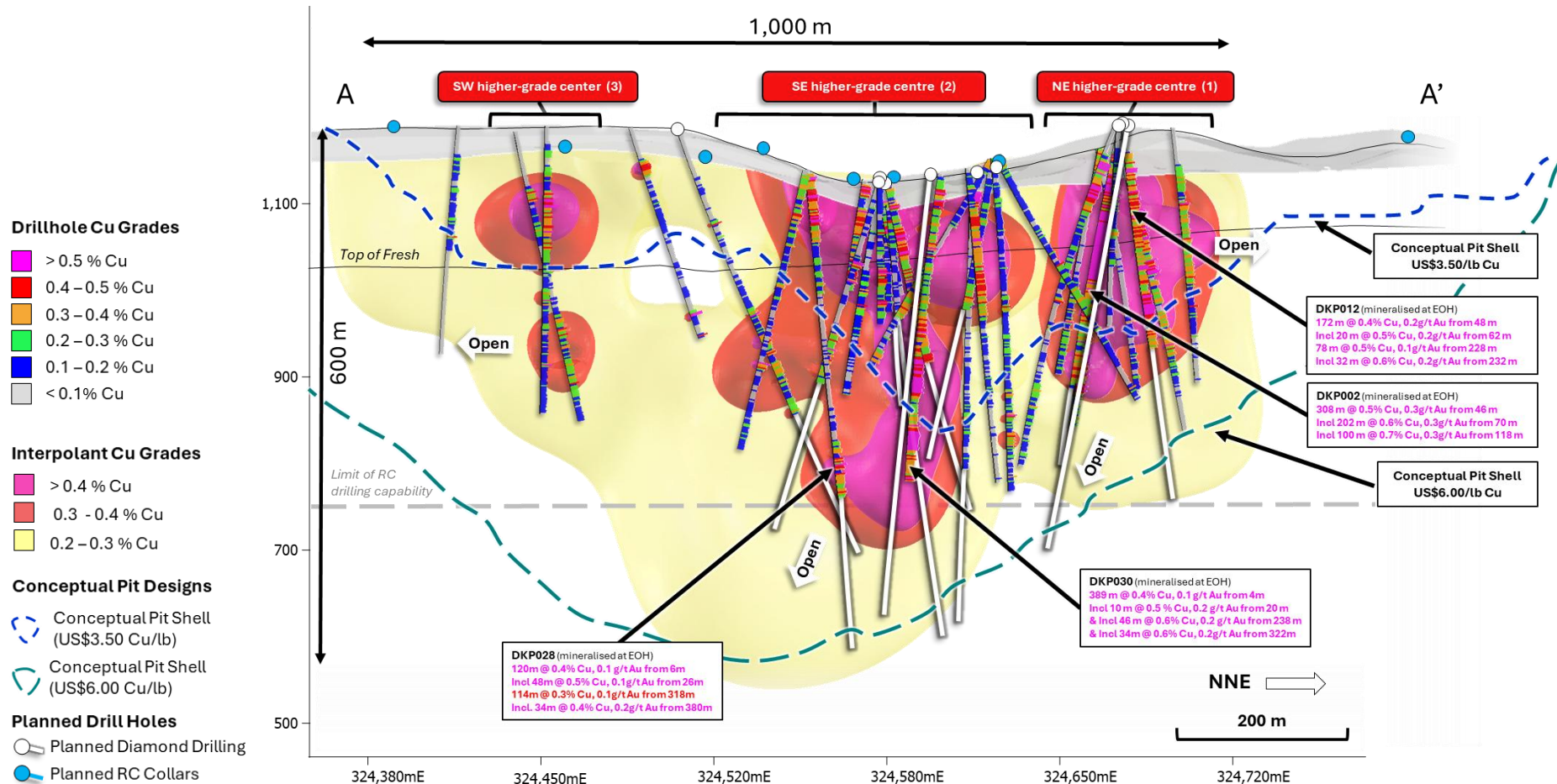
Figure 2. NNW facing longitudinal section (A - A') of the La Verde porphyry system showing planned diamond drill hole traces, and planned RC collars compared to +0.2% copper (yellow), +0.3% copper (red), +0.4% copper (Magenta) mineralisation interpolants from returned assay results. Weathering profile displayed as top of fresh material (black line). Returned Cu grades graphed downhole along hole traces (grey). Conceptual open pit shells 1 displayed for US$3.50/lb Cu (blue) and US$6.00/lb Cu (green) displayed as dashed lines.
