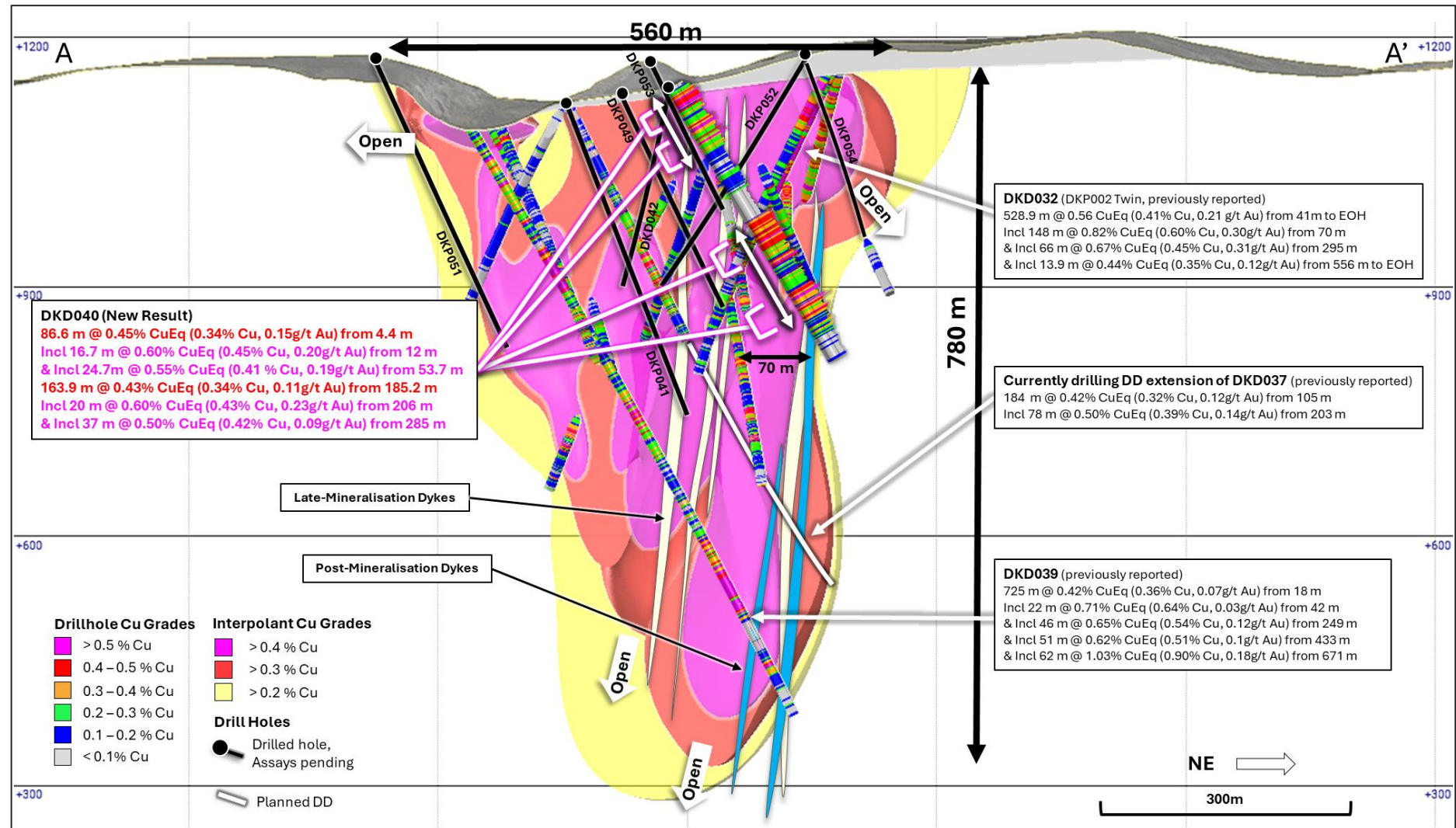
Figure 3. Cross section slice along DKD040 ( \pm 75\text{m} clipping) showing +0.2% copper (yellow), +0.3% copper (red), +0.4% copper (magenta) mineralisation interpolants and returned assay results for DKD040. Returned Cu grades shown on hole traces. Results reported including CuEq 1 .
