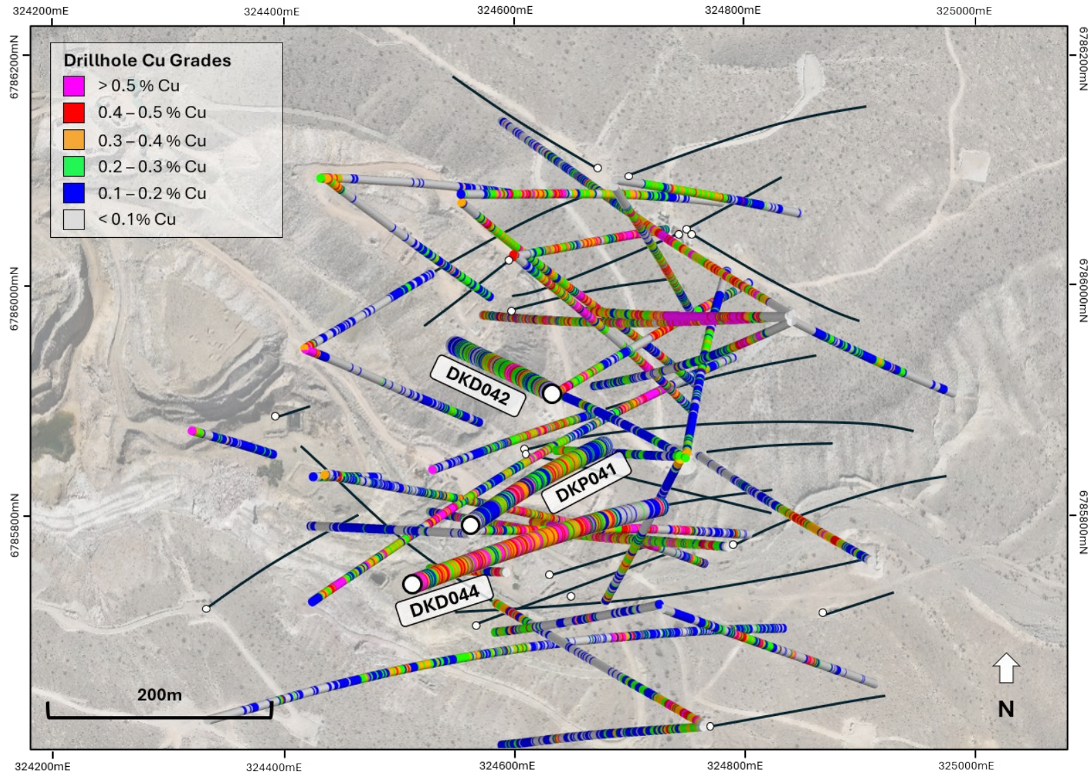
Figure 4. Zoomed plan view map of La Verde showing recent drill hole results DKD044, DKD042 and DKP041, returned Cu grades shown on hole traces. Drilled holes with pending assays are shown in black.
