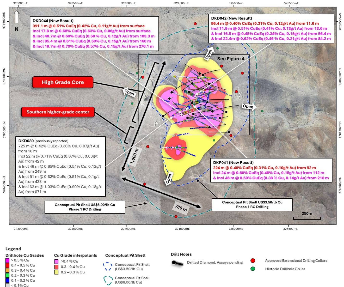
Figure 2. Plan view map of La Verde showing recent drill hole results DKD044, DKD042 and DKP041 and updated +0.2% copper (yellow), +0.3% copper (red), +0.4% copper (magenta) mineralisation interpolants. Drilled holes with pending assays are shown in black. Position of A – A' cross section annotated with white dashed lines. Conceptual open pit shells 1 displayed for US$3.50/lb Cu (blue) and US$6.00/lb Cu (green) displayed as dashed lines. Results reported including CuEq 2 .
