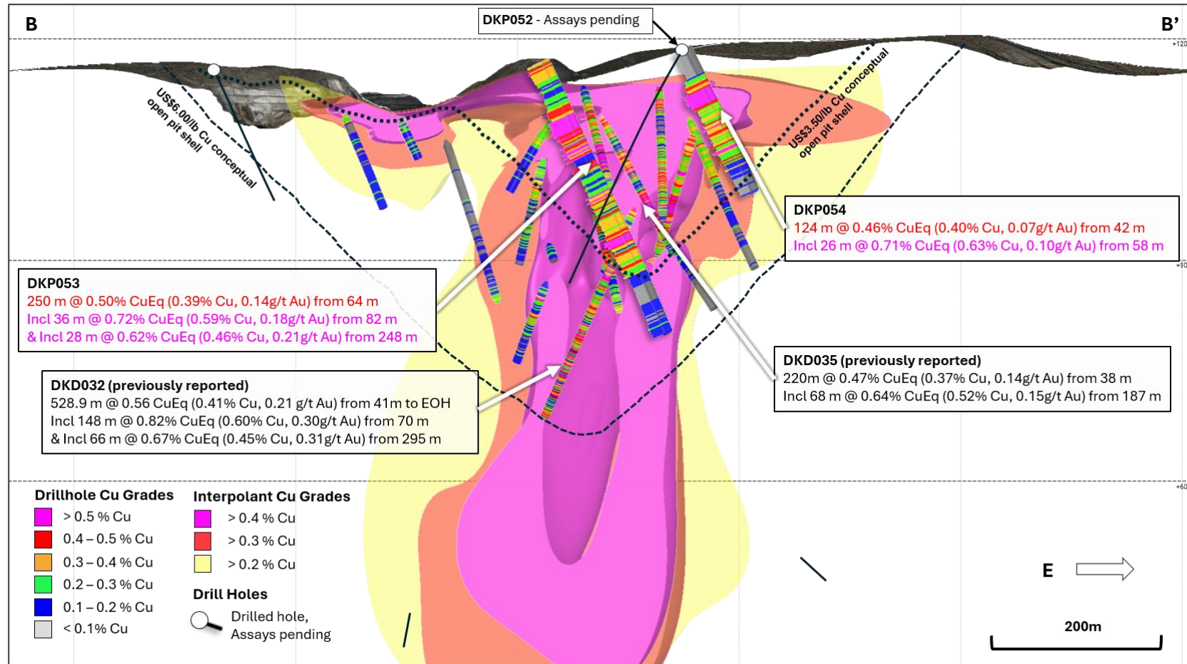
Figure 4. Cross section slice (B – B') showing recent drill hole results DKP053 and DKP054 ( \pm 75\text{m} clipping) and updated +0.2% copper (yellow), +0.3% copper (red), +0.4% copper (magenta) mineralisation interpolants. Returned Cu grades shown on hole traces, drilled holes with pending assays are shown in black. Conceptual open pit shells 1 displayed for $US3.50/lb Cu (blue) and $US6.00/lb Cu (green) displayed as dashed lines. Results reported including CuEq 2 . Assay pending for DKP052.
