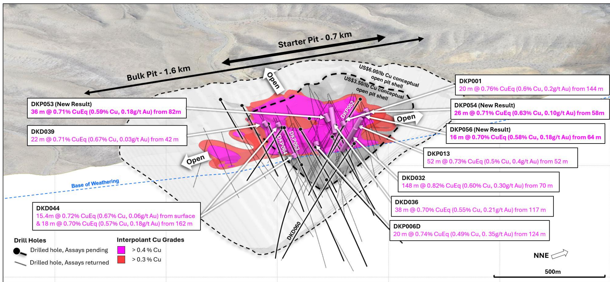
Figure 5. Oblique slice towards NW (Azi 325°, Plunge+26°). 0.3% and 0.4% Cu interpolants displayed for oxide and transitional material, sliced along NNE orientation with the front removed. US$3.50/lb Cu conceptual open pit shell displayed in dark grey; US$6.00/lb Cu conceptual open pit shell displayed in light grey 1 . Base of weathering shown as dashed blue line. Results reported including CuEq 2 .
