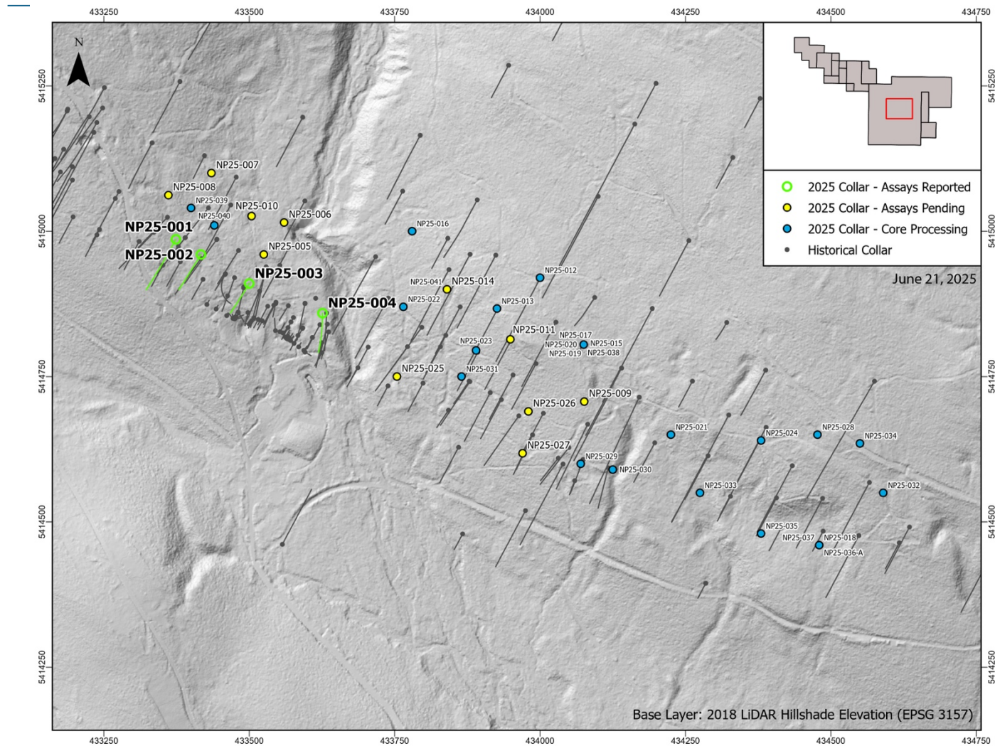
Figure 1: Lara VMS Project – Coronation area Phase 1 drilling locations
