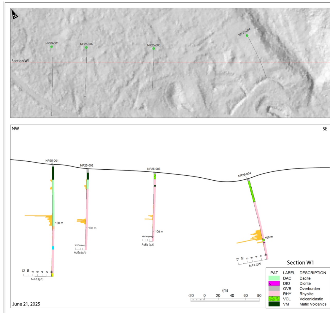
Figure 3: Lara VMS Project – Geological section looking N030°
