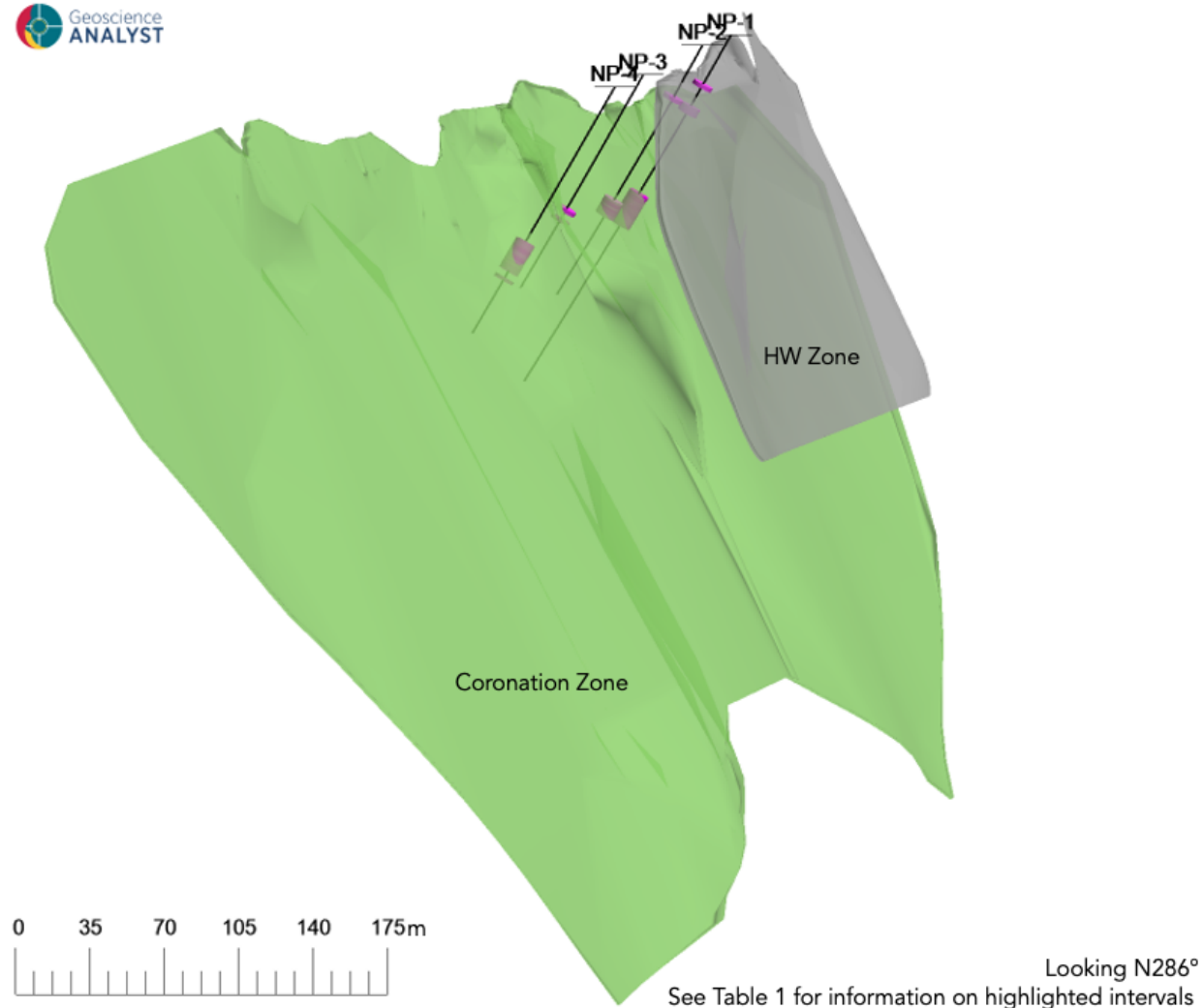
Figure 4: Lara VMS Project – 3D Isometric of Coronation area drillholes in this release looking N286°
