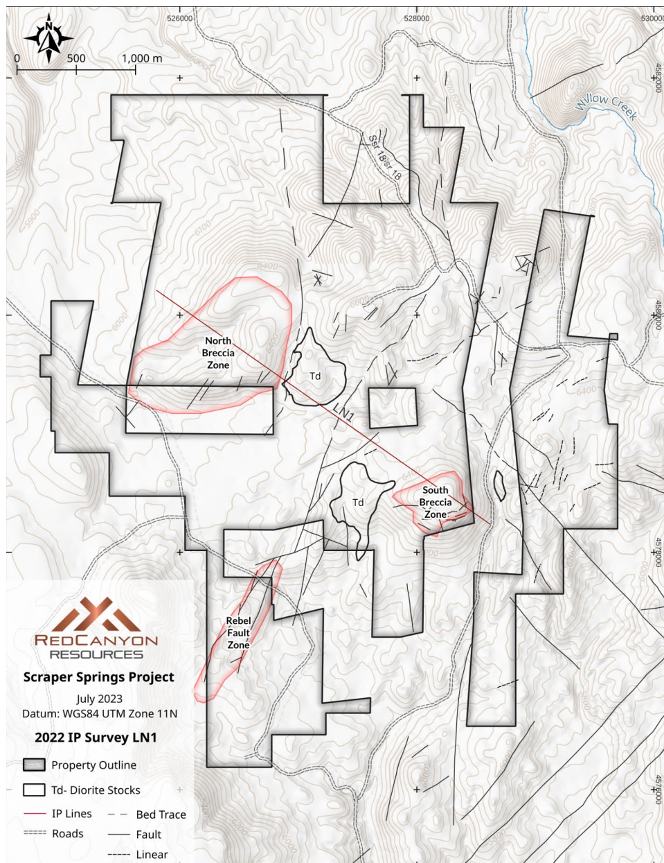
Figure 31: 2022 IP survey Line 1 location
