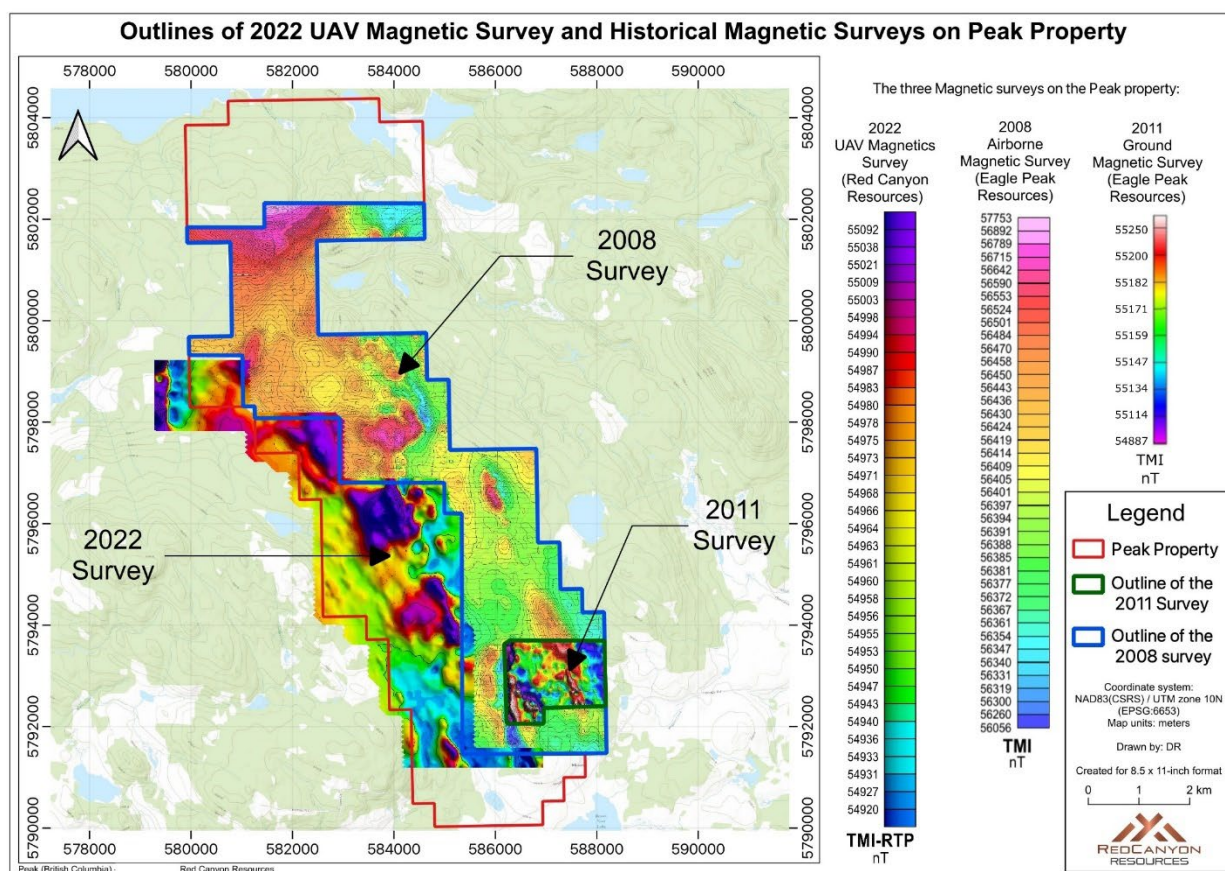
Figure 8: Geophysical Surveys
