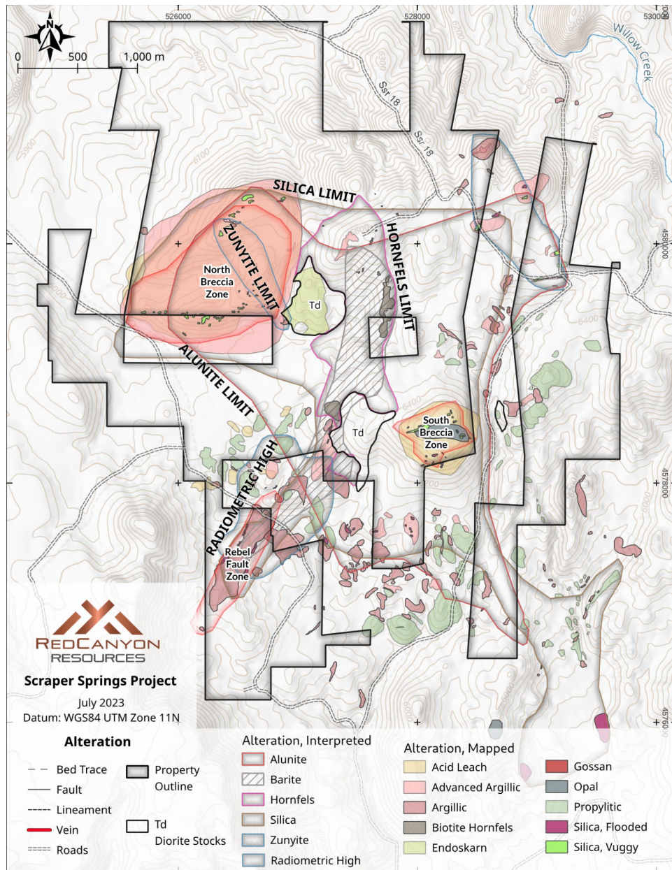
Figure 23: Project alteration map adapted from Wise (2008)
