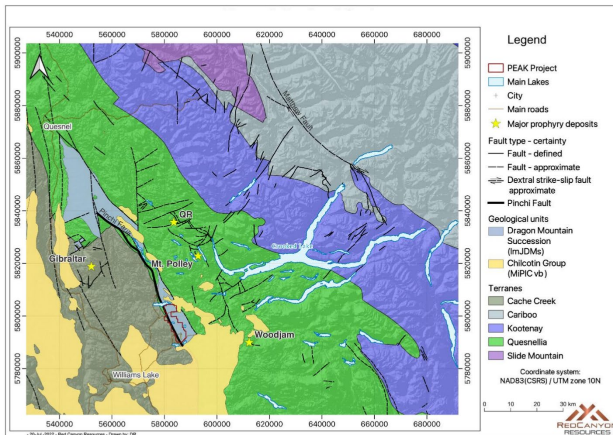
Figure 5: Regional Geology
