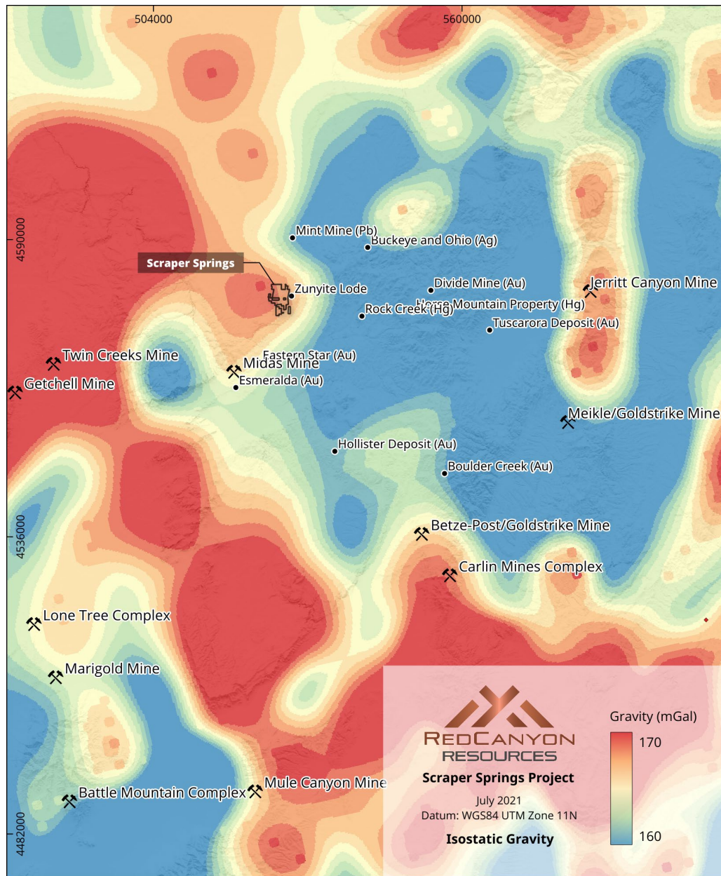
Figure 25: Regional isostatic gravity map of the greater Scraper Springs region (USGS, 1998)
