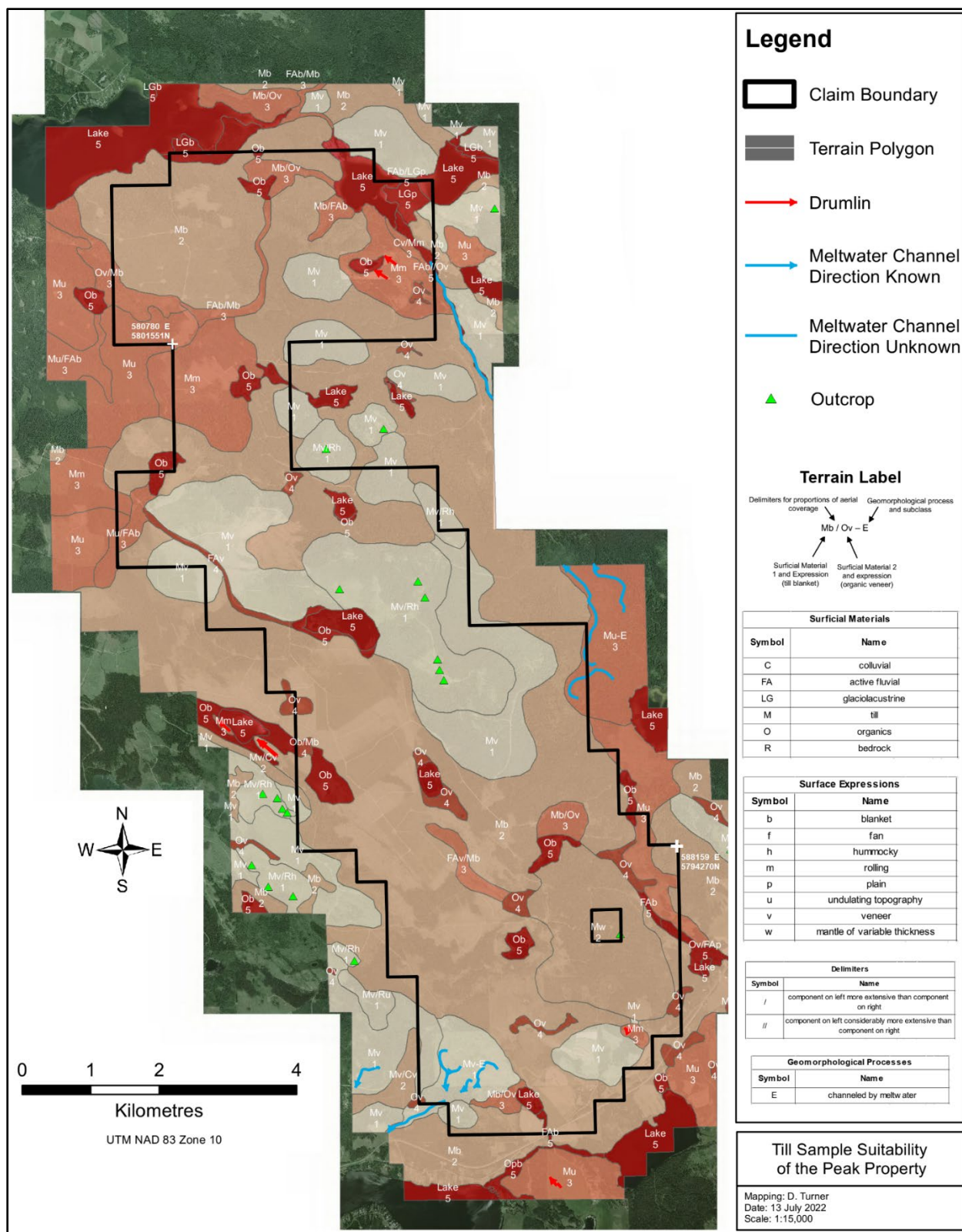
Figure 13: Terrain Surveys
