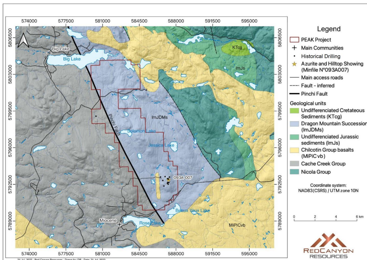
Figure 6: Property Geology
