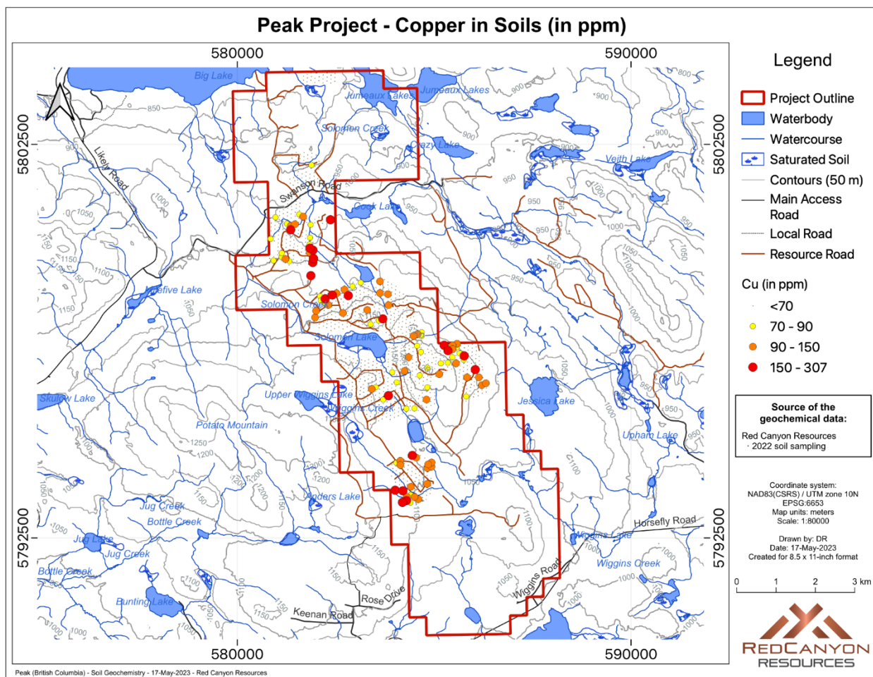
Figure 9: Copper in Soils
