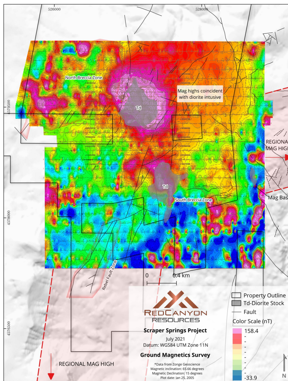
Figure 26: Ground magnetics survey from Zonge Geoscience for Cordex (2004) showing total magnetic field intensity in nT, upward continued to 10 ft and reduced to pole.
