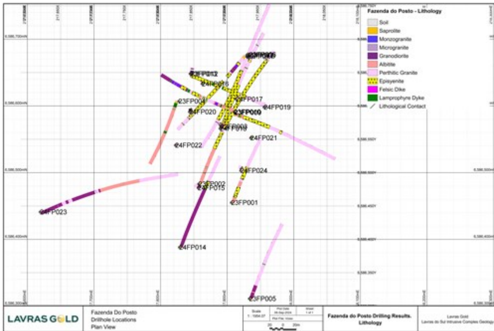
Figure 2. Plan View of 2023 and 2024 Fazenda do Posto Drillholes. (Several drillholes are collared in the same location - refer to Table 2 for details)
