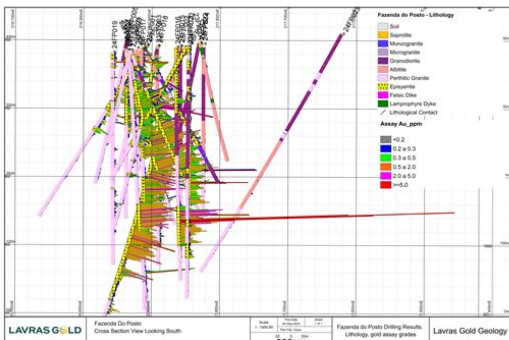
Figure 4. Cross-Section Looking South of 2023 and 2024 Fazenda do Posto Drillholes showing Lithology and Gold Assay Grade.
