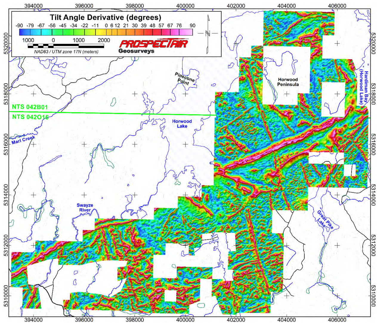
Figure 12 Tilt derivative
