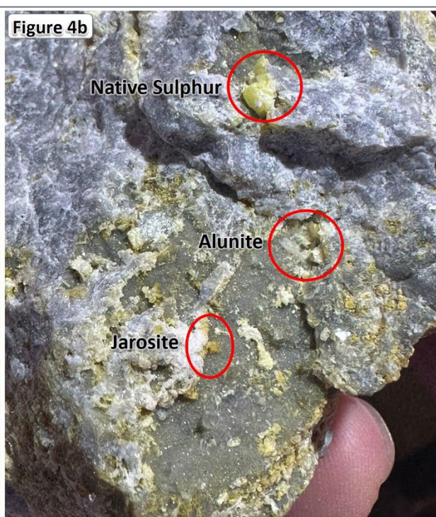
Figure 4b Filon Alunita hydrothermal breccia silica flooding of vuggy silica with late-stage crystalline alunite – native sulphur – jarosite on fractures and voids. No previous rock chip sampling of this breccia.
