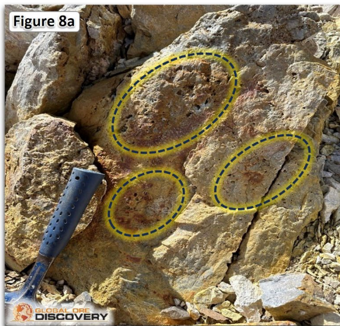
Outcrop of vuggy silica – alunite – jarosite breccia at Meseta prospect. A. Note clustering of leach voids possibly identifying ghosted larger clasts and in B. ghosted clast with pre-brecciation vein. Mogotes sampling of these outcrops returned a peak assay of 1.48 g/t Au, 4.6 g/t Ag, 36 ppm Cu, 822 ppm As and 88ppm Sb.
