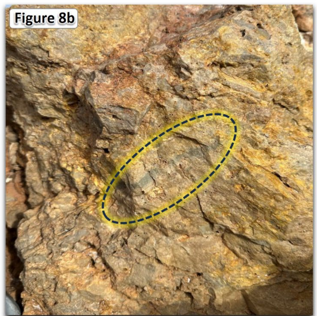
Outcrop of vuggy silica – alunite – jarosite breccia at Meseta prospect. A. Note clustering of leach voids possibly identifying ghosted larger clasts and in B. ghosted clast with pre-brecciation vein. Mogotes sampling of these outcrops returned a peak assay of 1.48 g/t Au, 4.6 g/t Ag, 36 ppm Cu, 822 ppm As and 88ppm Sb.
