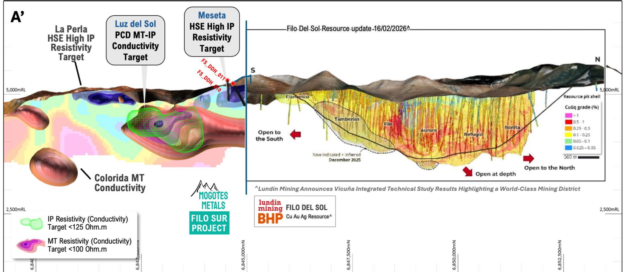
Figure 2: Long section geophysical targets and drilling progress at the Filo Sur Project
