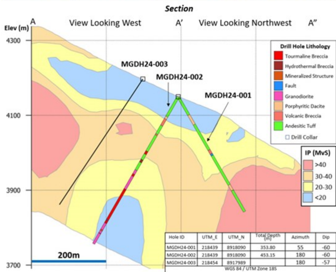
Figure 5 - Plan view and section for Mega-Gold drilling to date. Plan view shows location of drill holes
