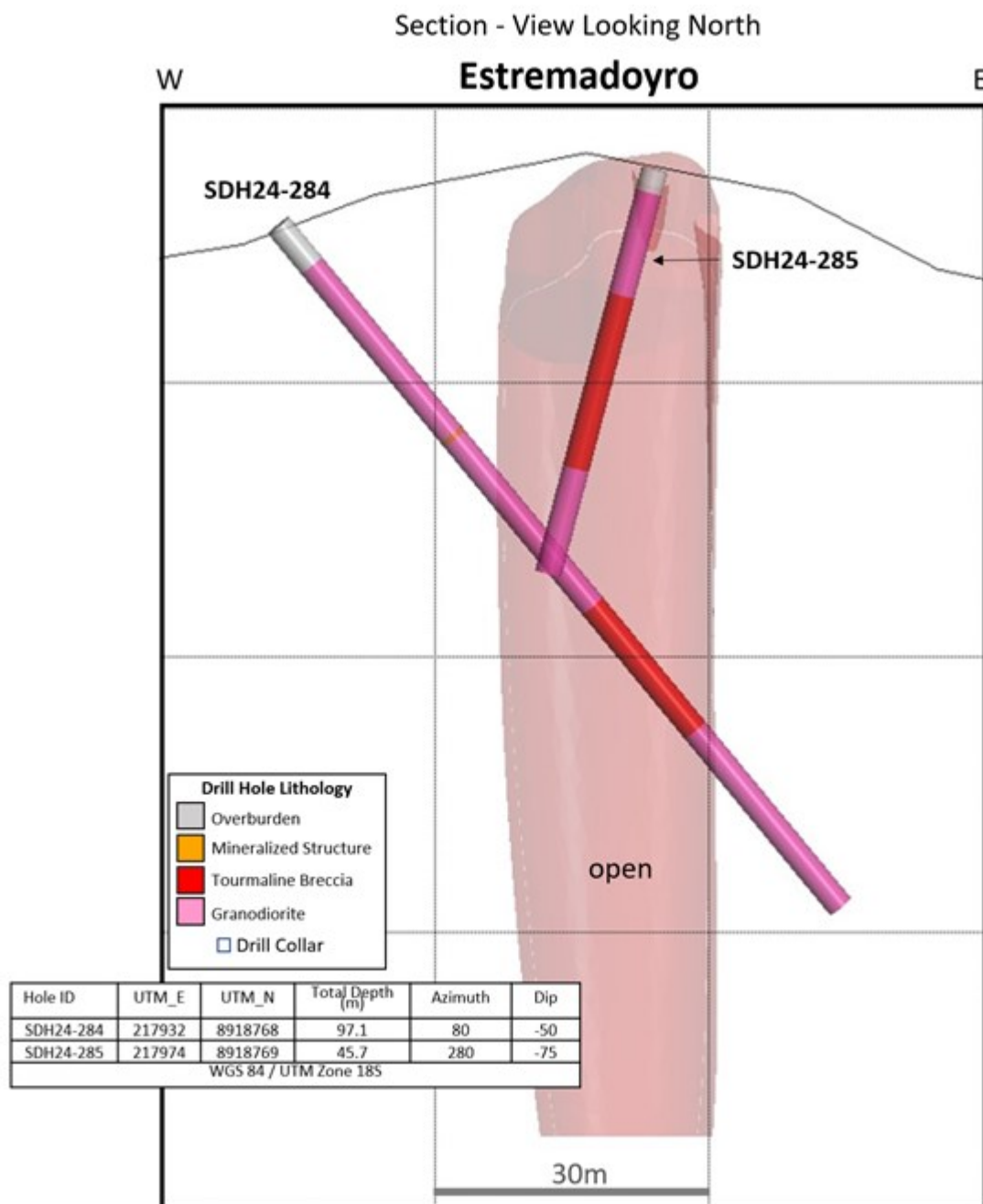
Figure 3 - 3D sectional view of Estremadoyro looking north. Light red 3D shape shows inferred breccia pipe geometry based on surface outcrops and drill intercepts.
