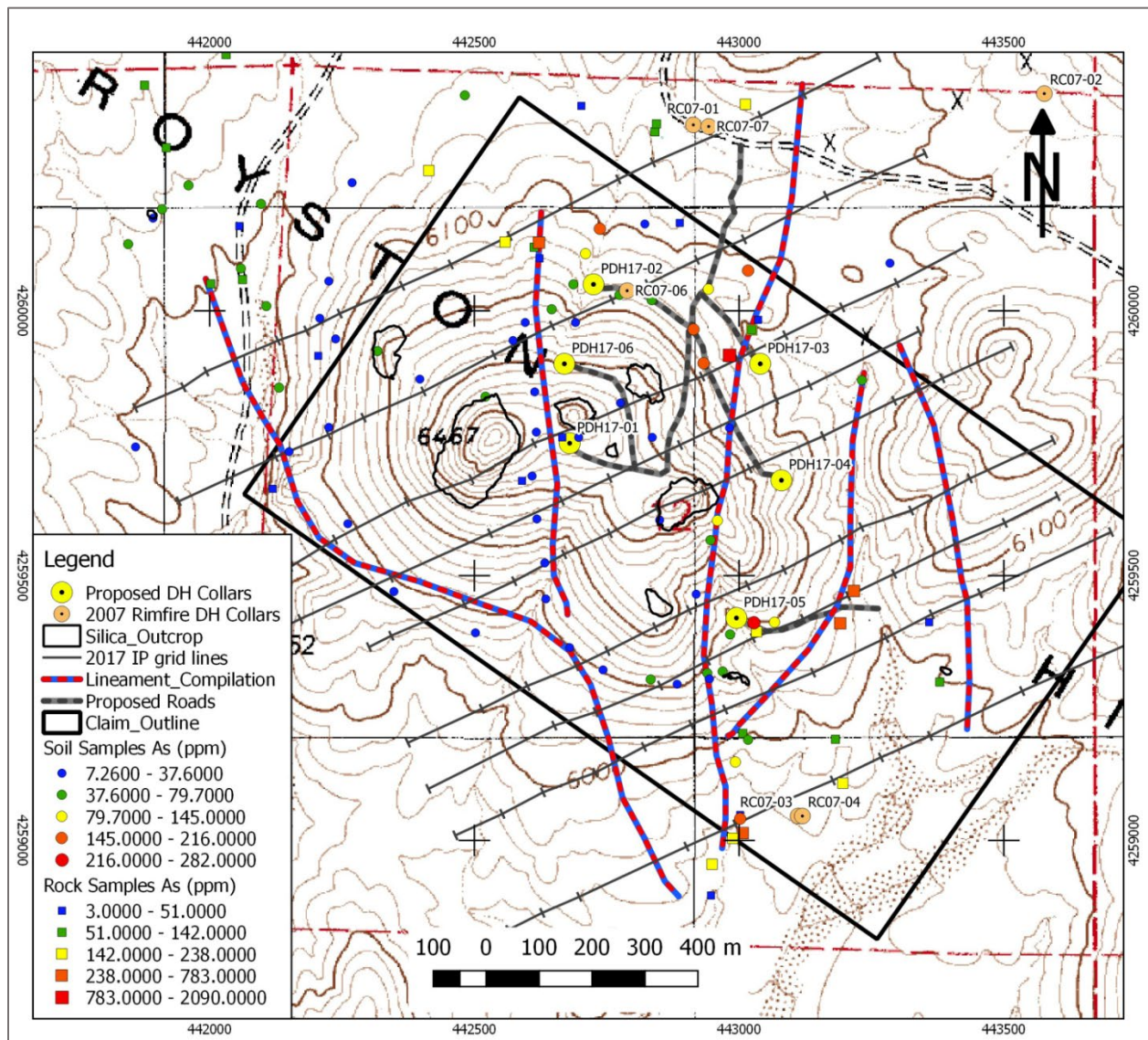
Figure 13: Arsenic geochem, silica caps, interpreted lineaments, and proposed drillholes
