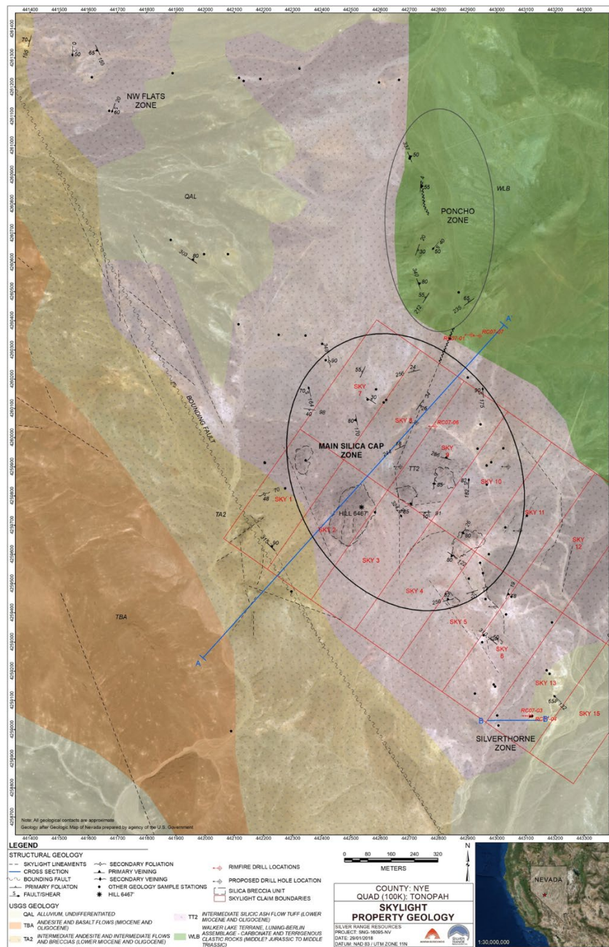
Figure 7: Skylight property geology
