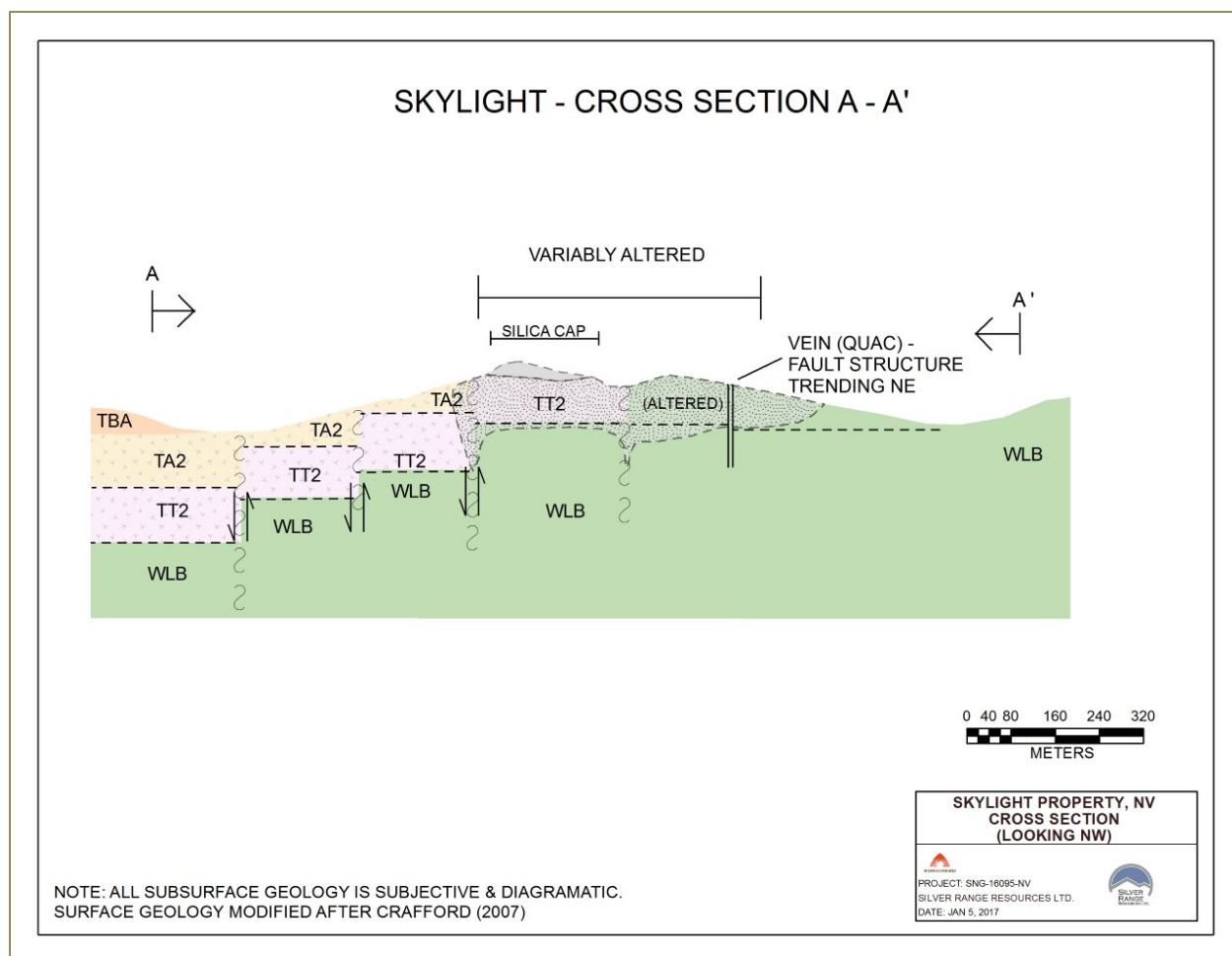
Figure 8: Conceptual cross-section A-A'
