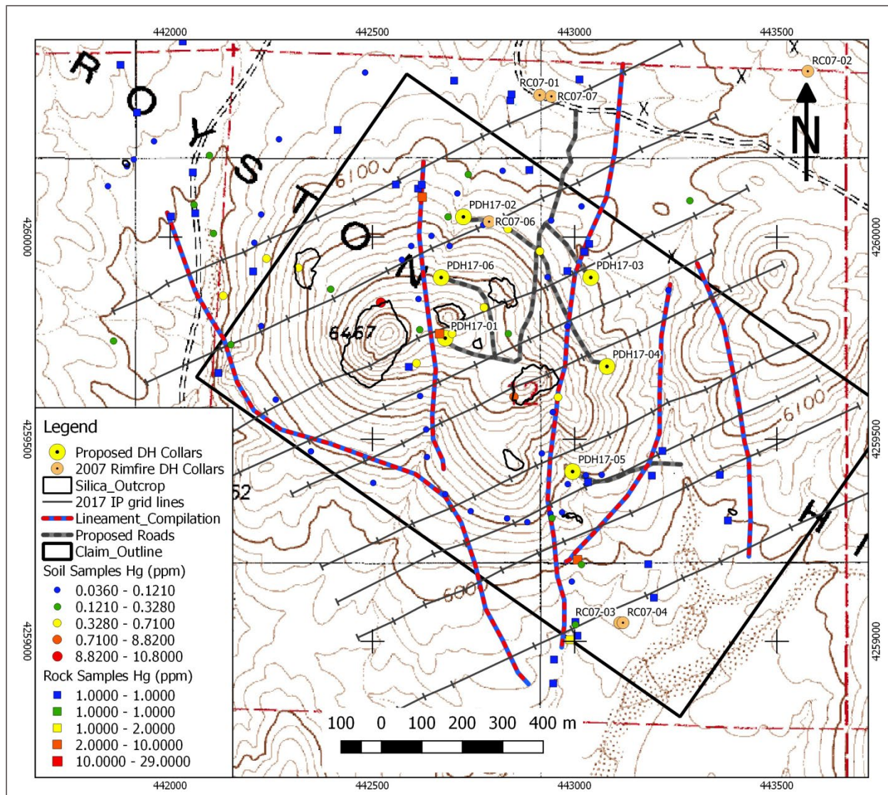
Figure 14: Mercury geochem, silica caps and interpreted lineaments, and proposed drillholes
