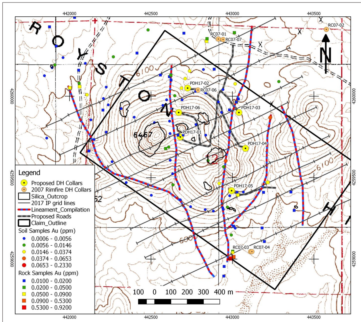
Figure 11: Gold geochem, silica caps, interpreted lineaments, and proposed drillholes
