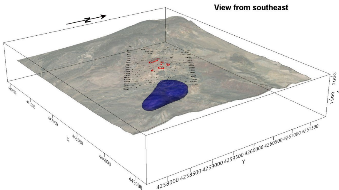
Figure 11: 3D resistivity model
