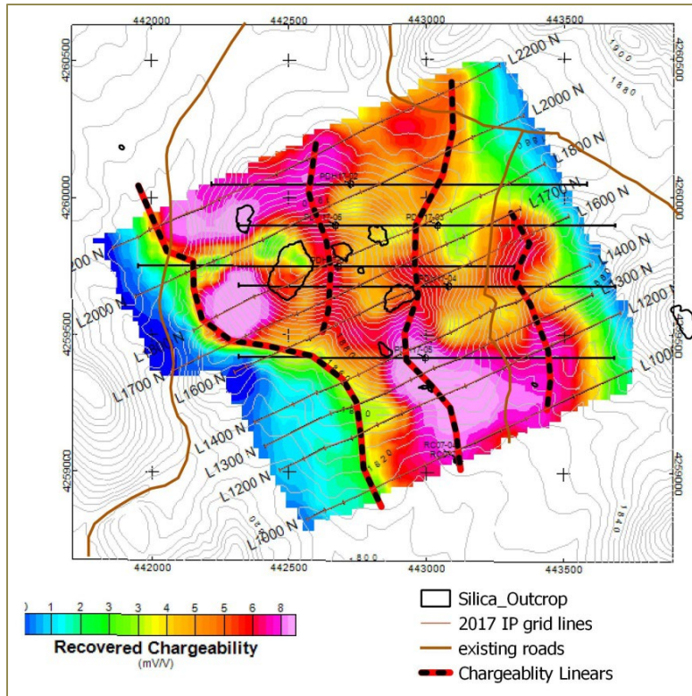
Figure 20. Inverted chargeability, draped at -100 m
