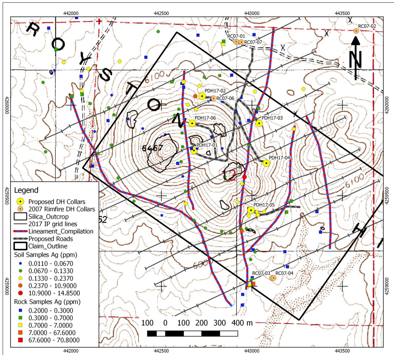
Figure 12: Silver geochem, silica caps, interpreted lineaments, and proposed drillholes
