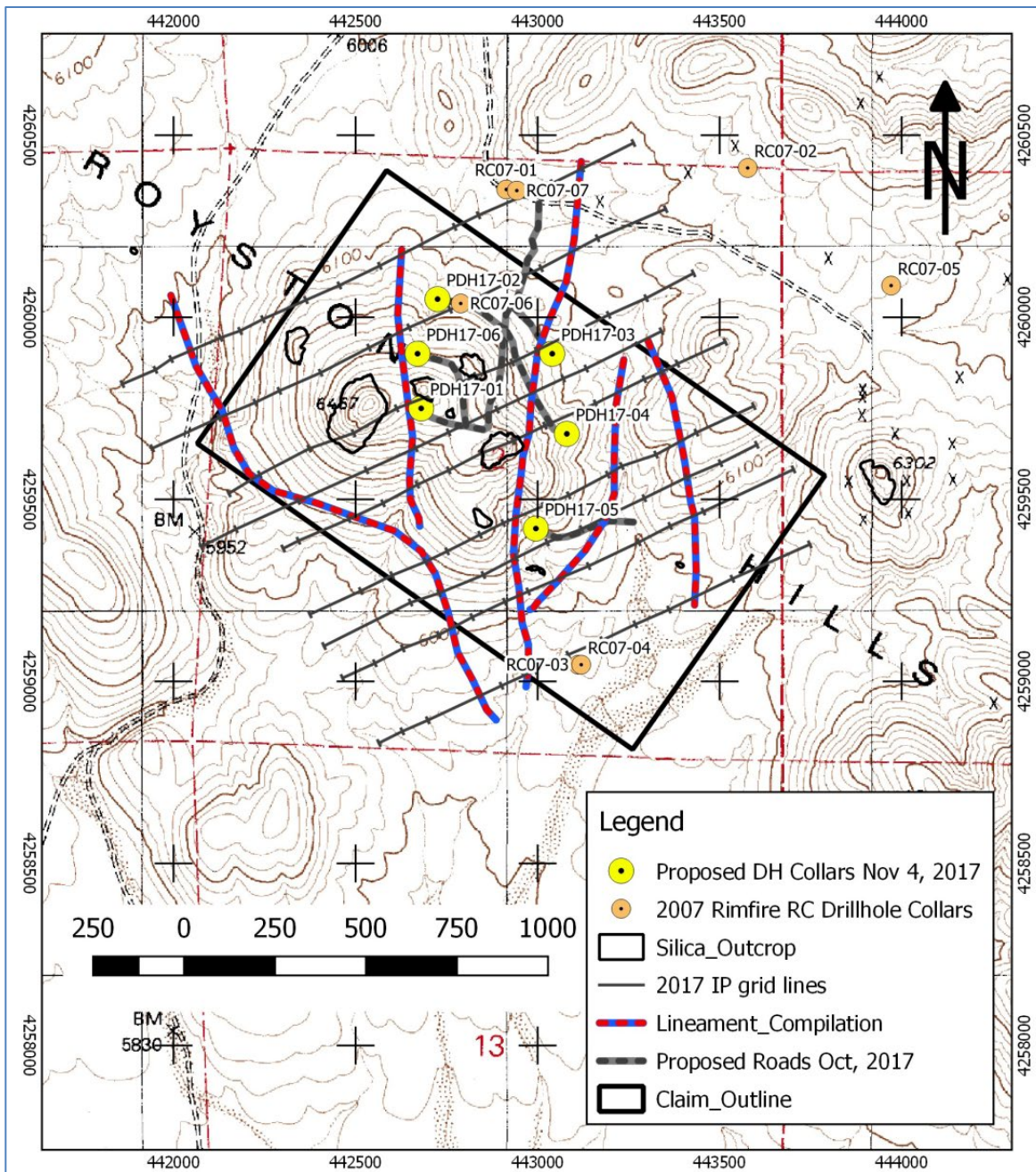
Figure 19: 2017 IP Grid location map
