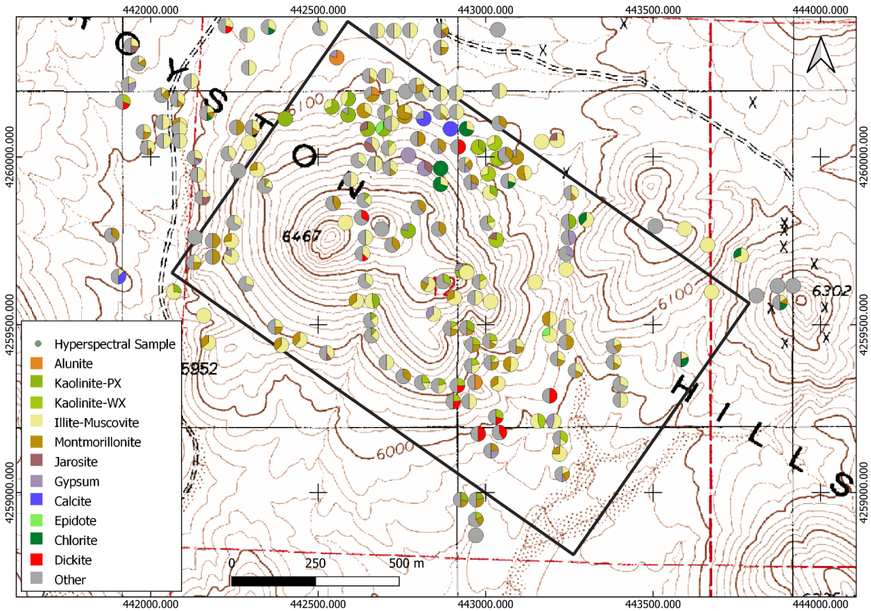
Figure 16: Hyperspectral mineral analysis
