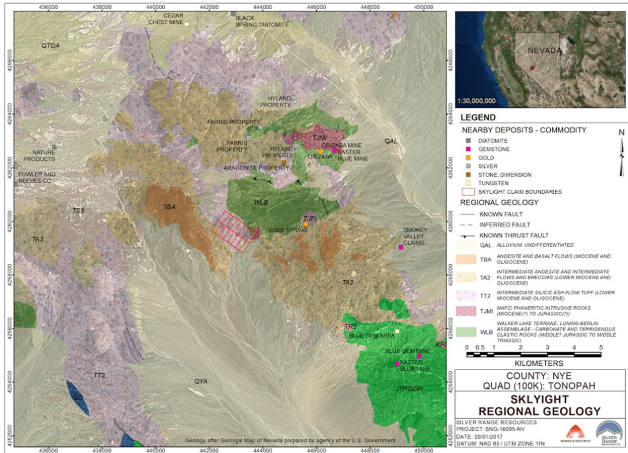
Figure 3: Skylight property – regional geology
