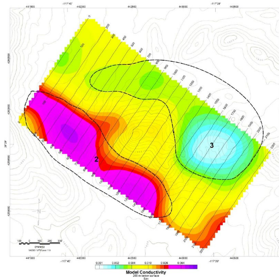
Figure 17: Conductivity model slice at 200 m below surface
