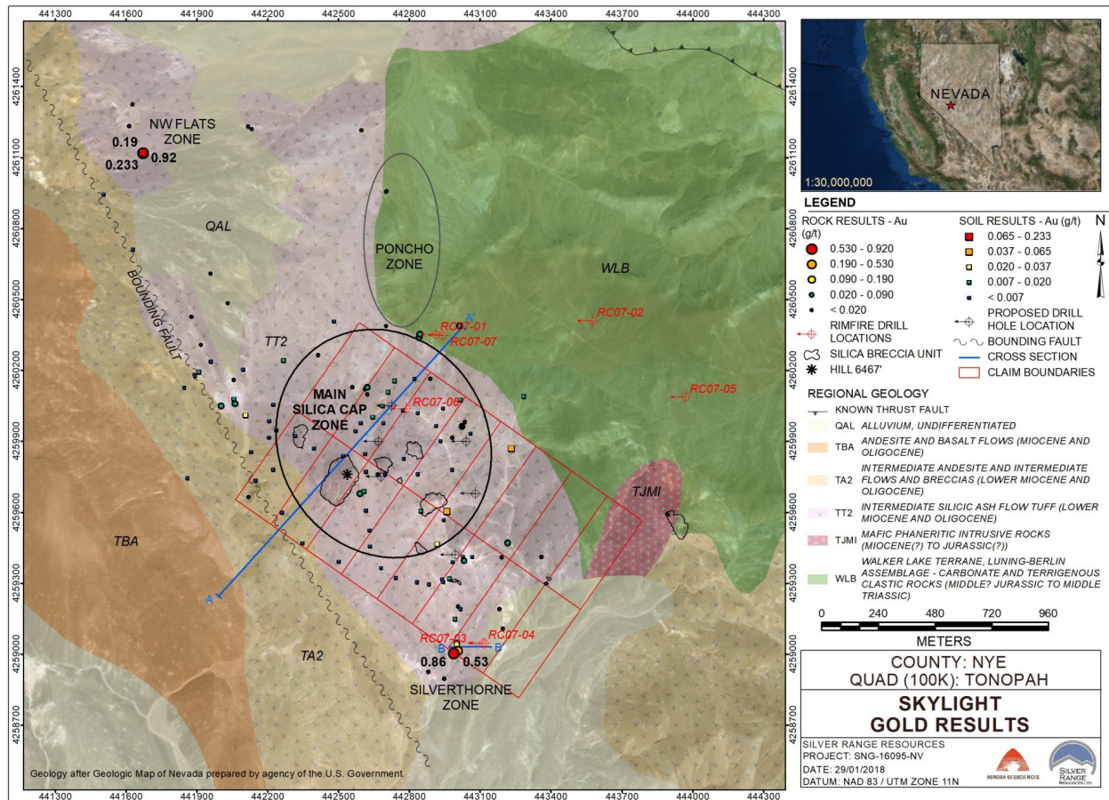
Figure 15: Compilation geology and Silver Range 2016 gold geochemistry
