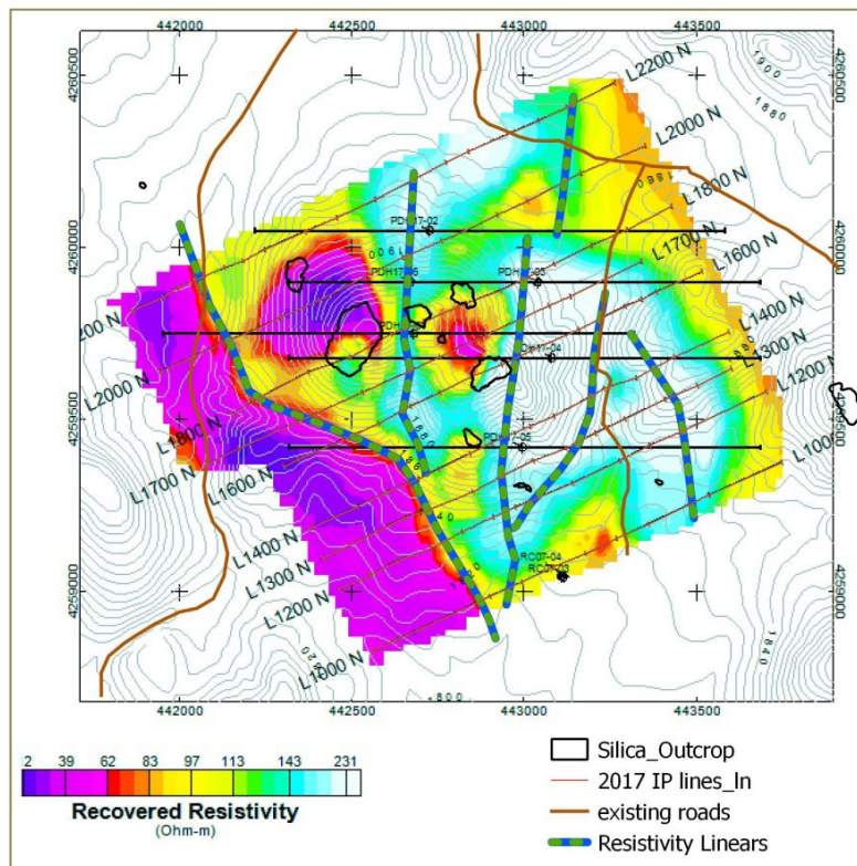
Figure 21. IP resistivity, draped at -100 m
