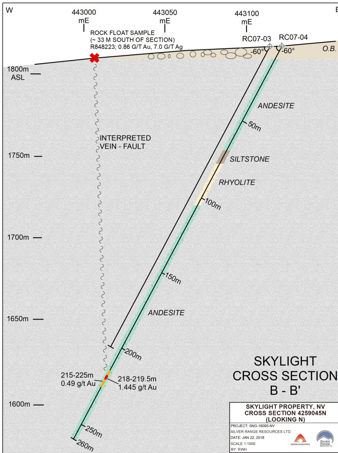
Figure 9: Silverthorne Zone – Cross-section B-B' and reverse circulation hole RC07-04
