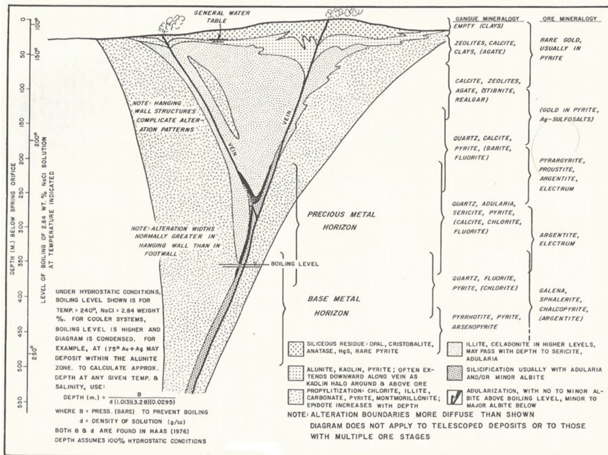
Figure 10: Buchanan epithermal deposit model (modified after Buchanan, 1981)
