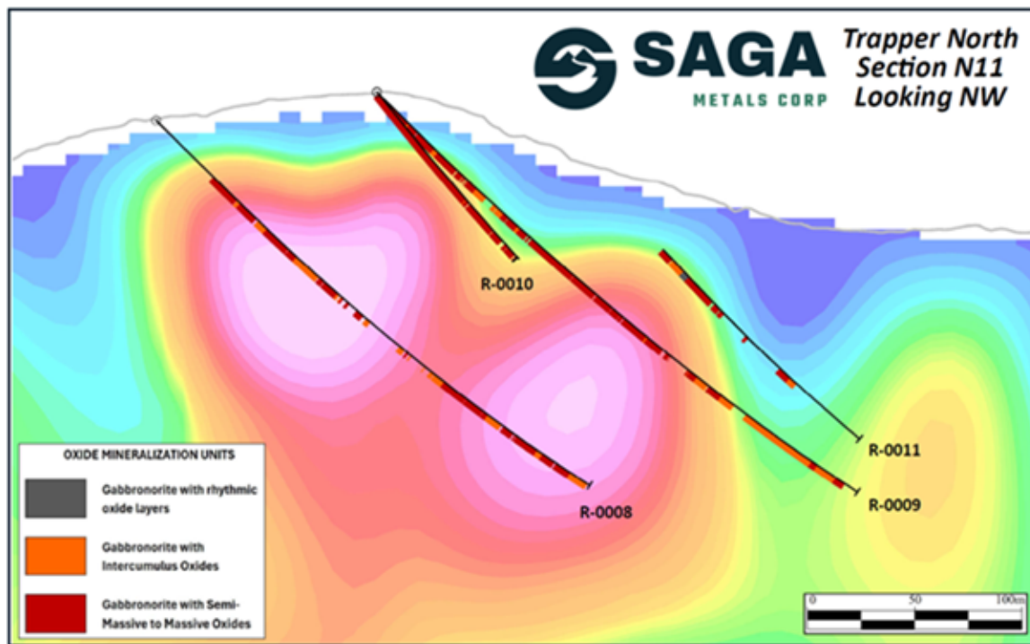
Figure 4: Cross-Section N-11 showing R-0008, -0009, -0010 and -0011 with the 3D Magnetic Inversion of the 2025 Trapper Zone ground magnetic survey.
