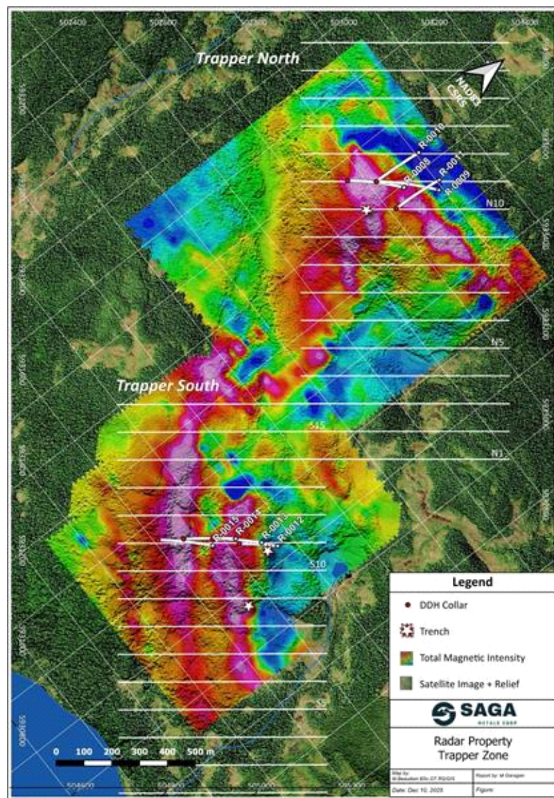
Figure 1: Location of the Phase 1 and Phase 2 of Fall 2025 Drilling at Trapper Zone, showing the TMI of the 2025 Trapper Zone ground magnetic survey.
