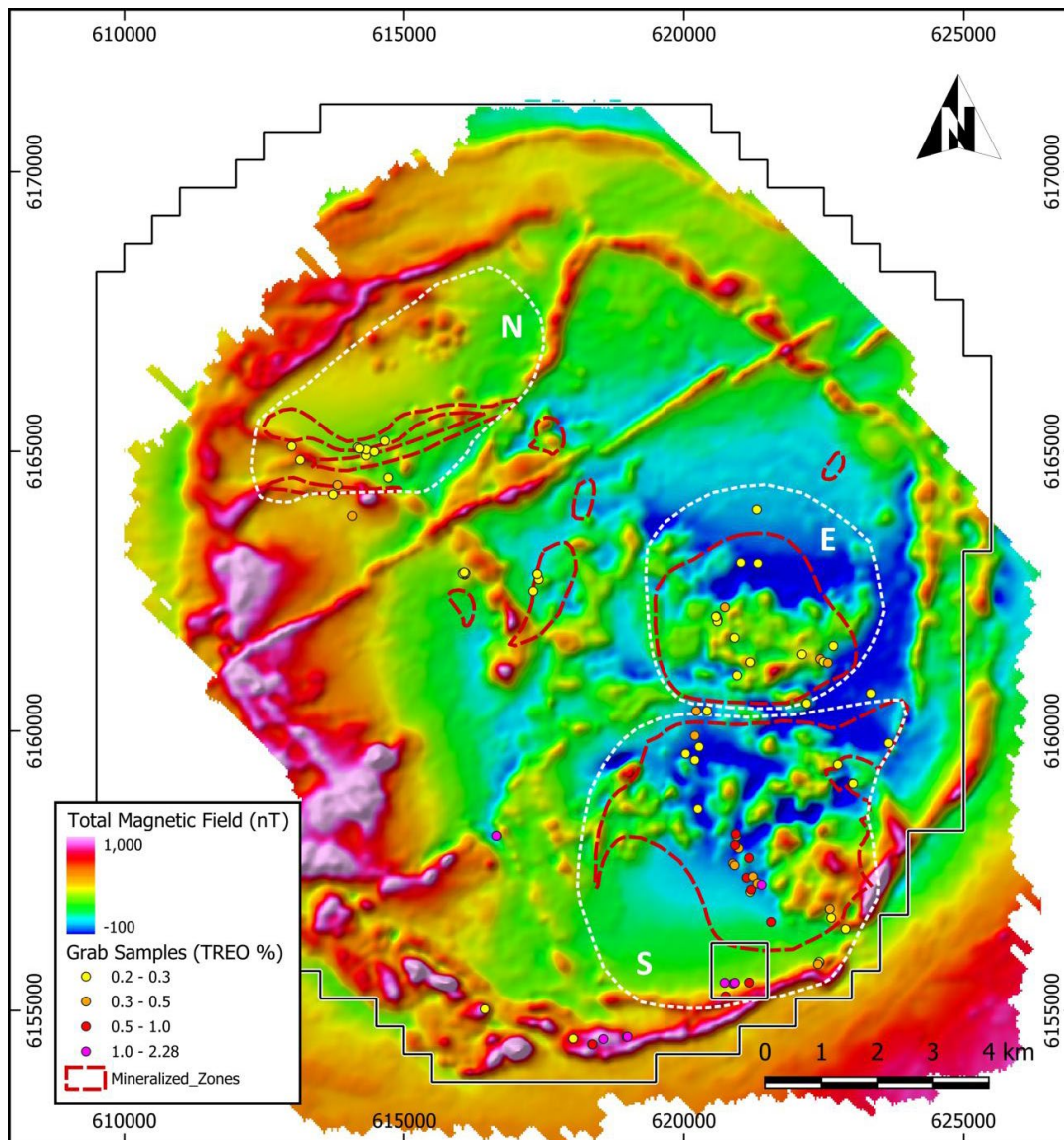
Figure 6: Total magnetic field map of the Nuiklavik Caldera Complex. Grab samples with TREO \geq 0.2\% are shown as scaled symbols. The volcanic pile is preserved within nested calderas in the central portion of FRIS.
