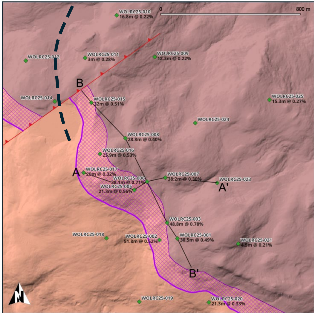
Figure 3: Drillholes are plotted on LiDAR-derived elevation model hillshade with the geologic map colors for Units 4 and 5. The enriched outcrop zone, possible normal fault trace, and cross sections (A-A' and B-B') are indicated. See Figure 2 for the broader geological context.
