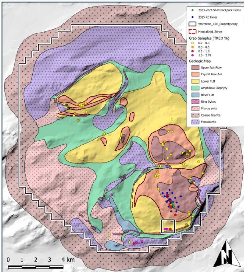
Figure 2: Local geologic map of the Nuiklavik Caldera Complex.
