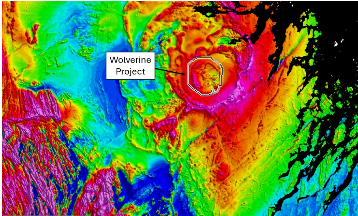
Figure 5: Total field aeromagnetic map of the Flowers River area. The FRIS is expressed as a prominent circular magnetic high within the surrounding Nain Plutonic Suite.
