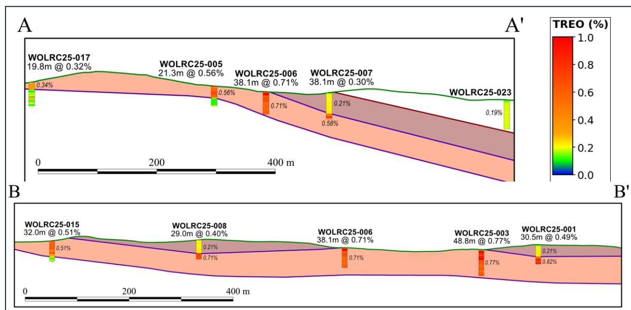
Figure 4: Cross sections A-A' and B-B' as outlined above in Figure 3 showcasing the shallow dipping stratigraphy from surface.
