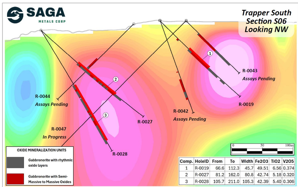
Figure 3: Cross section of S6 looking NW showing R-0019, -0027, -0028, -0042, -0043, -0044, and -0047 highlighting intercepts of semi-massive oxides and layering sequence with the 3D Magnetic Inversion of the 2025 Trapper Zone ground magnetic survey. Assays shown for R-0019, -0027, and -0028 with pending assays for R-0042, R-0043, R-0044, and R-0047.
