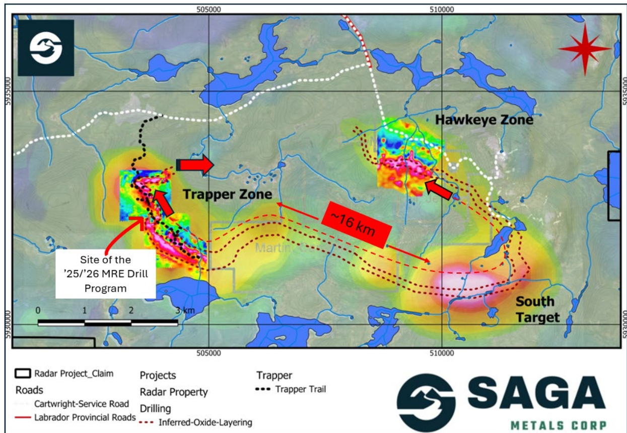
Figure 5: Radar Project's prospective oxide layering zone validated over about 16 km strike length through Fall 2025 drilling, as shown on a compilation of historical airborne geophysics as well as ground-based geophysics in the Hawkeye and Trapper zones completed by SAGA in the 2024/2025 field programs. SAGA has demonstrated the reliability of the regional airborne magnetic surveys after ground-truthing and drilling in the 2024 and 2025 field programs.
