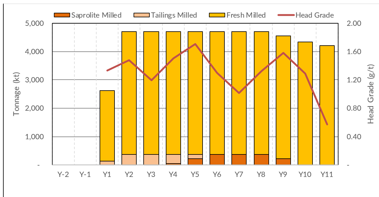
Figure 1.2: Annual Mill Production
