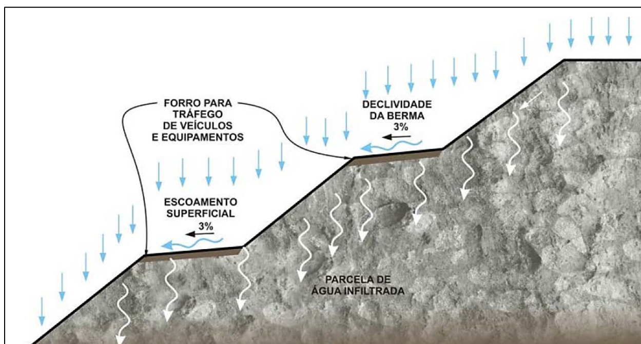
Figure 16.7: Inclined Berms
