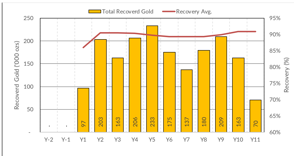
Figure 16.24: Gold Production
