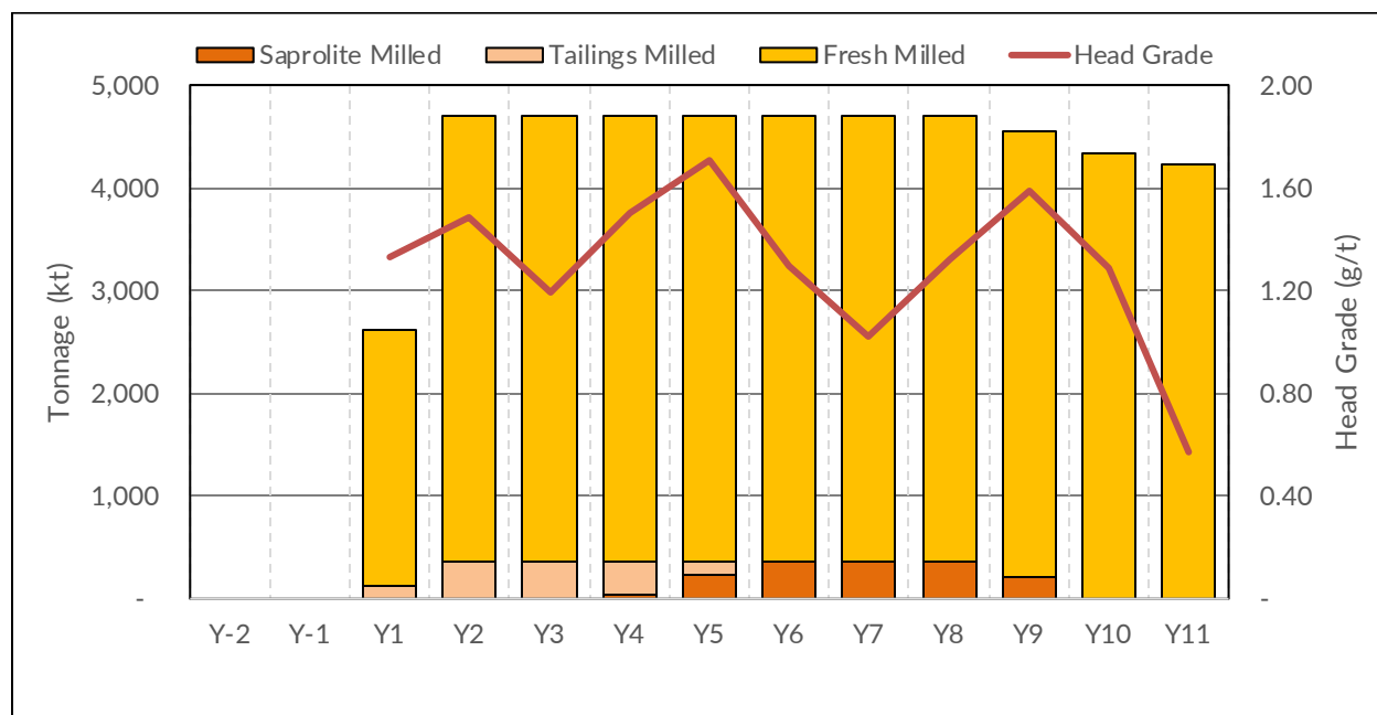
Figure 16.21: Mill Feed by Rock Type
