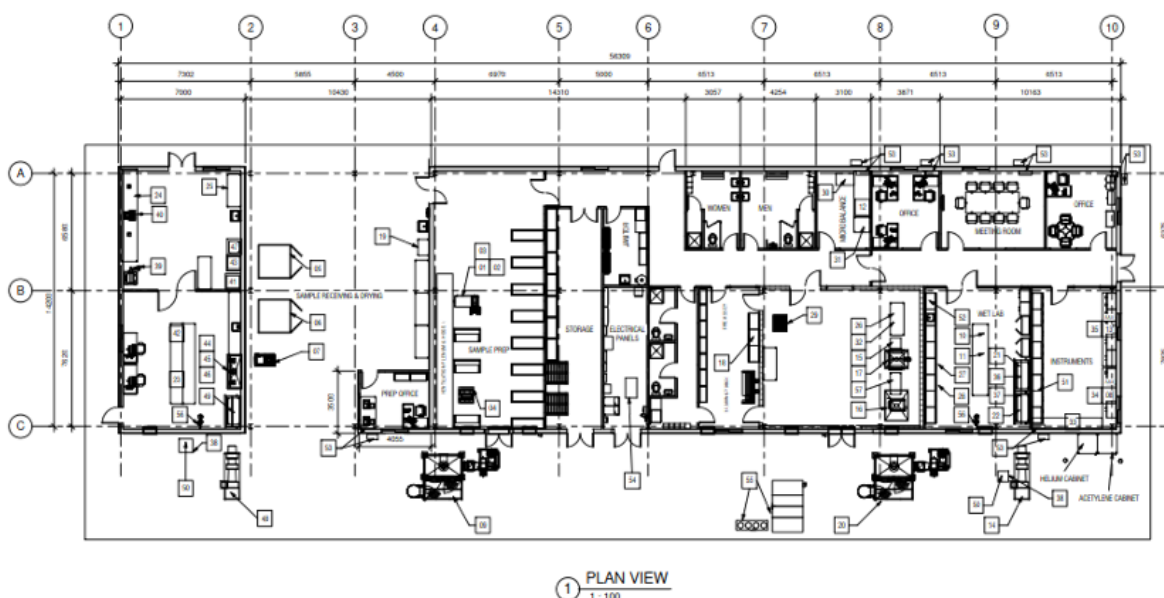
Figure 18.8: Assay Laboratory
