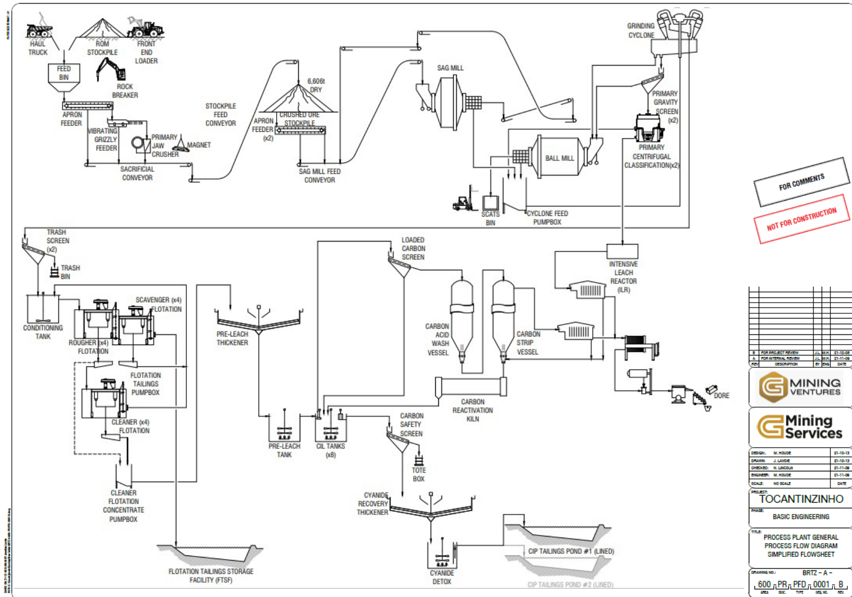
Figure 17.1: Overall Flowsheet
