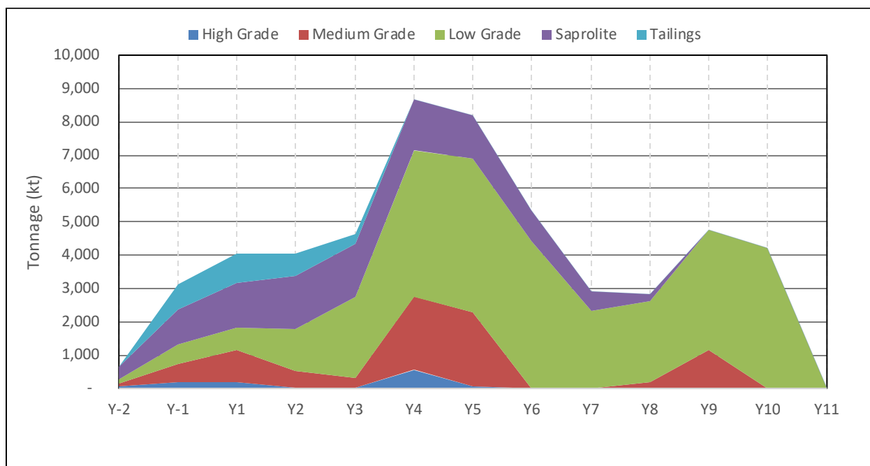
Figure 16.23: Stockpile Inventories
