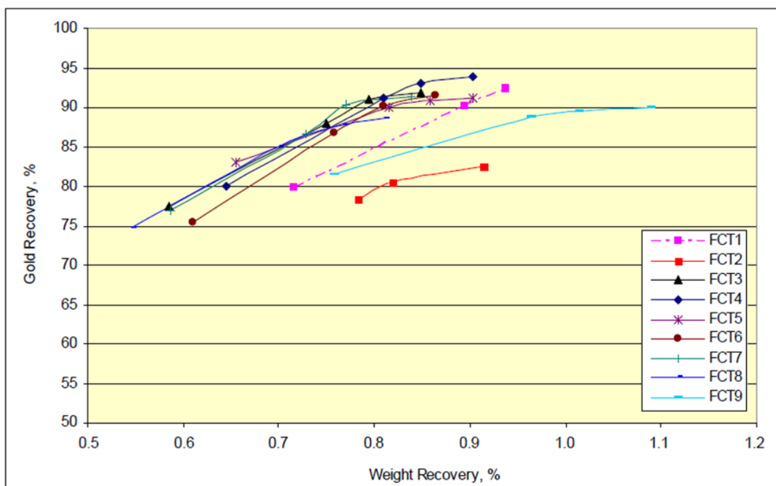
Figure 13.7: Gold Recovery vs Concentrate Mass Pull for Cleaner Flotation Test Work
