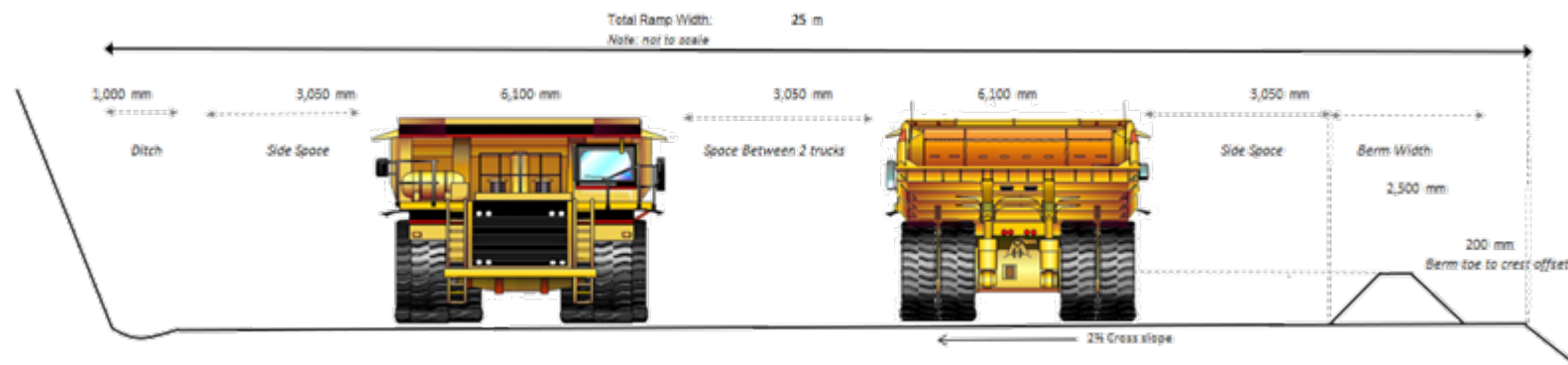
Figure 15.7: Double-Lane Ramp Design Criteria
