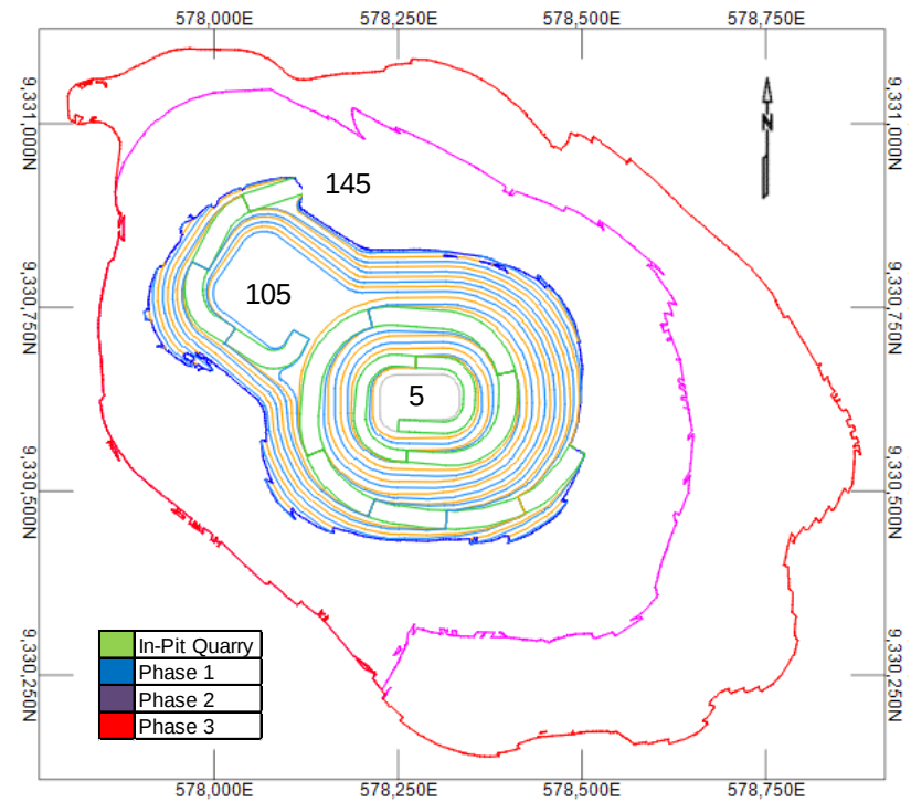
Figure 16.3: Phase 1 Design
