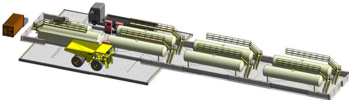
Figure 18.7: Fuel Storage
