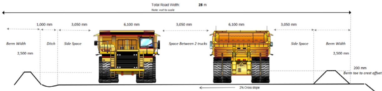
Figure 16.11: Ex-Pit Haul Road Design Criteria
