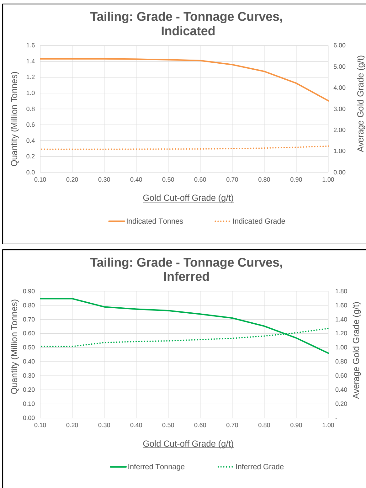
Figure 14.20: Global Grade Tonnage Curves for Tailings (Indicated, above and Inferred below)
