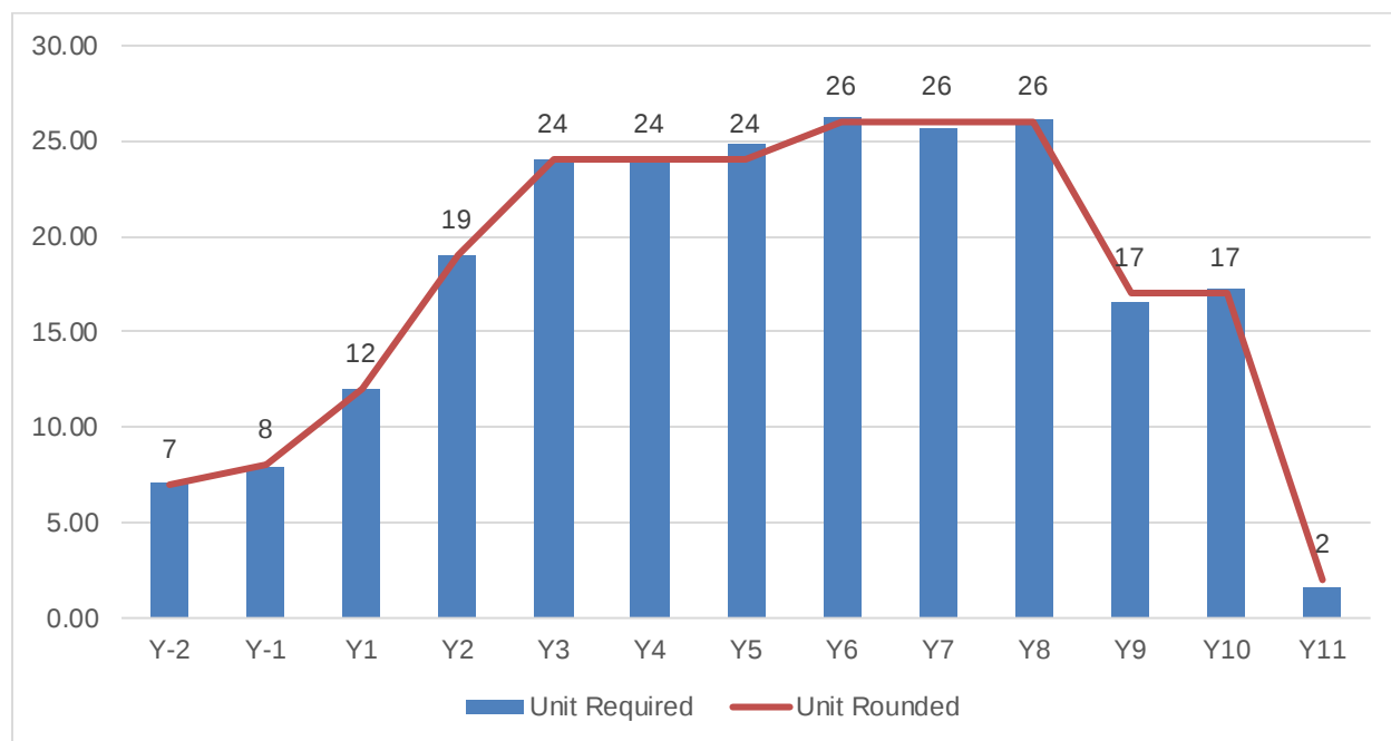
Figure 16.27: Truck Requirements
