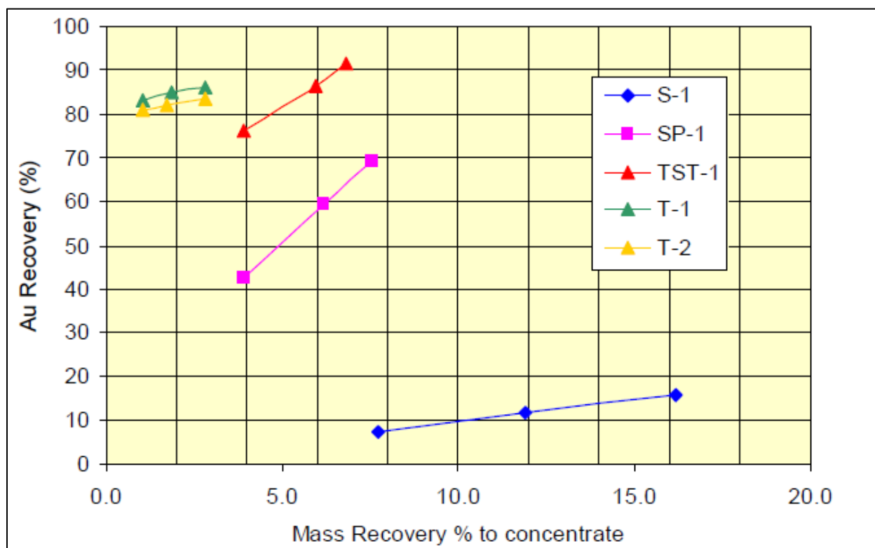
Figure 13.9: Gold Flotation Recovery Results of Saprolite and Tailings Samples
