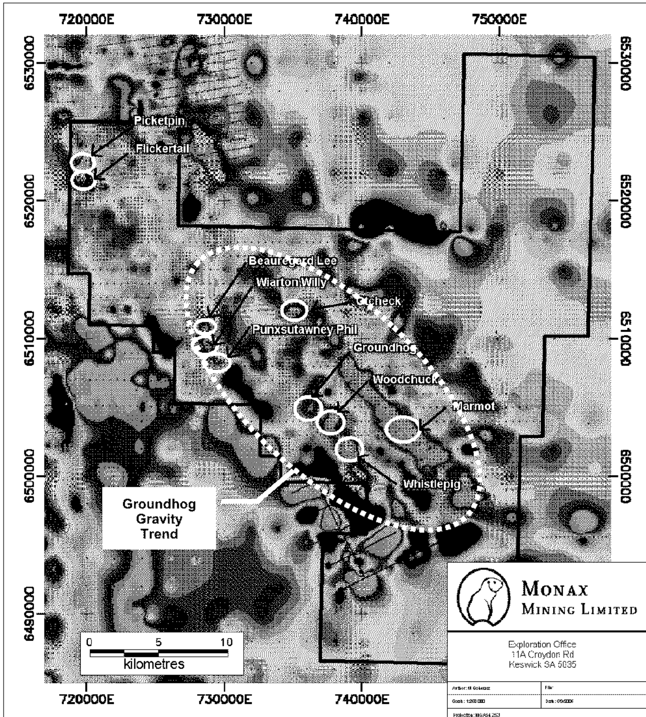
Figure 2. Punt Hill iron oxide copper-uranium-gold targets on residual gravity image
