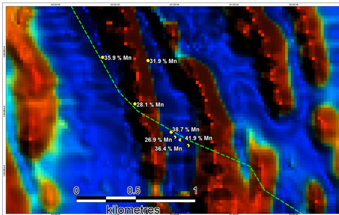
Figure 2. Pollinga Prospect, sample locations on residual magnetics (Mn %)
