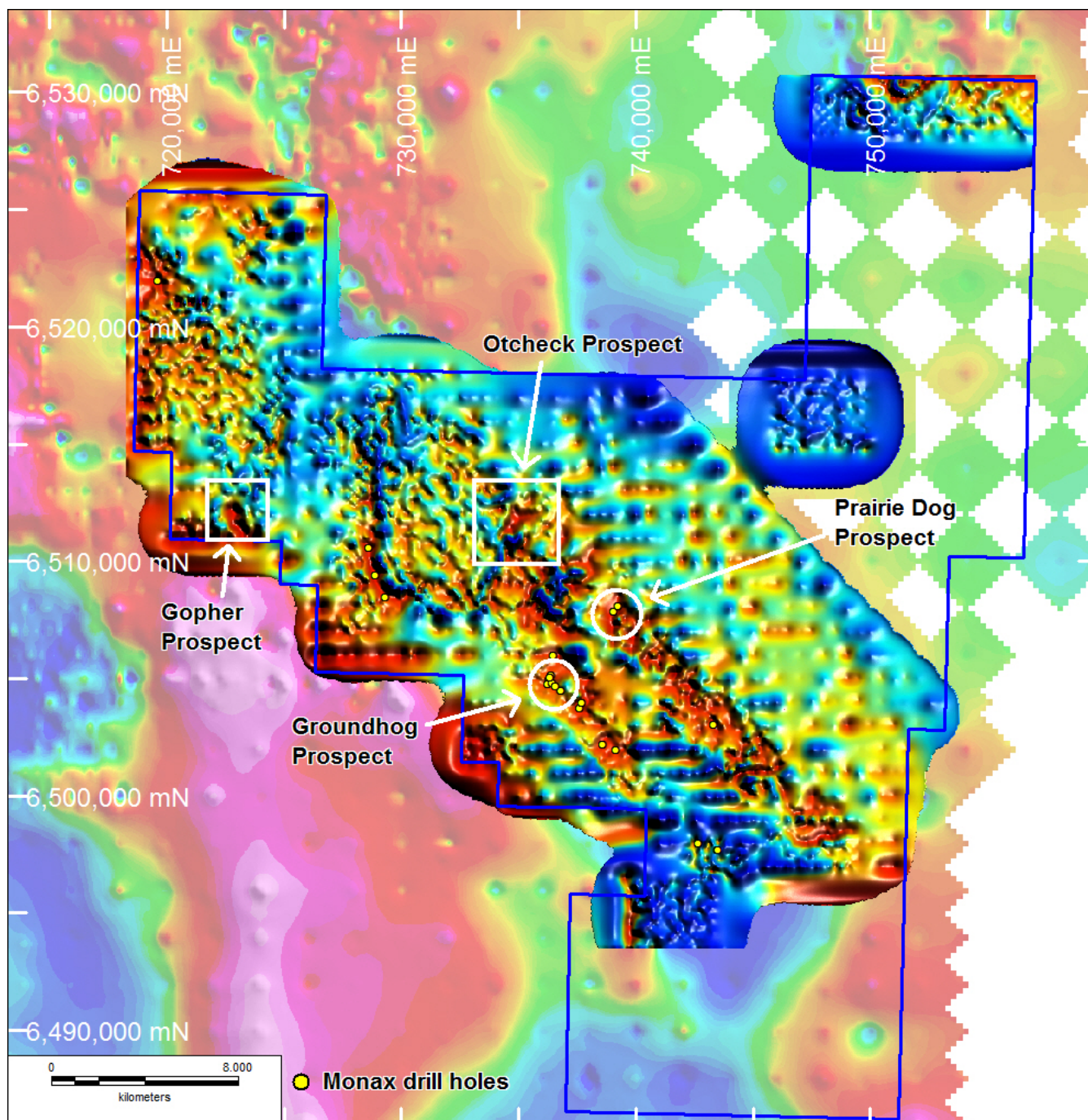
Figure 3: New infill gravity data combined with previously collected data showing two new gravity anomalies at Gopher and Otcheck
