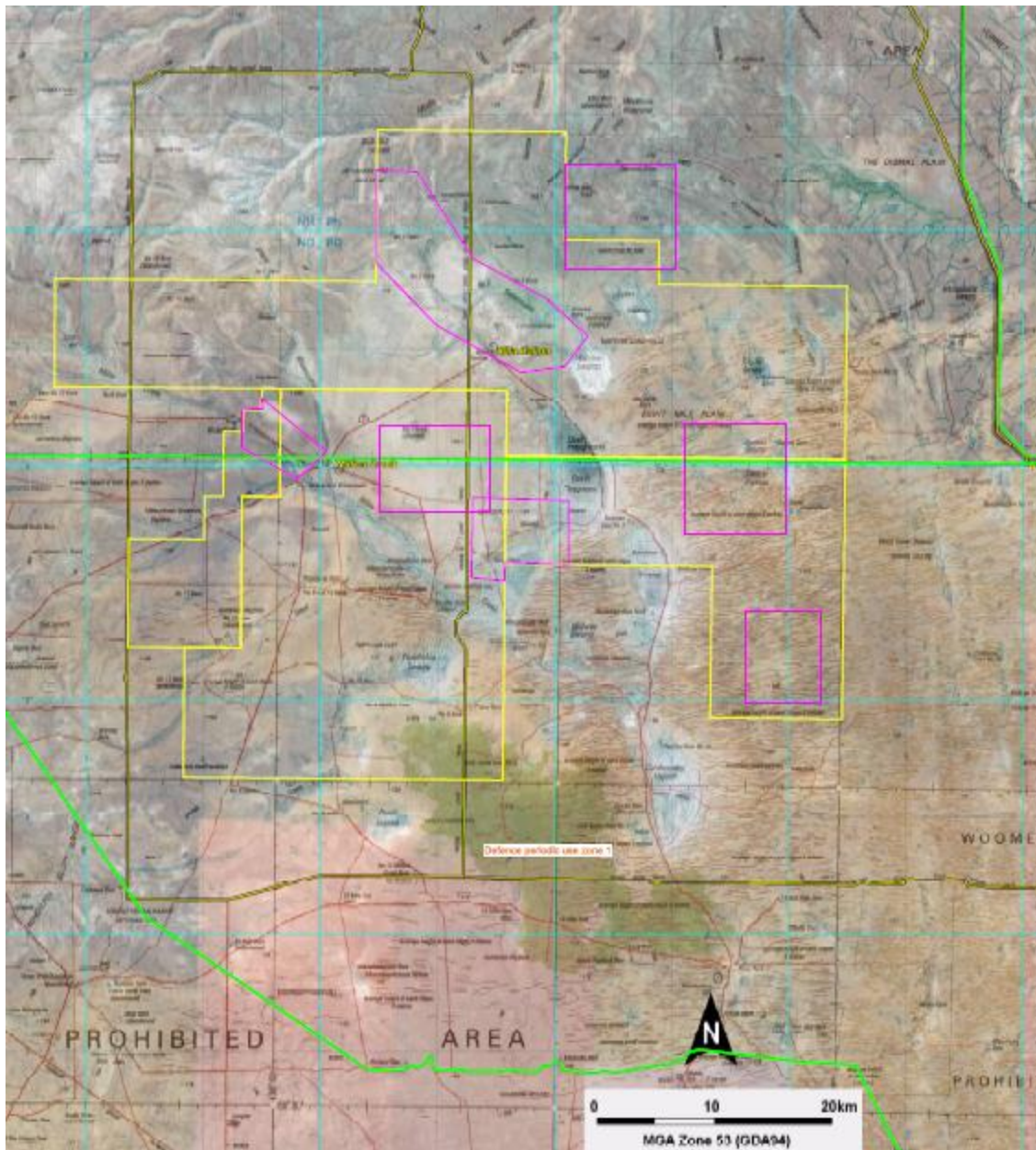
Figure 1. Gravity targets (purple shapes) within the Billa Kalina tenements.
