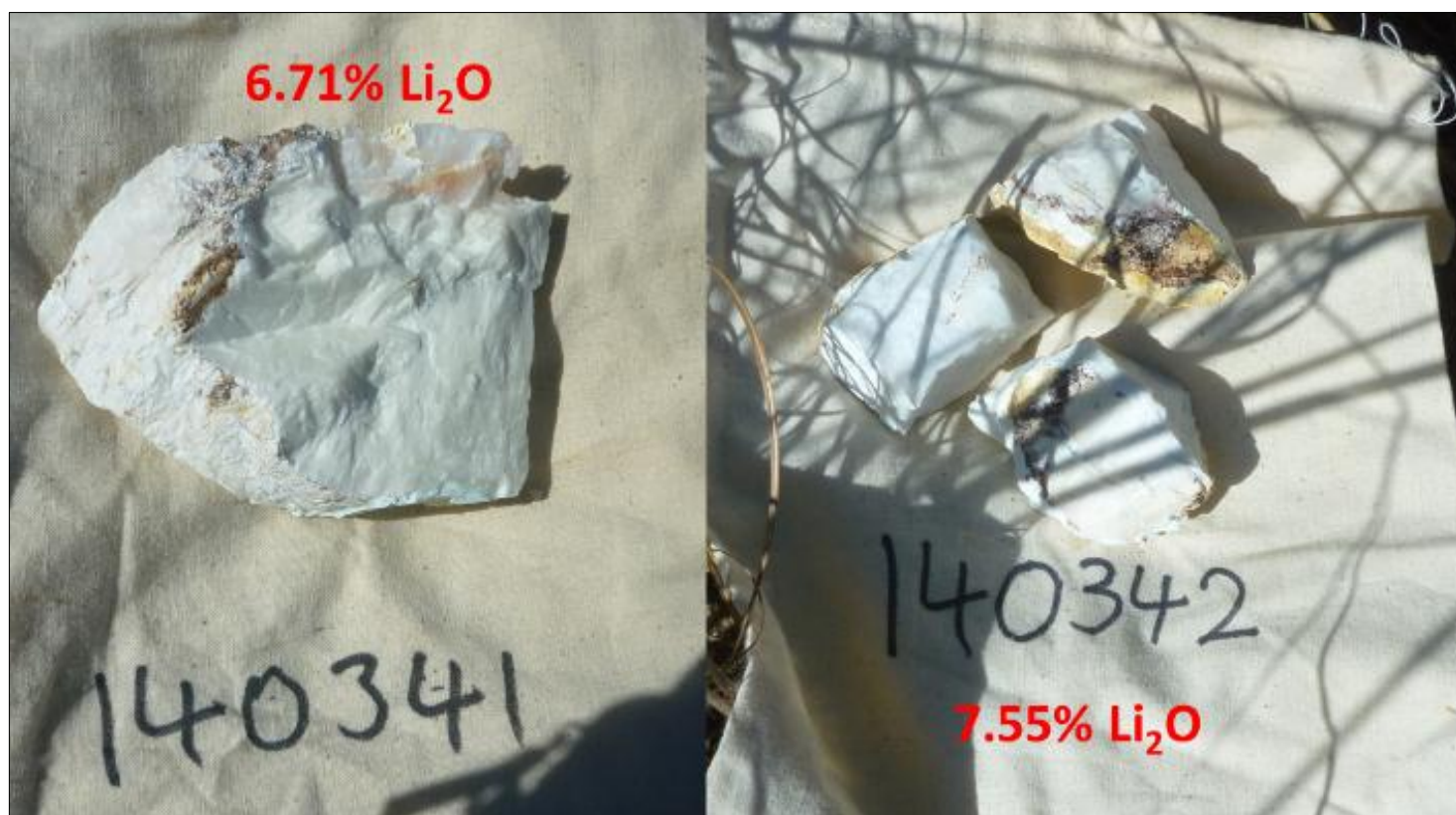
Plate 1: High-grade amblygonite samples from Litchfield Project.
