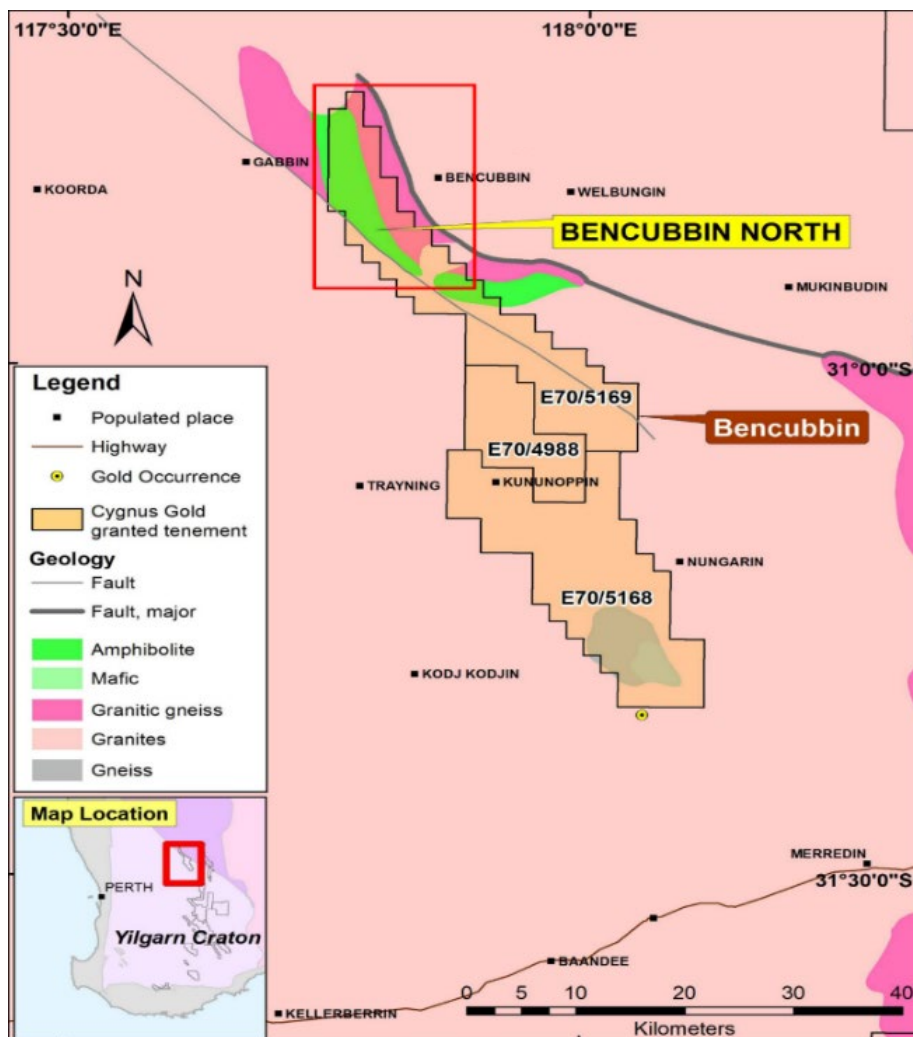
Figure 3: Cygnus' Bencubbin project on mapped regional geology (1:500,000 GSWA mapping)
