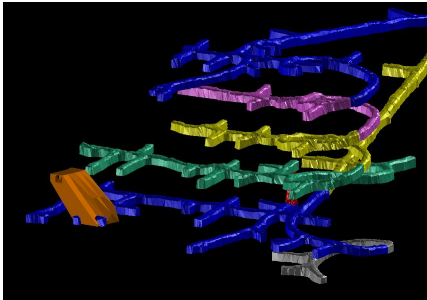
Level development and first stope location (855 level) at Roswell
