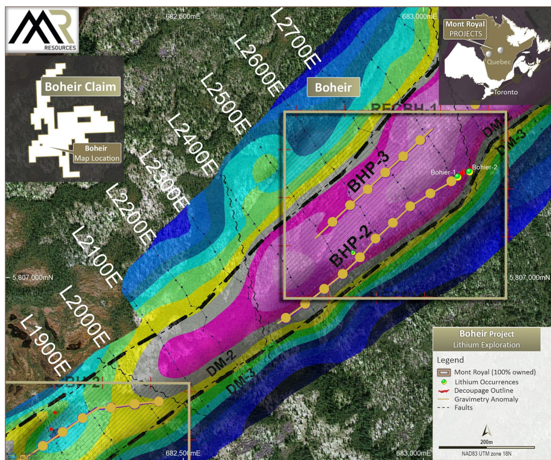
Figure 2 – Gravimetric survey results showing the 500m target zone and the three known pegmaties. Source: IOS Géoscientifique.
