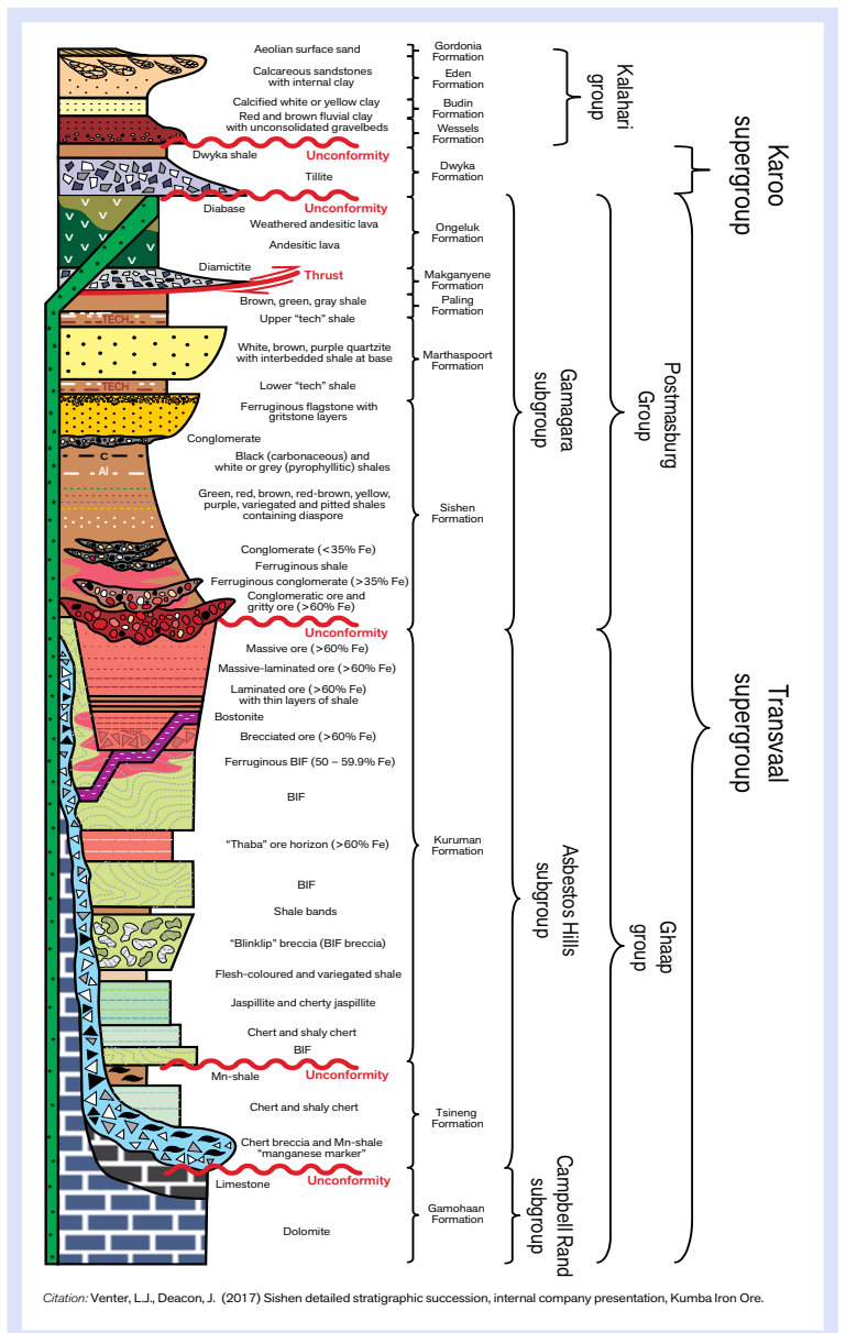
Figure 25: Simplified stratigraphic column depicting the Sishen local geology
