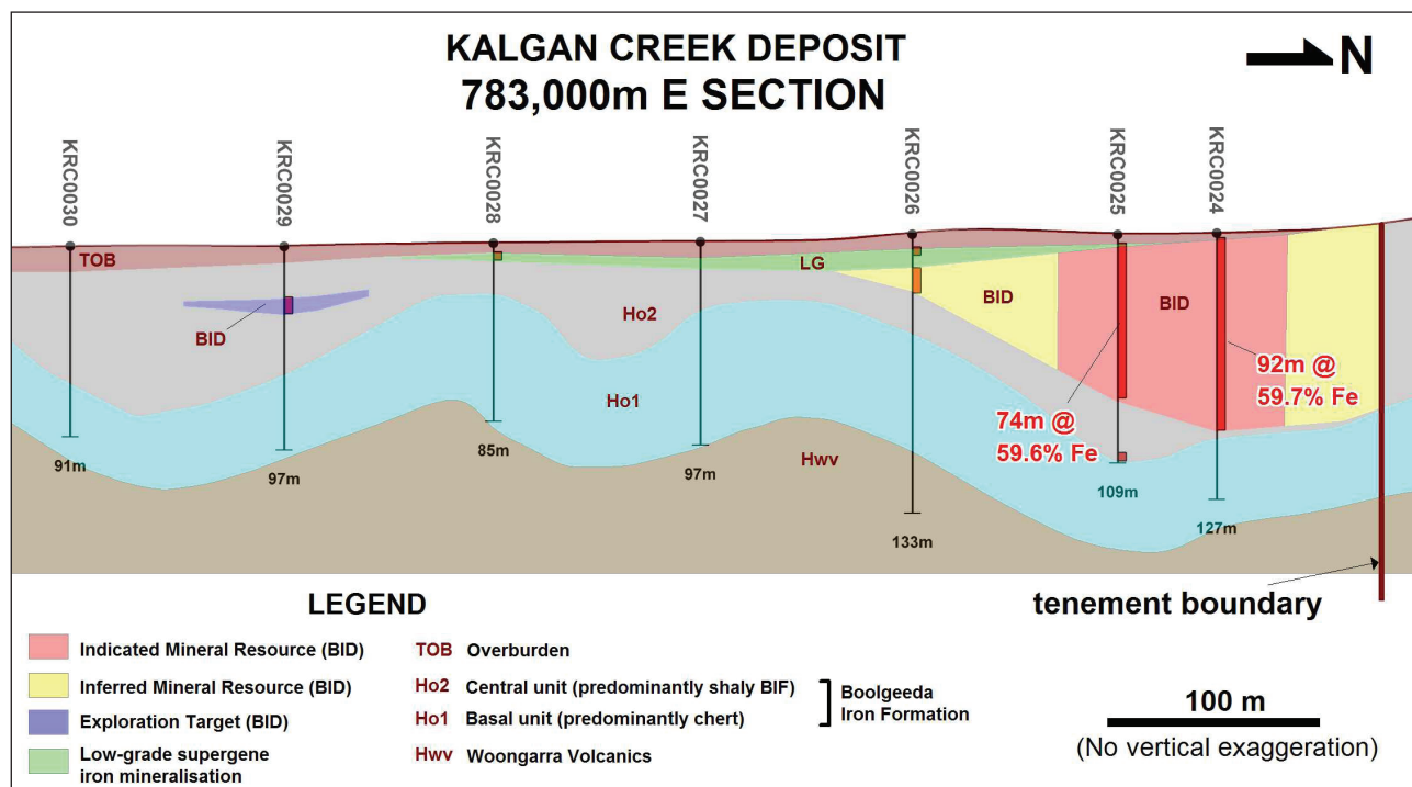
Figure 3: Kalgan Creek Deposit – cross-section at 783000m E
