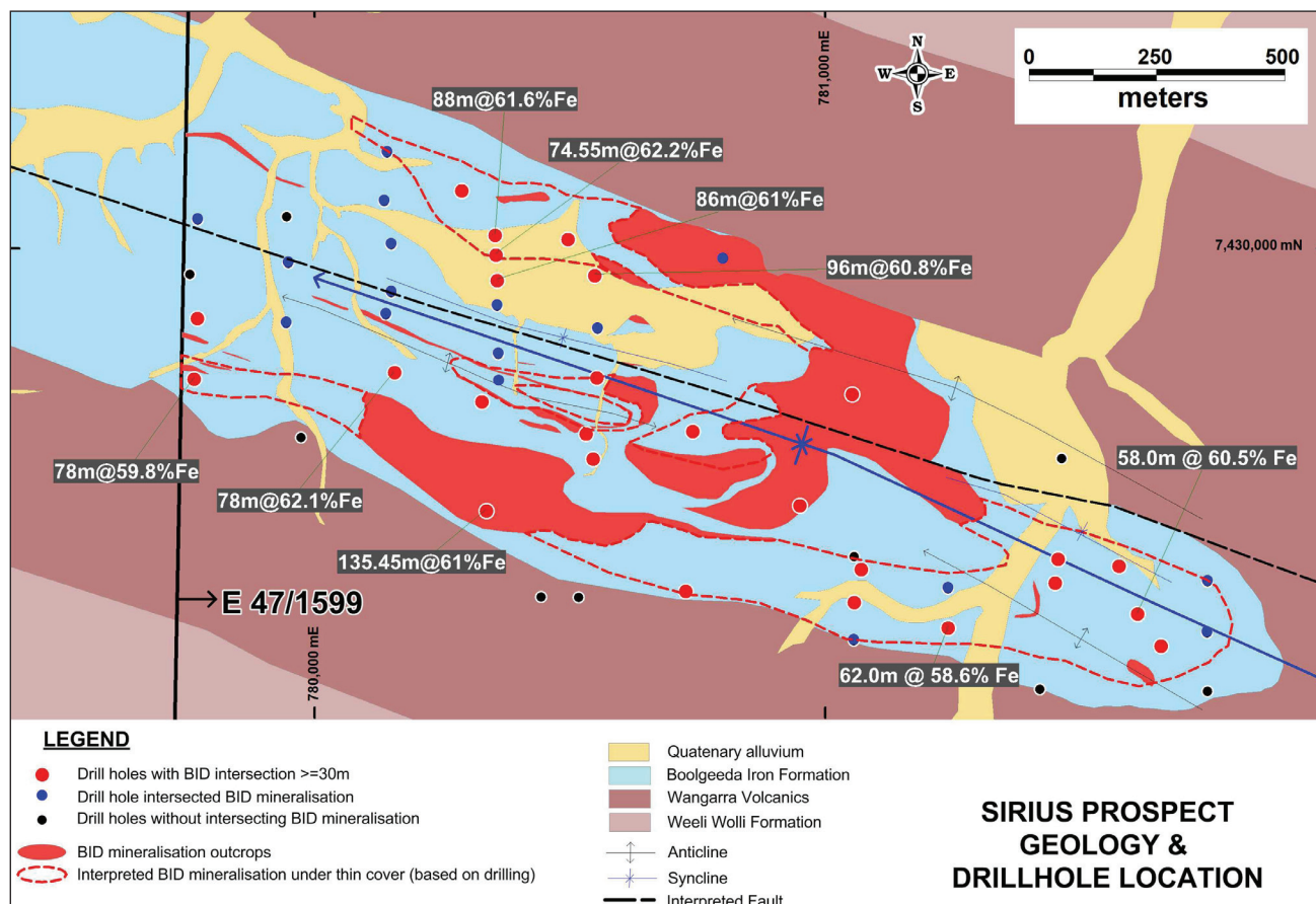
Figure 4: Geology and drill hole location of Sirius prospect
