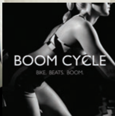
Boom Cycle
