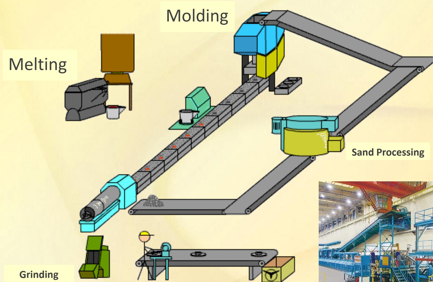
DISA Molding Line
