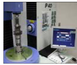
Klingelnberg 齒形機Gear Tester
