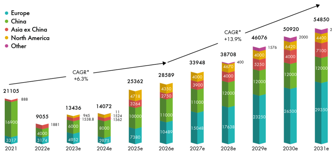
New offshore installations, global (MW)
